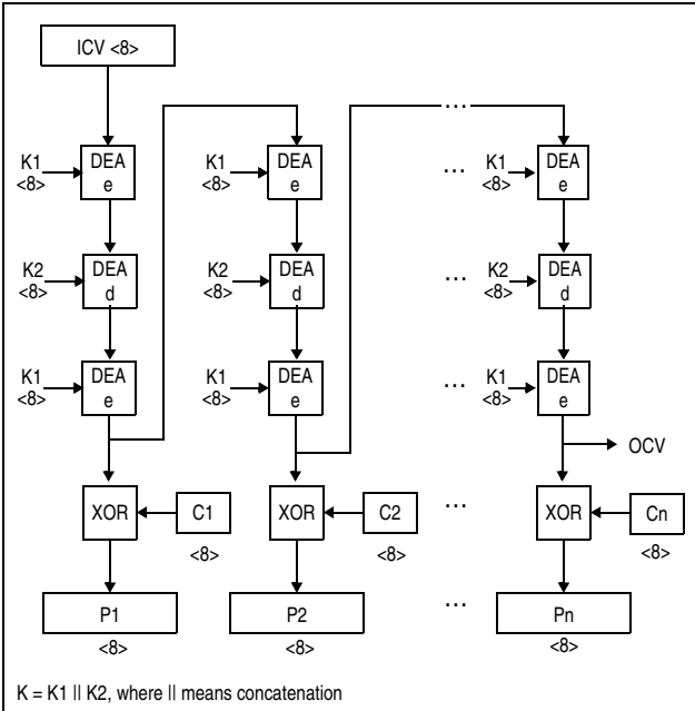
Figure 7-156. KMO-TDEA-128 Decipher Operation
