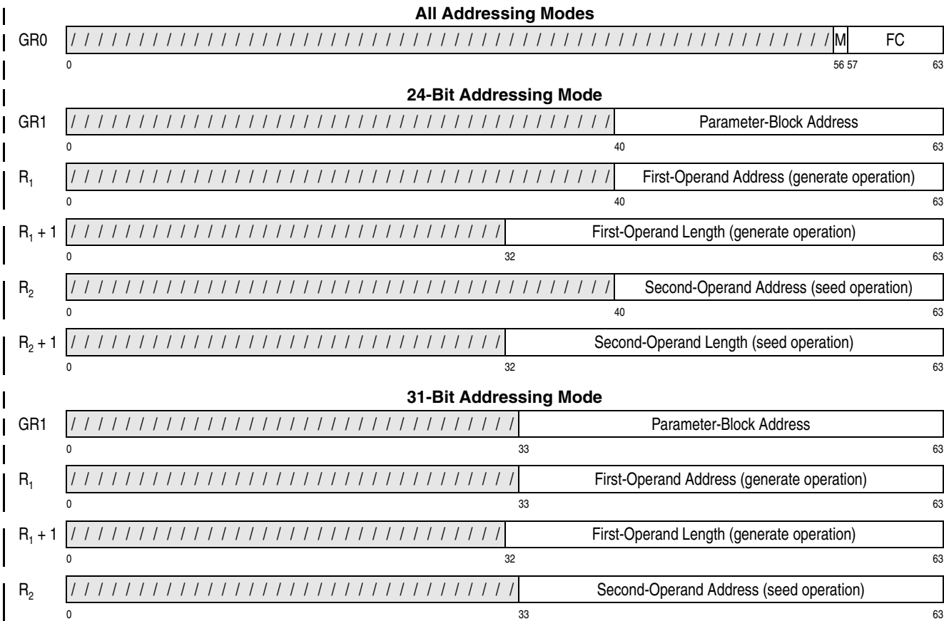
Figure 7-297. General Register Assignment for PPNO (Part 1 of 2)
