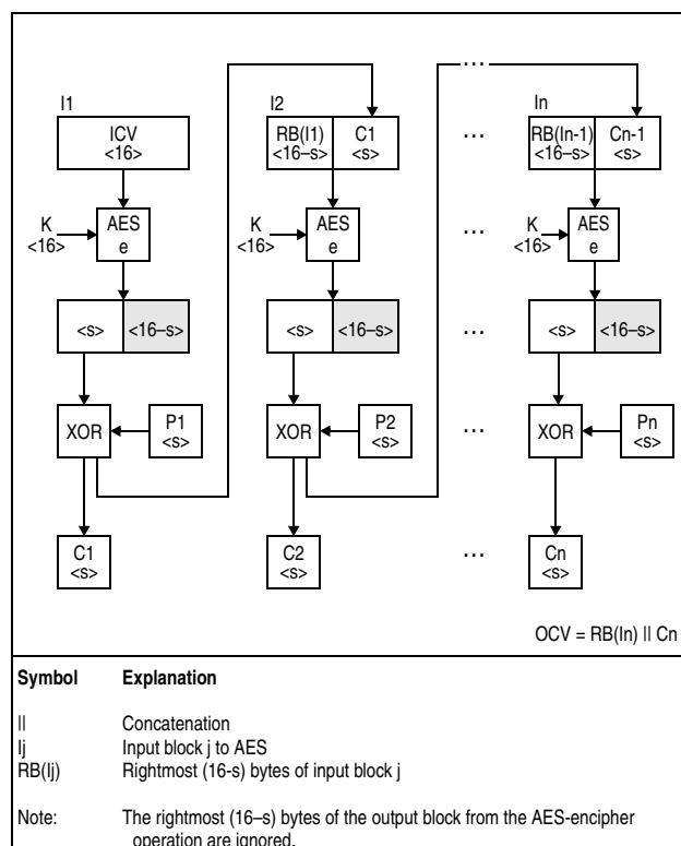
Figure 7-97. KMF-AES-128 Encipher Operation
