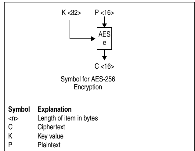
Figure 7-225. Symbols for AES-256 Encryption
