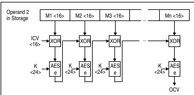
Figure 7-241. KMAC-AES-192
