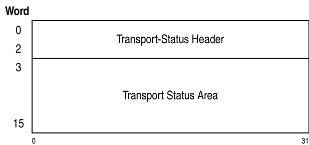
Figure 15-20. Transport-Status Block
