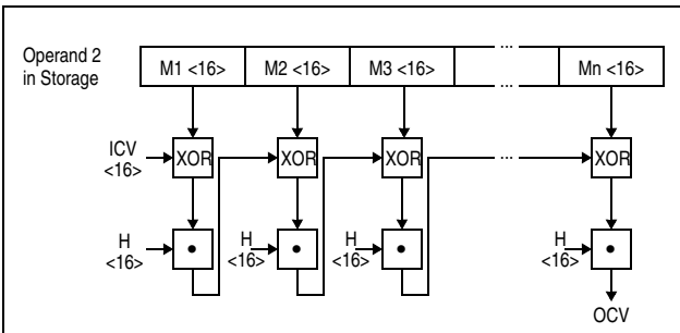
Figure 7-201. KIMD-GHASH
