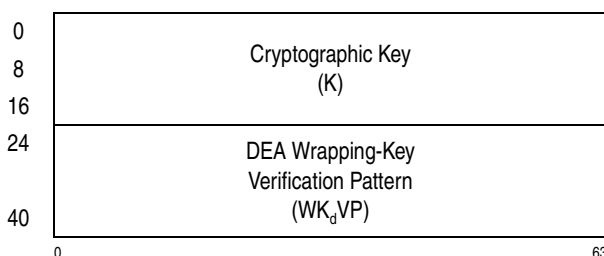
Figure 10-43. Parameter Block for PCKMO-Encrypt-TDEA-192-Key
