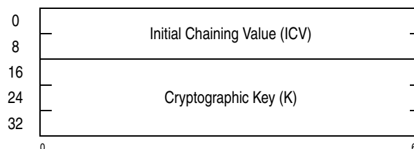
Figure 7-239. Parameter Block for KMAC-AES-192
