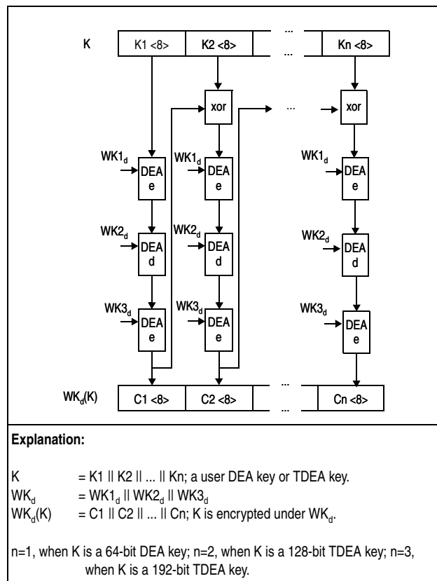
Figure 7-320. Encryption of DEA or TDEA Key Using WK d
