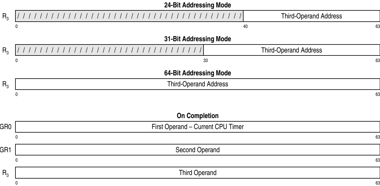
Figure 7-252. General Register Assignment for EXTRACT CPU TIME
