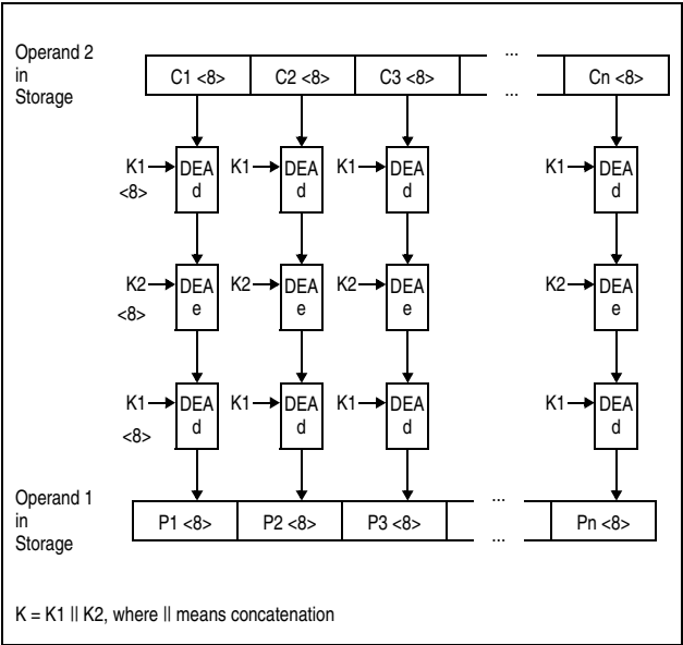
Figure 7-22. KM TDEA Decipher Operation Using 128-Bit Key
