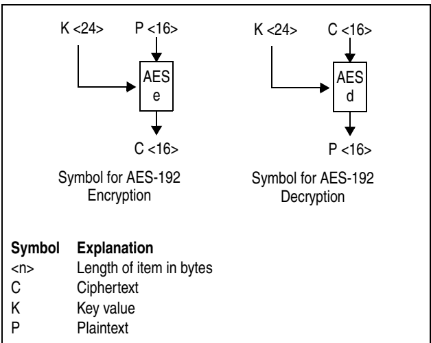
Figure 7-263. Symbols for AES-192 Encryption and Decryption
