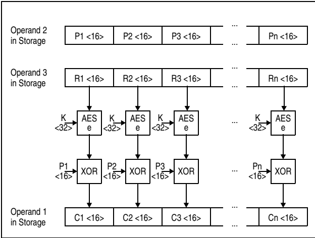
Figure 7-138. KMCTR AES Encipher Operation Using 256-Bit Key
