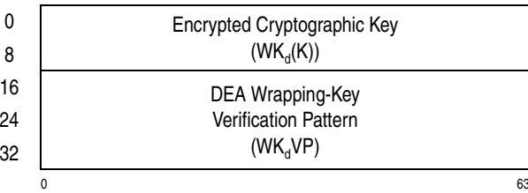
Figure 7-121. Parameter Block for KMCTR Encrypted-TDEA-128
