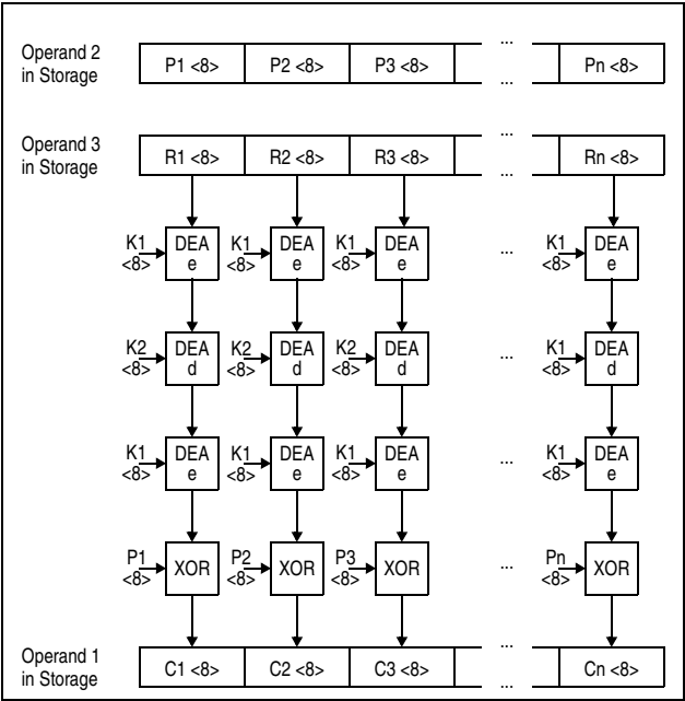
Figure 7-122. KMCTR TDEA Encipher Operation Using 128-Bit Key
