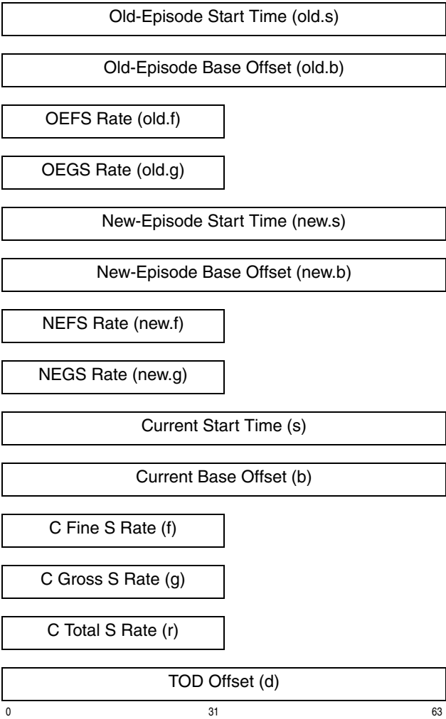
Figure 4-12. TOD-Clock-Steering Registers
