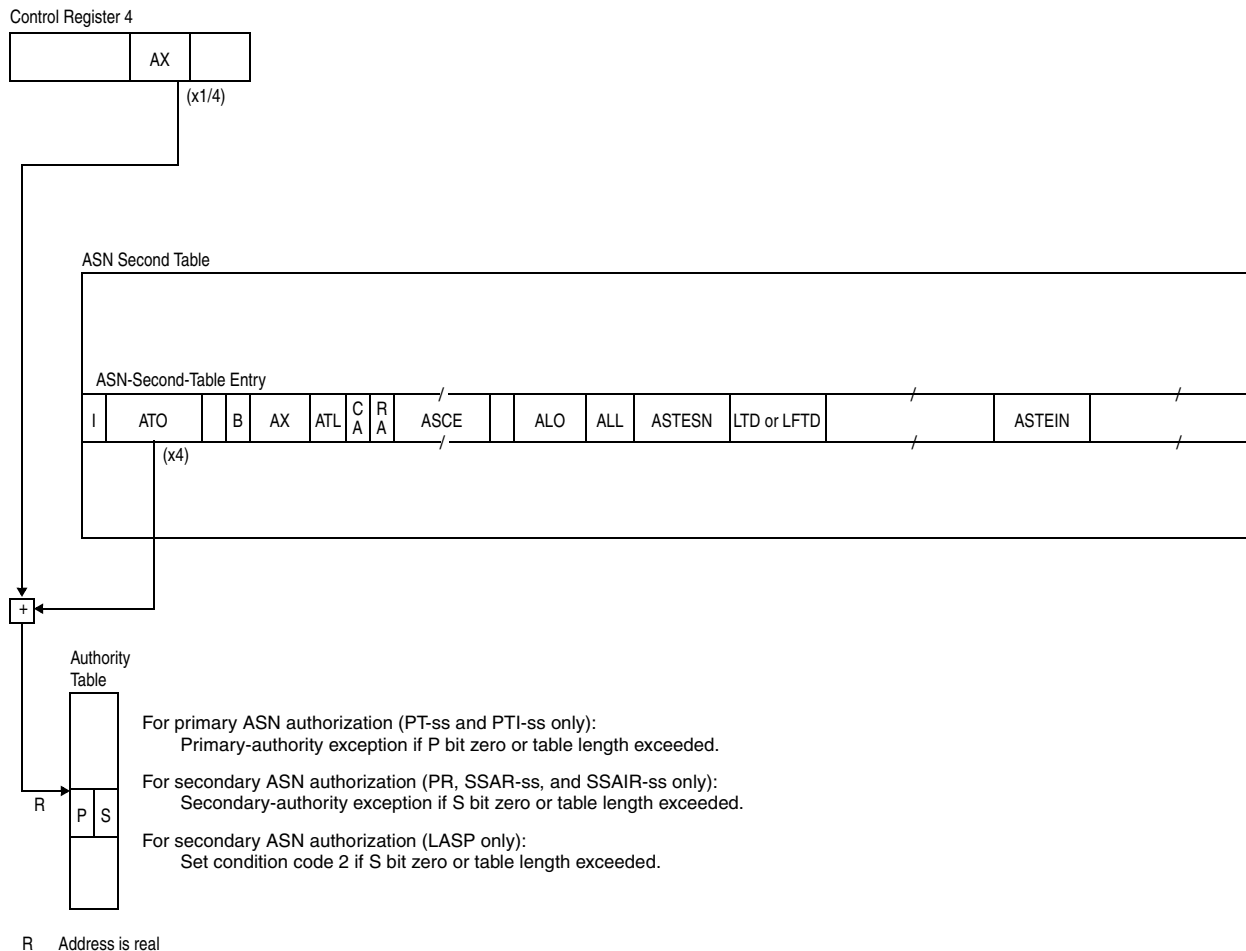
Figure 3-10. ASN Authorization
