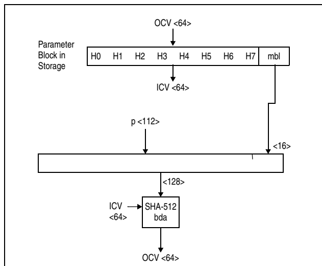
Figure 7-215. KLMD-SHA-512 Empty Block ( L = 0 )
