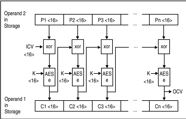
Figure 7-62. KMC AES Encipher Operation Using 128-Bit Key
