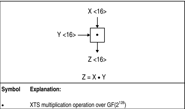
Figure 7-259. Symbol For XTS Multiplication Operation Over GF(2^{128})
