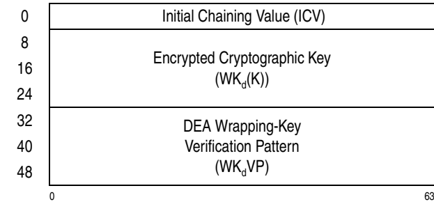
Figure 7-234. Parameter Block for KMAC-Encrypted-TDEA-192
