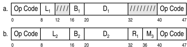
Figure 5-1. Basic Instruction Formats (Part 2 of 5)
