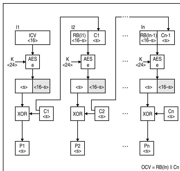
Figure 7-102. KMF-AES-192 Decipher Operation
