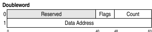
Figure 15-28. Modified-Indirect-Data-Address Word (MIDAW)
