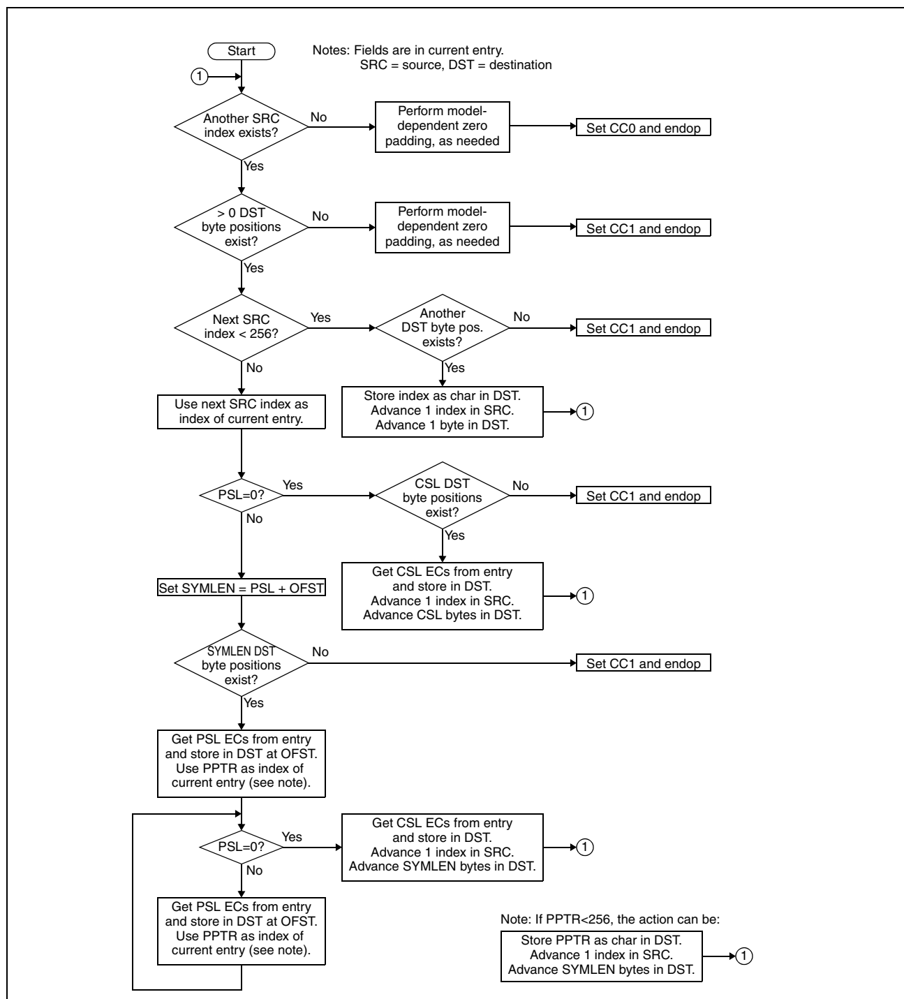
Figure 7-185. Expansion Process
