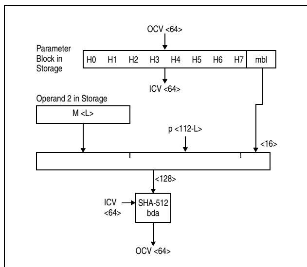
Figure 7-216. KLMD-SHA-512 Partial-Block Case 1 ( 1 \leq L \leq 111 )
