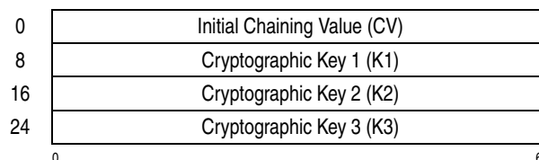
Figure 7-233. Parameter Block for KMAC-TDEA-192
