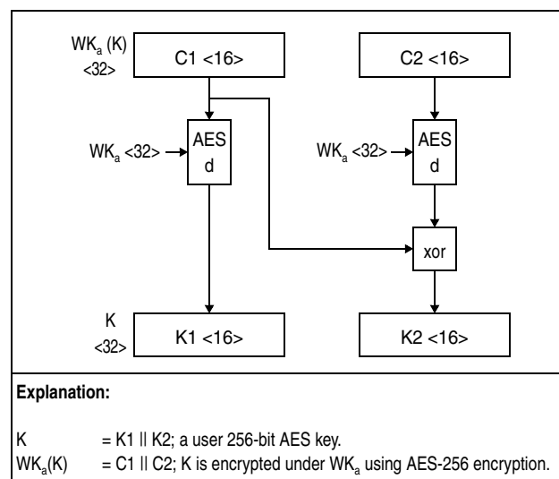
Figure 7-327. Decryption of 256-Bit AES Key Using WK_a
