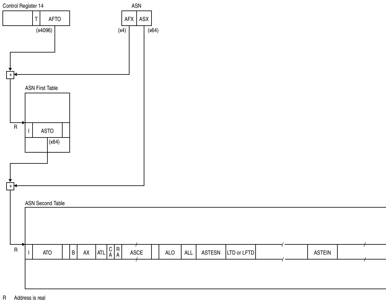
Figure 3-9. ASN Translation
