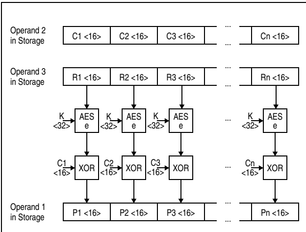
Figure 7-139. KMCTR AES Decipher Operation Using 256-Bit Key
