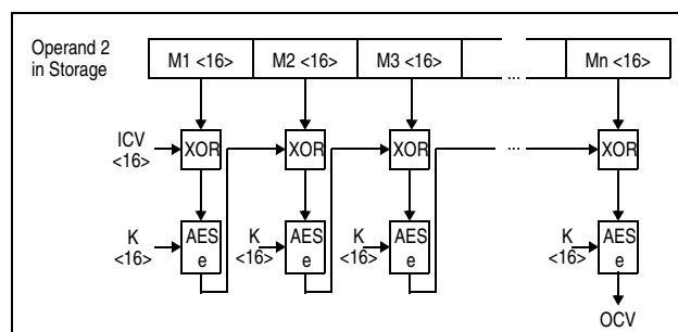
Figure 7-238. KMAC-AES-128
