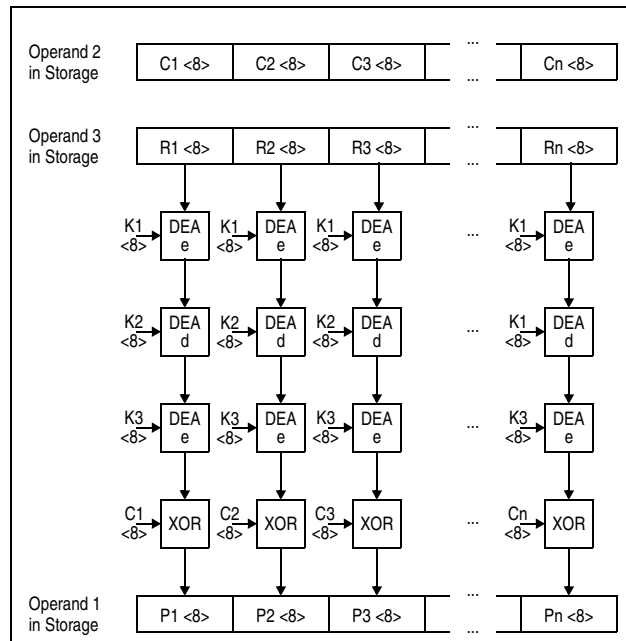
Figure 7-127. KMCTR TDEA Decipher Operation Using 192-Bit Key
