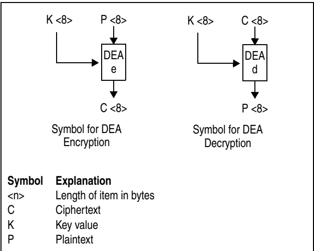
Figure 7-144. Symbols for DEA Encryption and Decryption
