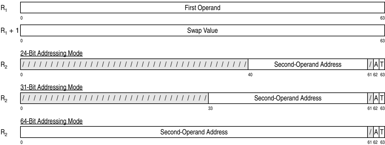
Figure 10-7. Register Contents for COMPARE AND SWAP AND PURGE (CSPG)
