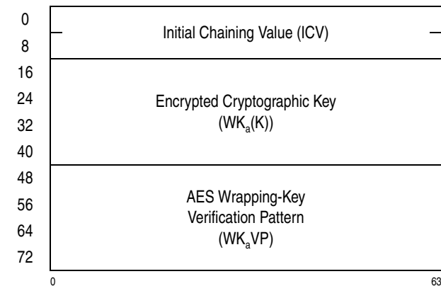
Figure 7-243. Parameter Block for KMAC-Encrypted-AES-256
