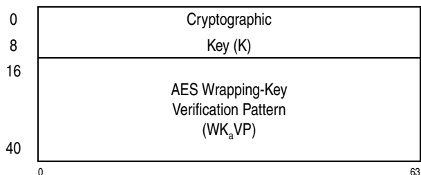
Figure 10-41. Parameter Block for PCKMO-Encrypt-AES-128-Key
