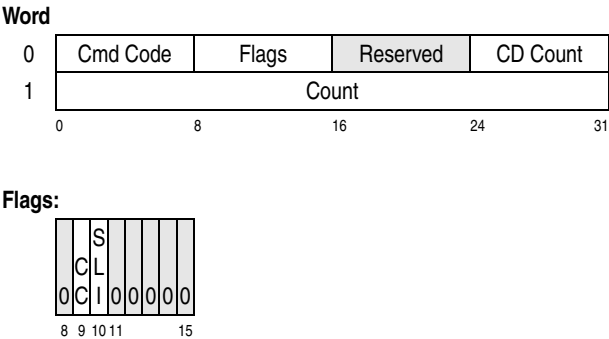
Figure 15-11. Device-Command Word (DCW)
