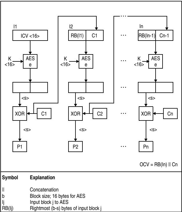
Figure 7-98. KMF-AES-128 Decipher Operation
