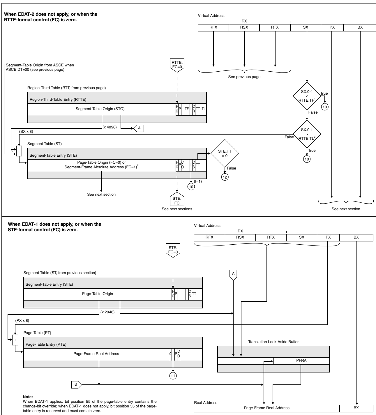
Figure 3-11. Translation Process (Part 2 of 3)
