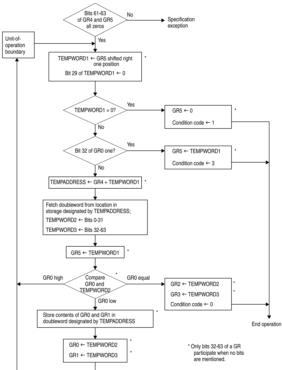
Figure 7-305. Execution of UPDATE TREE in the 24-Bit or 31-Bit Addressing Mode
