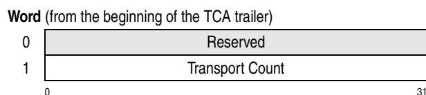
Figure 15-12. Transport-Command-Area Trailer (TCAT)
