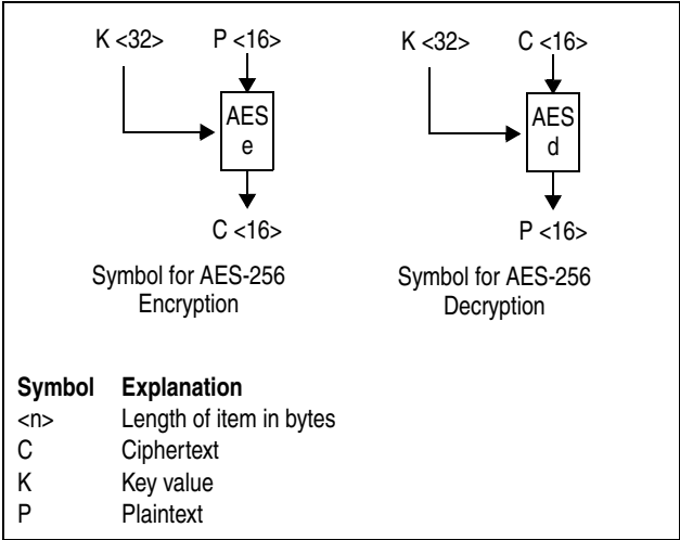
Figure 7-264. Symbols for AES-256 Encryption and Decryption
