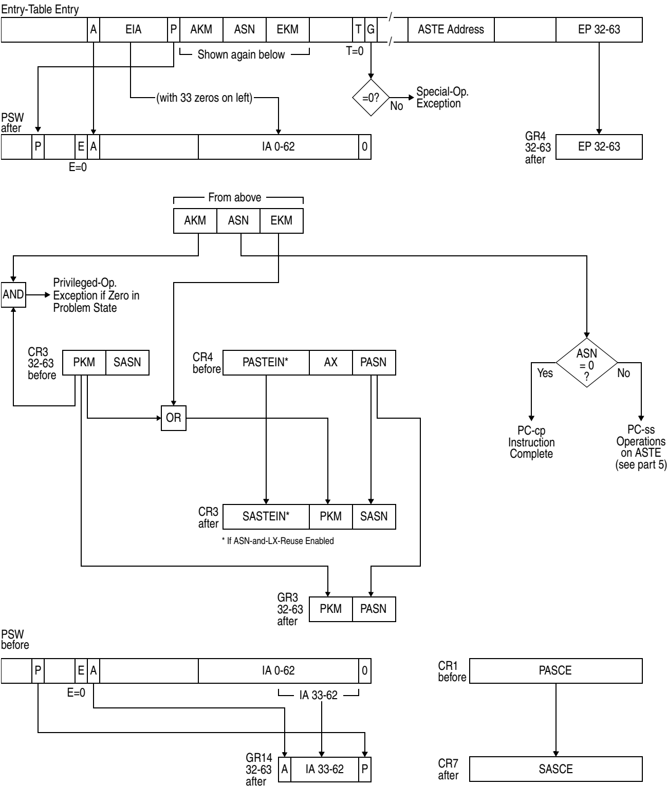
Figure 10-60. Execution of PROGRAM CALL (Part 1 of 5).
