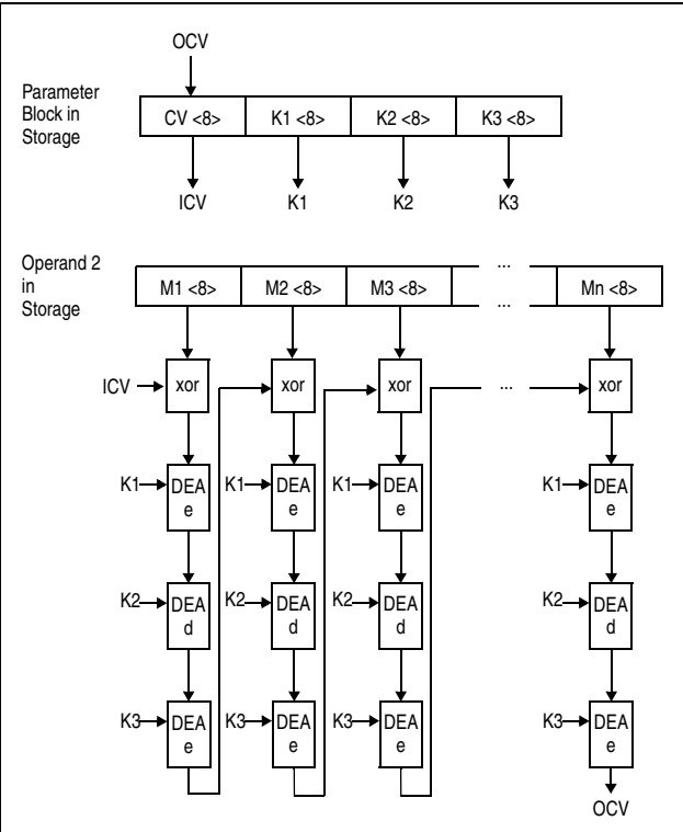
Figure 7-235. MAC Computation Using 192-bit TDEA Key
