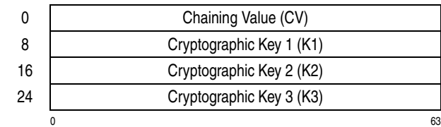
Figure 7-91. Parameter Block for KMF-TDEA-192
