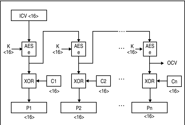
Figure 7-164. KMO-AES-128 Decipher Operation
