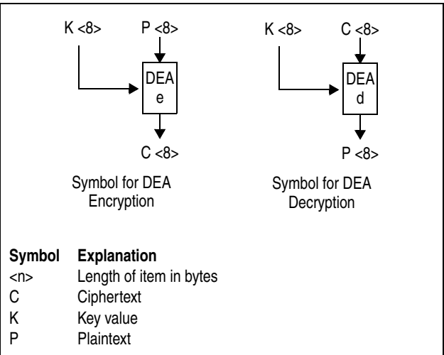
Figure 7-78. Symbols for DEA Encryption and Decryption
