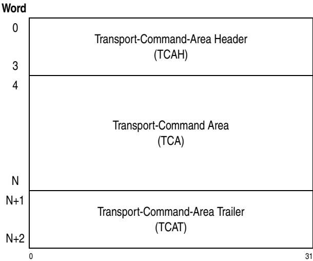
Figure 15-8. Transport-Command-Control Block (TCCB)
