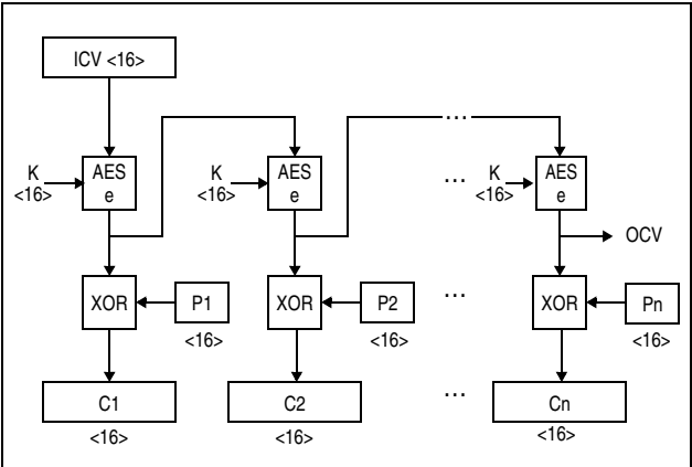
Figure 7-163. KMO-AES-128 Encipher Operation
