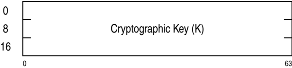
Figure 7-132. Parameter Block for KMCTR-AES-192
