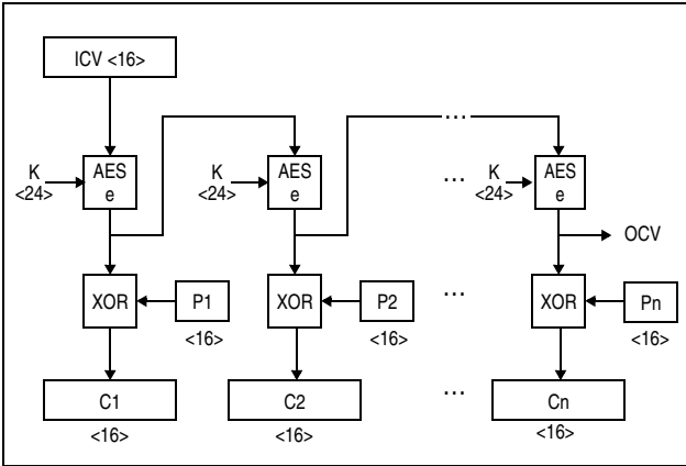
Figure 7-167. KMO-AES-192 Encipher Operation
