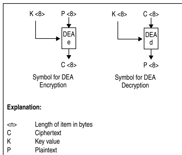
Figure 7-309. Symbols for DEA Encryption and Decryption
