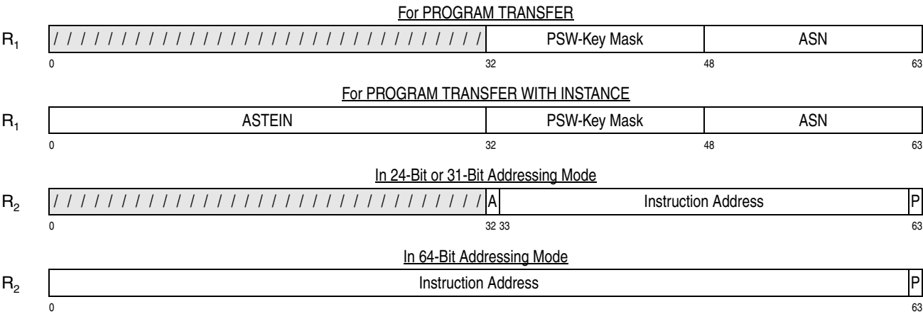
Figure 10-62. Register Contents for PROGRAM TRANSFER (WITH INSTANCE)
