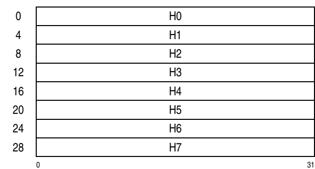
Figure 7-196. Parameter Block for KIMD-SHA-256
