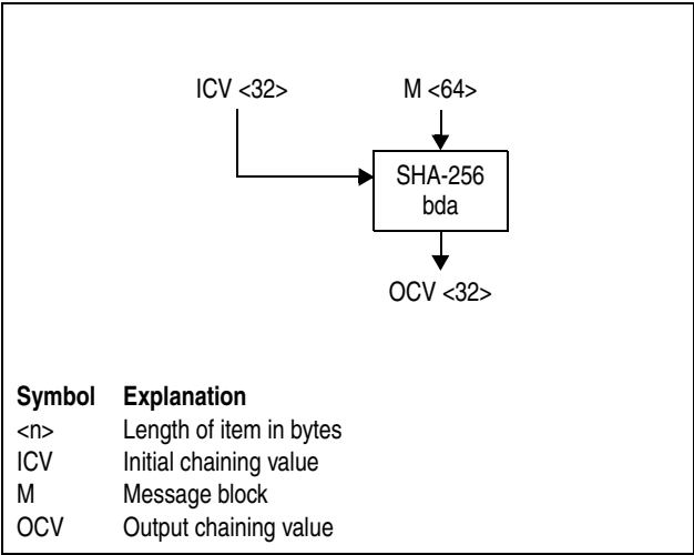
Figure 7-190. Symbol for SHA-256 Block Digest Algorithm
