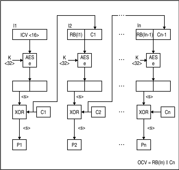
Figure 7-106. KMF-AES-256 Decipher Operation
