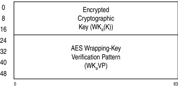
Figure 7-133. Parameter Block for KMCTR-Encrypted-AES-192
