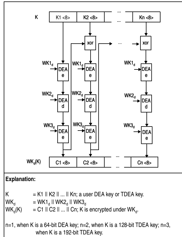
Figure 7-311. Encryption of DEA or TDEA Key Using WK_d
