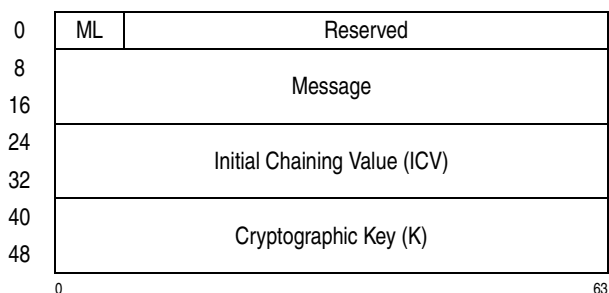
Figure 7-275. Parameter Block for PCC-Compute-Last-Block-CMAC-Using-AES-128
