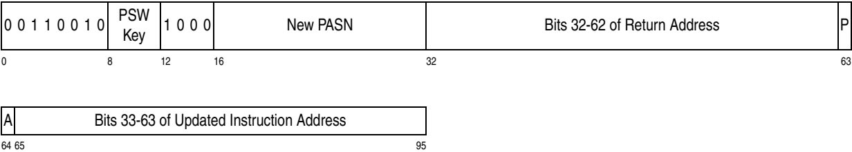
Figure 4-6. Trace Entries (Part 4 of 7)
