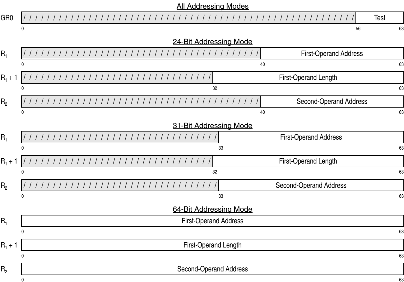
Figure 7-303. Register Contents for TRANSLATE EXTENDED
