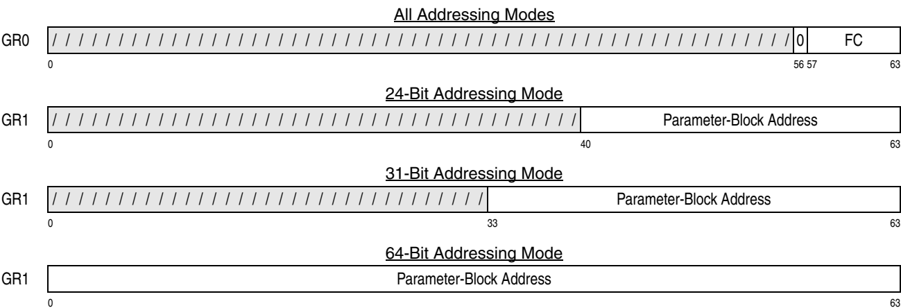
Figure 10-36. General Register Assignment for PCKMO
