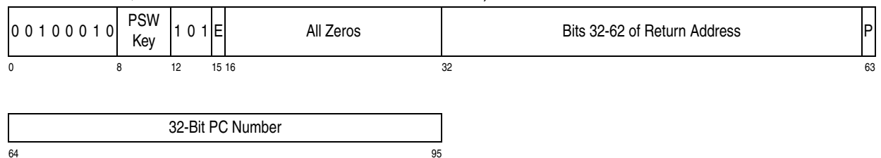
Figure 4-6. Trace Entries (Part 3 of 7)
