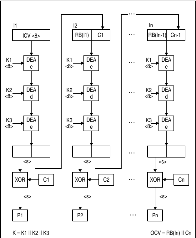
Figure 7-94. KMF-TDEA-192 Decipher Operation
