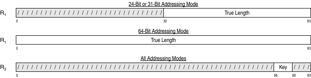
Figure 10-30. Register Contents of MOVE WITH KEY
