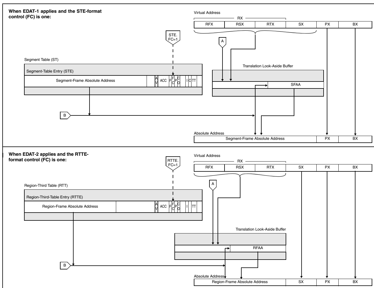
Figure 3-11. Translation Process (Part 3 of 3)
