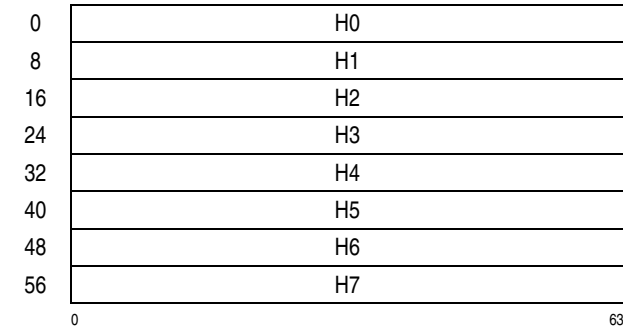
Figure 7-198. Parameter Block for KIMD-SHA-512
