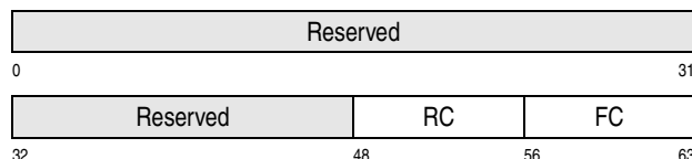
Figure 10-58. General-Register R_1 Format
