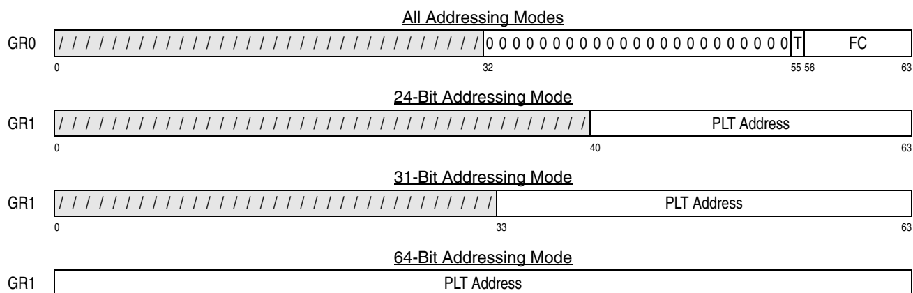
Figure 7-292. General Register Assignment for PLO
