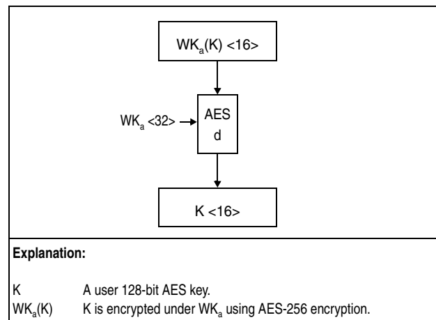
Figure 7-314. Decryption of 128-Bit AES Key Using WK_a
