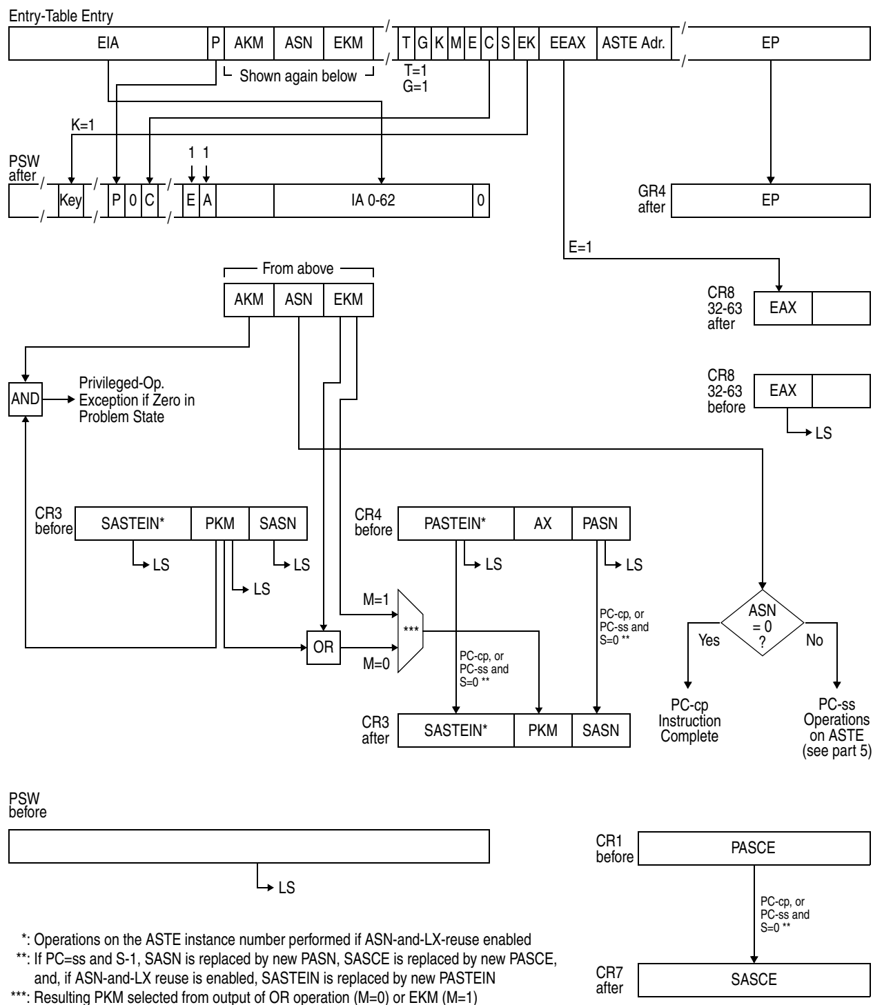
Figure 10-60. Execution of PROGRAM CALL (Part 3 of 5).
