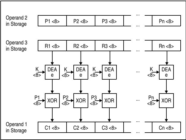
Figure 7-118. KMCTR DEA Encipher Operation Using 64-Bit Key
