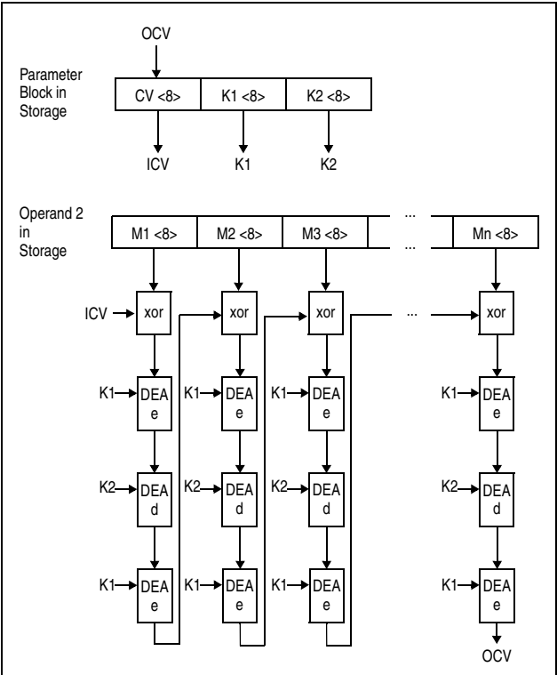
Figure 7-232. MAC Computation Using 128-bit TDEA Key
