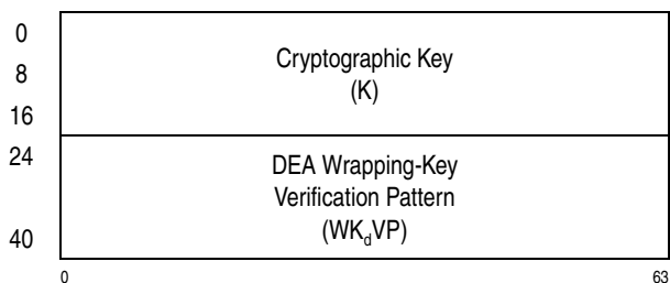
Figure 10-40. Parameter Block for PCKMO-Encrypt-TDEA-192-Key
