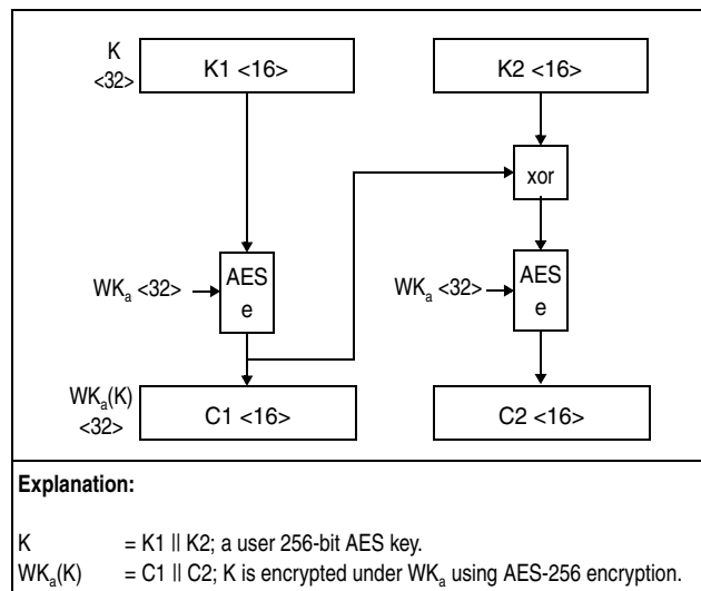
Figure 7-317. Encryption of 256-Bit AES Key Using WK_a
