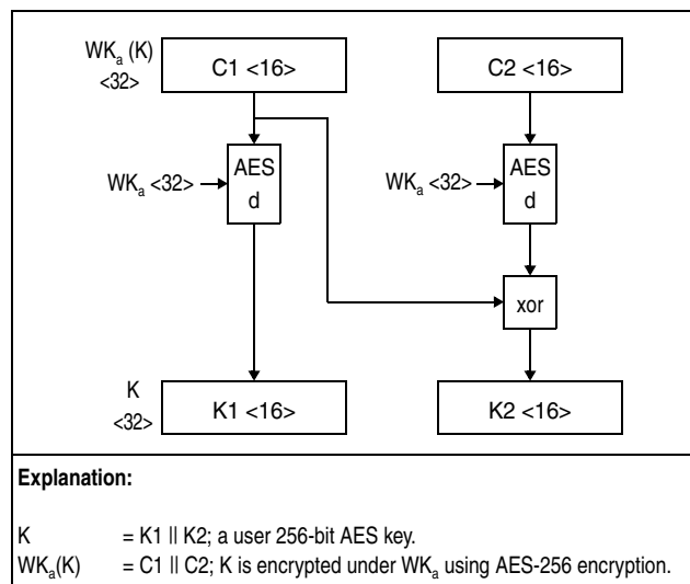
Figure 7-318. Decryption of 256-Bit AES Key Using WK_a
