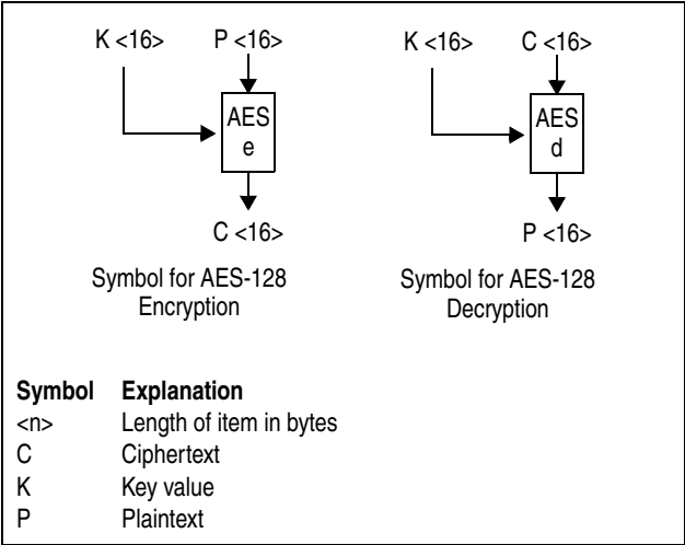
Figure 7-262. Symbols for AES-128 Encryption and Decryption
