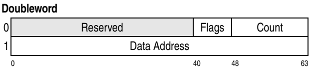
Figure 15-26. Modified-Indirect-Data-Address Word (MIDAW)
