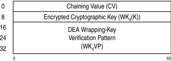
Figure 7-84. Parameter Block for KMF-Encrypted-DEA
