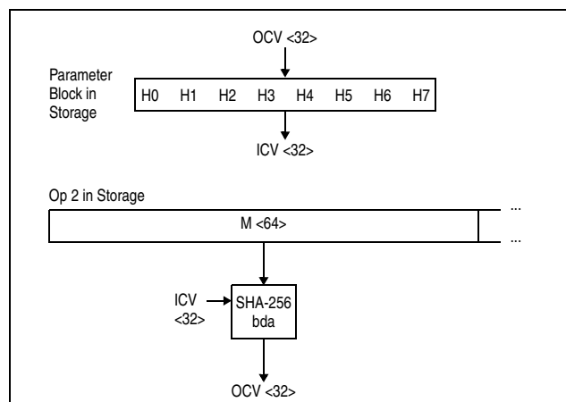
Figure 7-209. KLMD-SHA-256 Full Block ( L \geq 64 )
