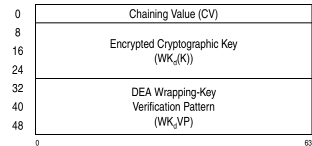
Figure 7-92. Parameter Block for KMF-Encrypted-TDEA-192
