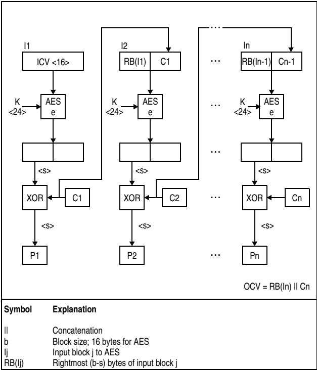
Figure 7-102. KMF-AES-192 Decipher Operation
