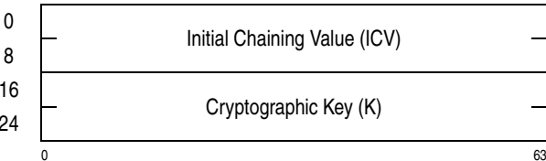
Figure 7-236. Parameter Block for KMAC-AES-128
