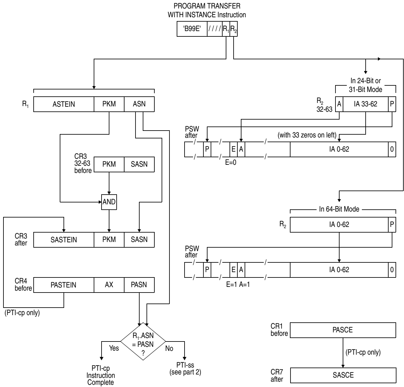
Figure 10-65. Execution of PROGRAM TRANSFER WITH INSTANCE (Part 1 of 2).
