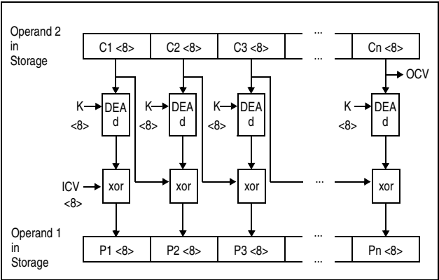
Figure 7-51. KMC DEA Decipher Operation Using 64-Bit Key
