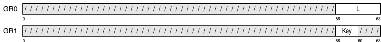
Figure 10-29. Register Contents of MOVE WITH DESTINATION KEY
