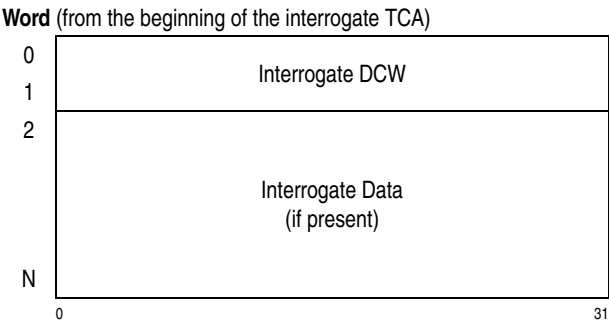
Figure 15-16. Interrogate Transport-Command Area (TCA)
