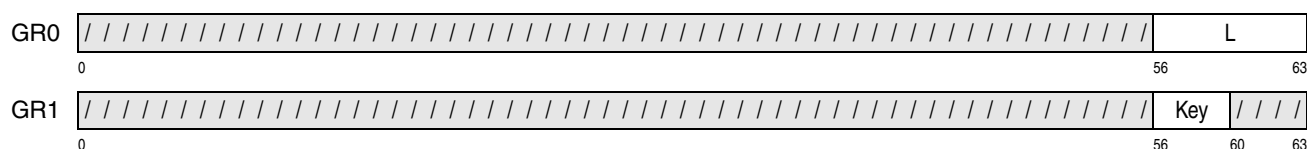
Figure 10-34. Register Contents of MOVE WITH SOURCE KEY
