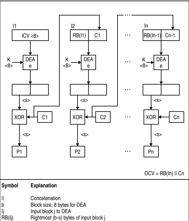
Figure 7-86. KMF-DEA Decipher Operation
