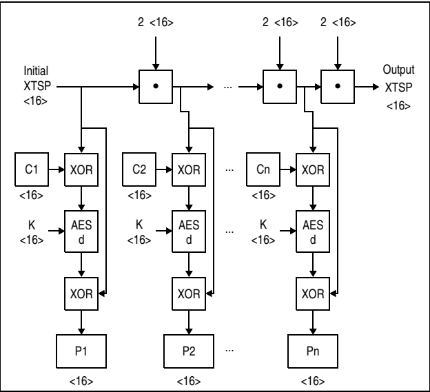
Figure 7-42. XTS-AES-128 Decipher Operation
