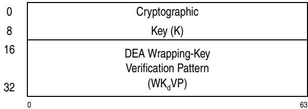
Figure 10-39. Parameter Block for PCKMO-Encrypt-TDEA-128-Key
