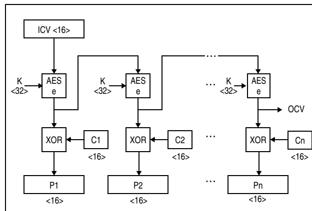
Figure 7-172. KMO-AES-256 Decipher Operation
