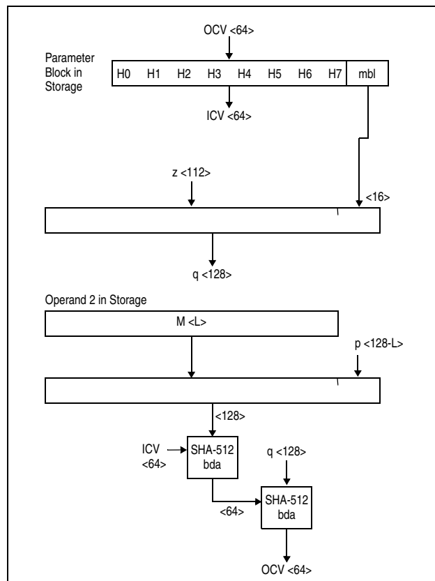
Figure 7-217. KLMD-SHA-512 Partial-Block Case 2 ( 112 \leq L \leq 127 )
