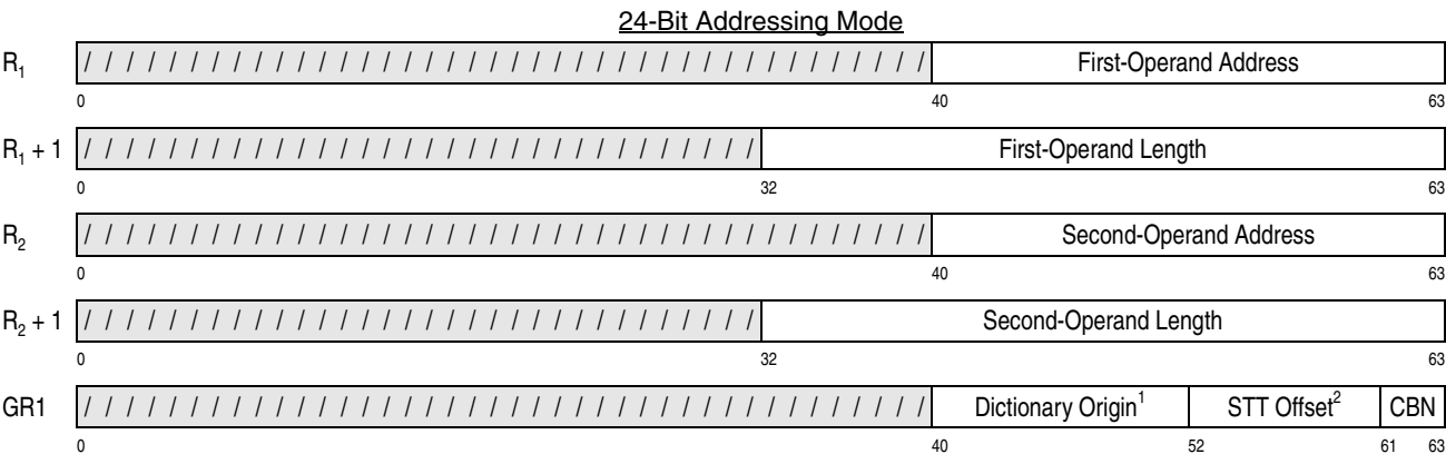
Figure 7-183. Register Contents for COMPRESSION CALL (Part 1 of 2)
