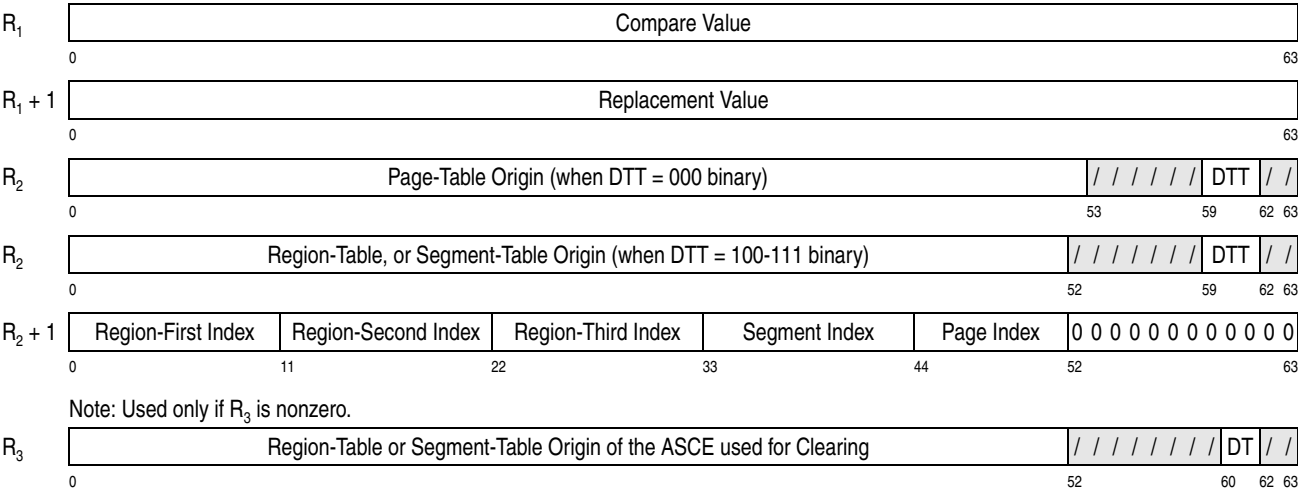
Figure 10-5. Register Contents for COMPARE AND REPLACE DAT TABLE ENTRY
