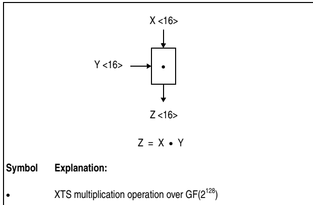
Figure 7-9. Symbol For XTS Multiplication Operation Over GF(2^{128})
