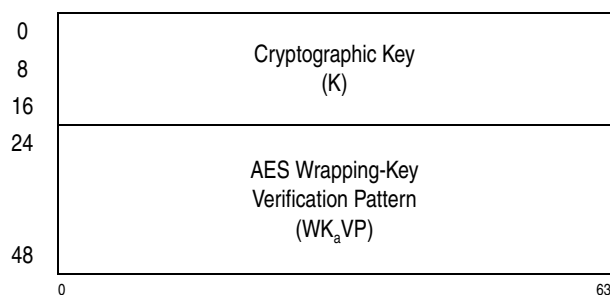
Figure 10-42. Parameter Block for PCKMO-Encrypt-AES-192-Key
