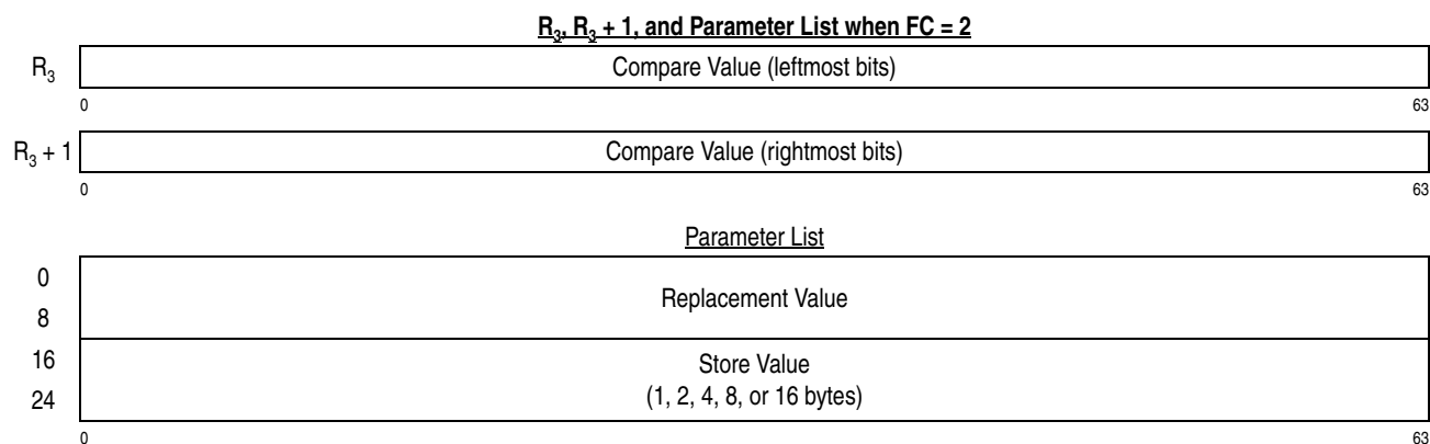
Figure 7-178. Register Contents for COMPARE AND SWAP AND STORE
