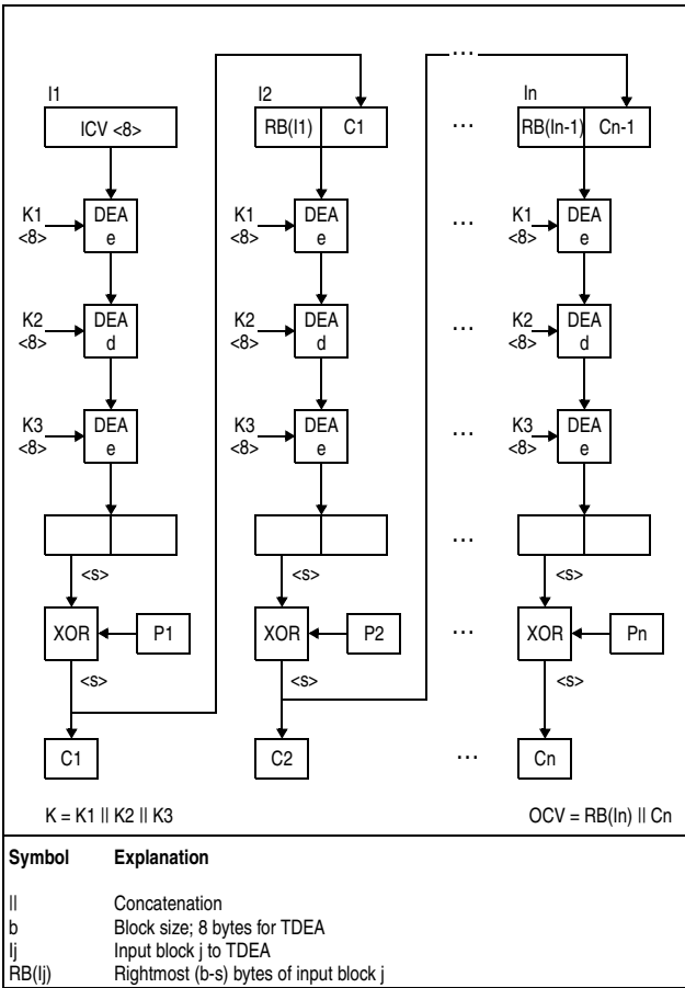
Figure 7-93. KMF-TDEA-192 Encipher Operation
