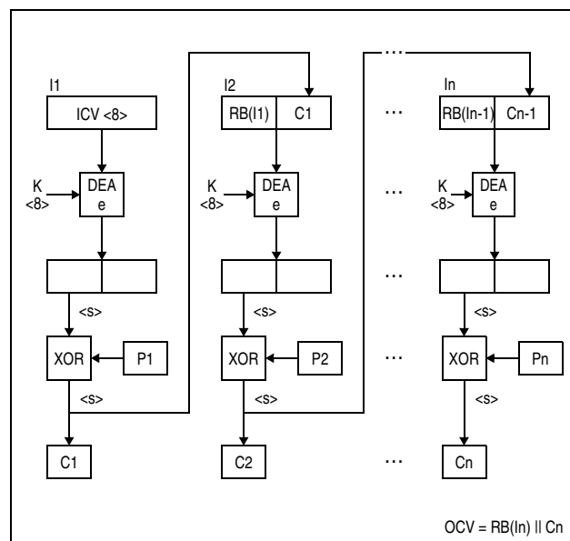
Figure 7-50. KMF-DEA Encipher Operation
