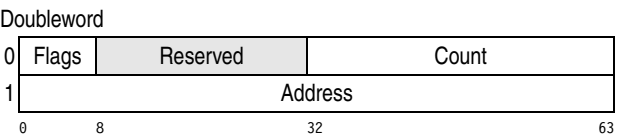
Figure 15-27. Transport-Indirect-Data-Address Word (TIDAW)
