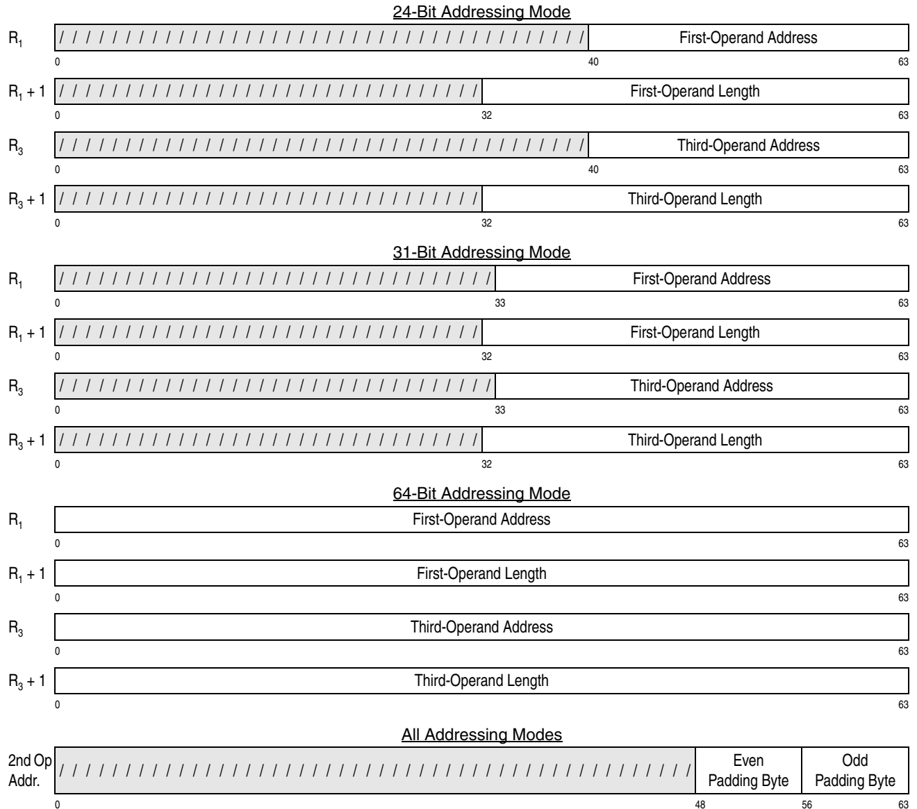
Figure 7-255. Register Contents and Second-Operand Address for MOVE LONG UNICODE
