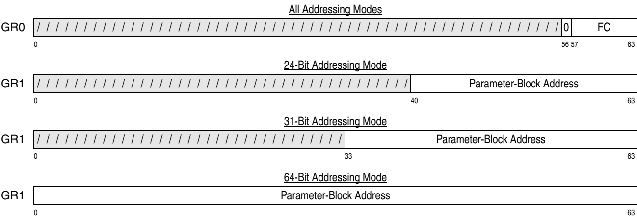
Figure 10-45. General Register Assignment for PERFORM TIMING FACILITY FUNCTION
