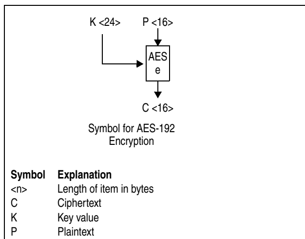
Figure 7-113. Symbols for AES-192 Encryption
