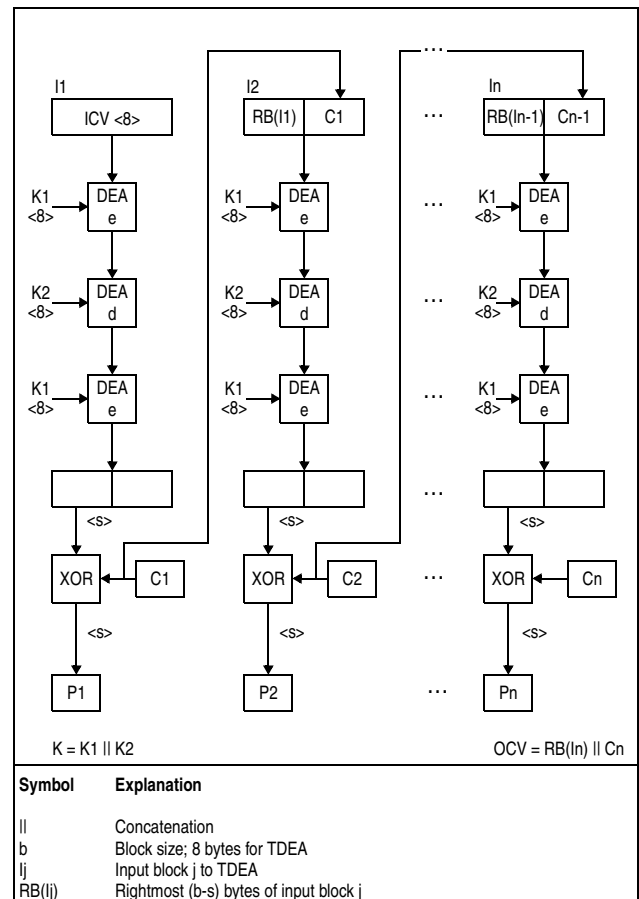
Figure 7-90. KMF-TDEA-128 Decipher Operation
