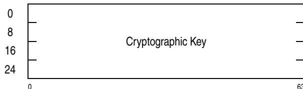
Figure 7-35. Parameter Block for KM-AES-256
