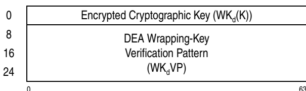
Figure 7-117. Parameter Block for KMCTR-Encrypted-DEA
