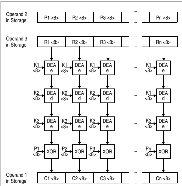
Figure 7-126. KMCTR TDEA Encipher Operation Using 192-Bit Key
