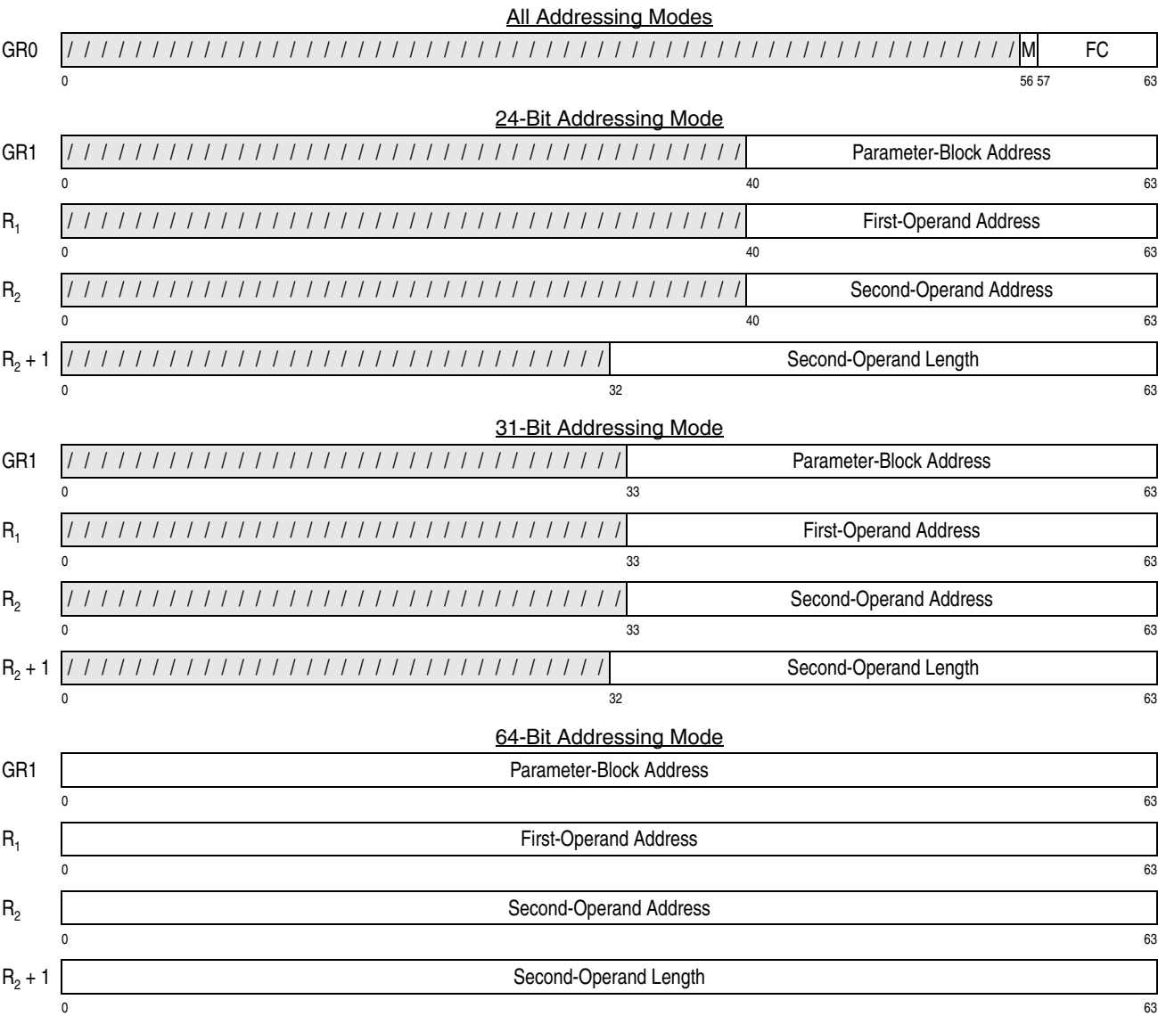
Figure 7-142. General Register Assignment for KMO
