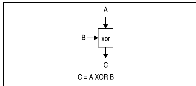
Figure 7-8. Symbol For Bit-Wise Exclusive OR
