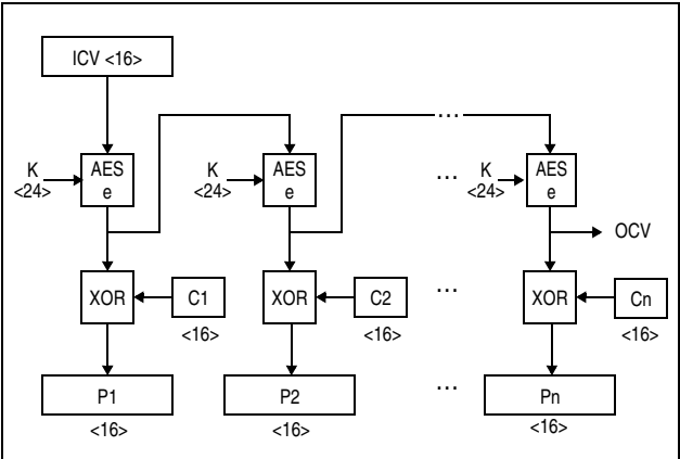
Figure 7-168. KMO-AES-192 Decipher Operation
