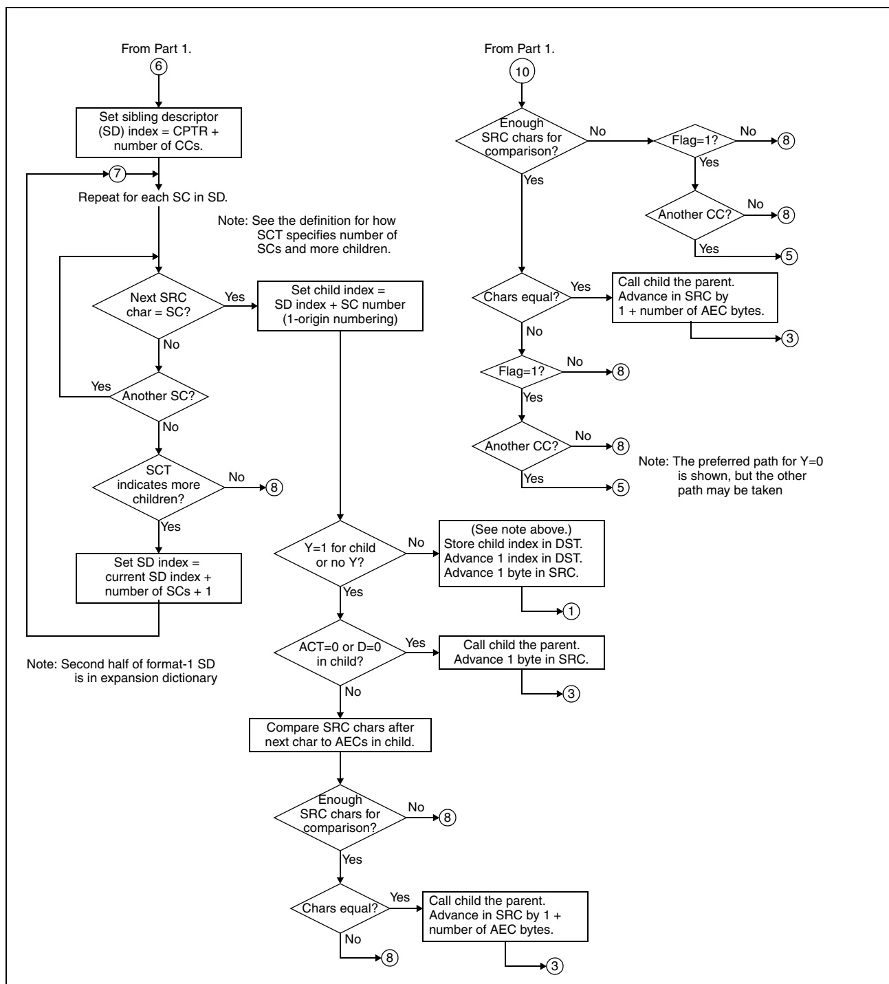
Figure 7-184. Compression Process (Part 2 of 2)
