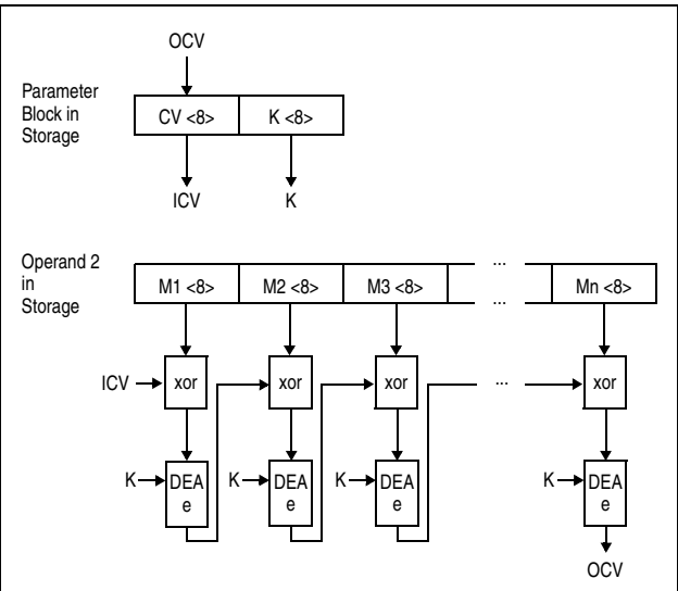
Figure 7-229. MAC Computation Using 64-bit DEA Key
