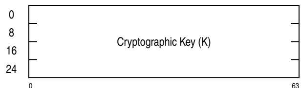
Figure 7-136. Parameter Block for KMCTR-AES-256
