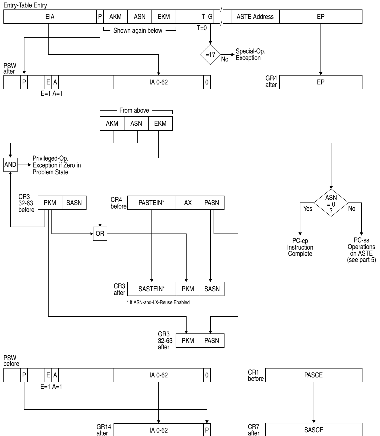
Figure 10-60. Execution of PROGRAM CALL (Part 2 of 5).
