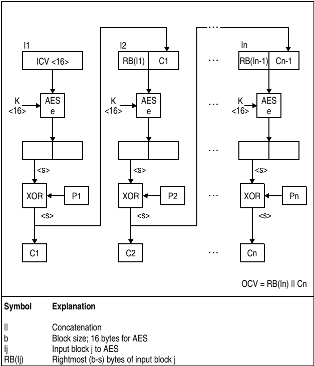
Figure 7-97. KMF-AES-128 Encipher Operation
