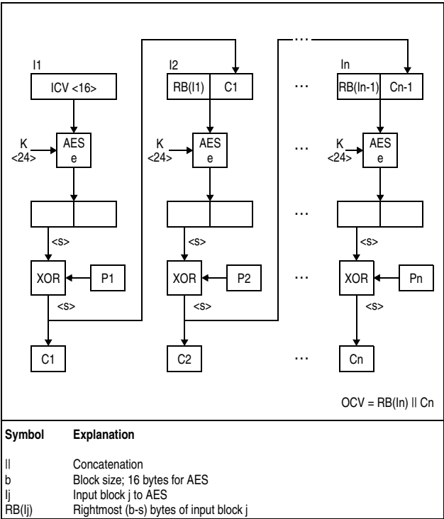
Figure 7-101. KMF-AES-192 Encipher Operation
