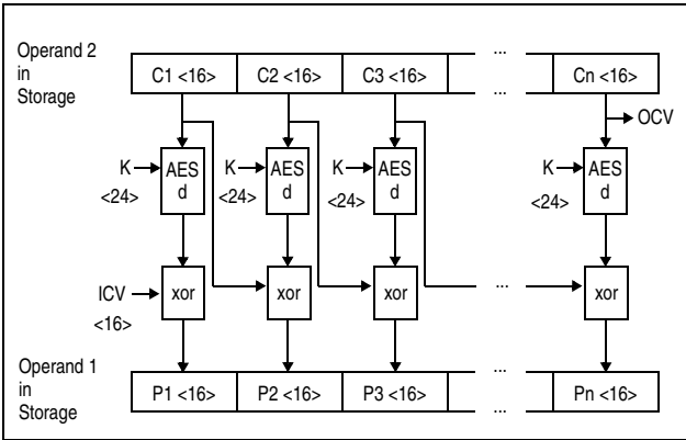
Figure 7-67. KMC AES Decipher Operation Using 192-Bit Key
