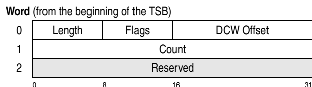
Figure 15-19. Transport-Status Header (TSH)
