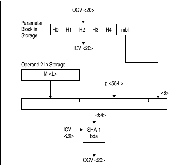
Figure 7-206. KLMD-SHA-1 Partial-Block Case 1 ( 1 \leq L \leq 55 )
