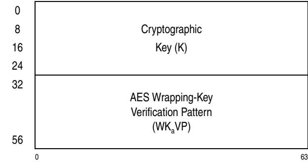
Figure 10-43. Parameter Block for PCKMO-Encrypt-AES-256-Key
