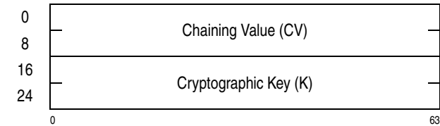
Figure 7-161. Parameter Block for KMO-AES-128
