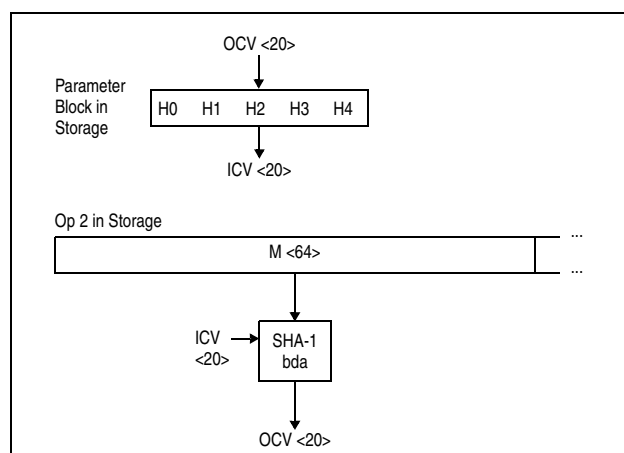
Figure 7-204. KLMD-SHA-1 Full Block ( L \geq 64 )
