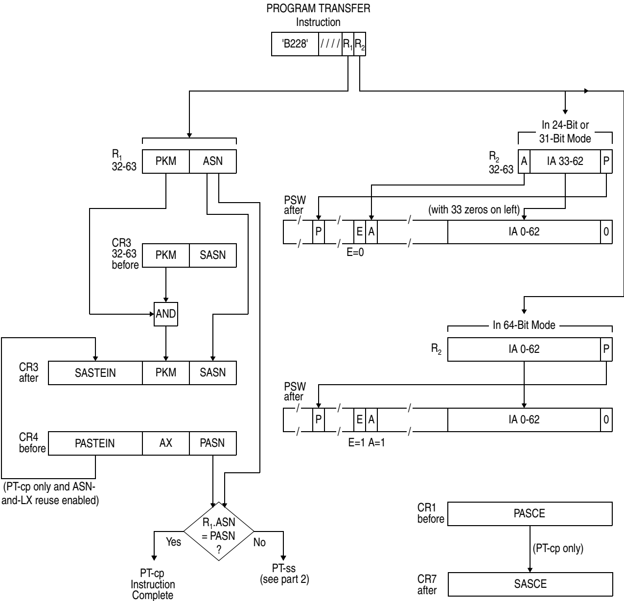
Figure 10-64. Execution of PROGRAM TRANSFER (Part 1 of 2).
