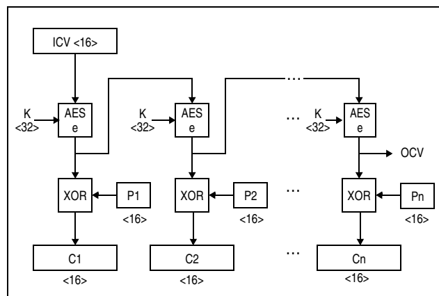
Figure 7-171. KMO-AES-256 Encipher Operation
