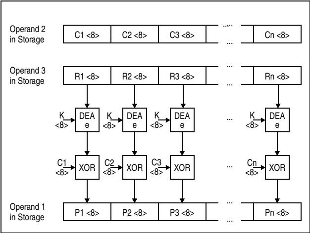
Figure 7-119. KMCTR DEA Decipher Operation Using 64-Bit Key
