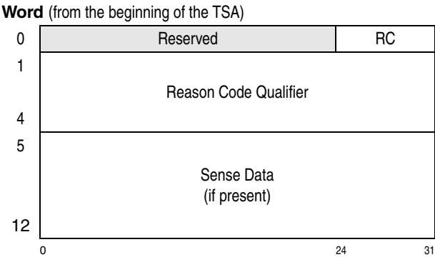
Figure 15-21. Device-Detected-Program-Check Transport-Status Area (TSA)
