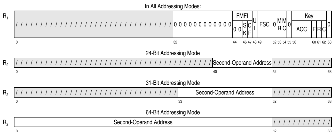
Figure 10-44. Register Contents for PERFORM FRAME-MANAGEMENT FUNCTION
