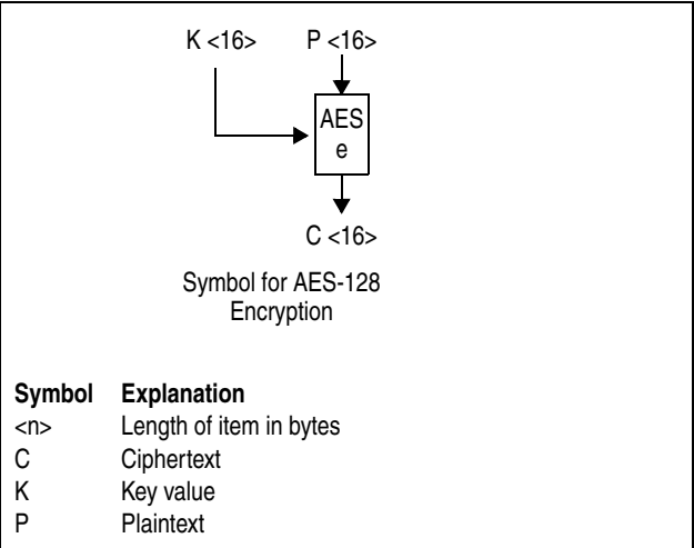
Figure 7-79. Symbols for AES-128 Encryption
