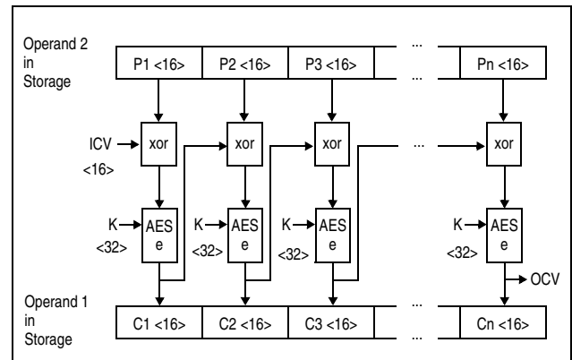
Figure 7-70. KMC AES Encipher Operation Using 256-Bit Key
