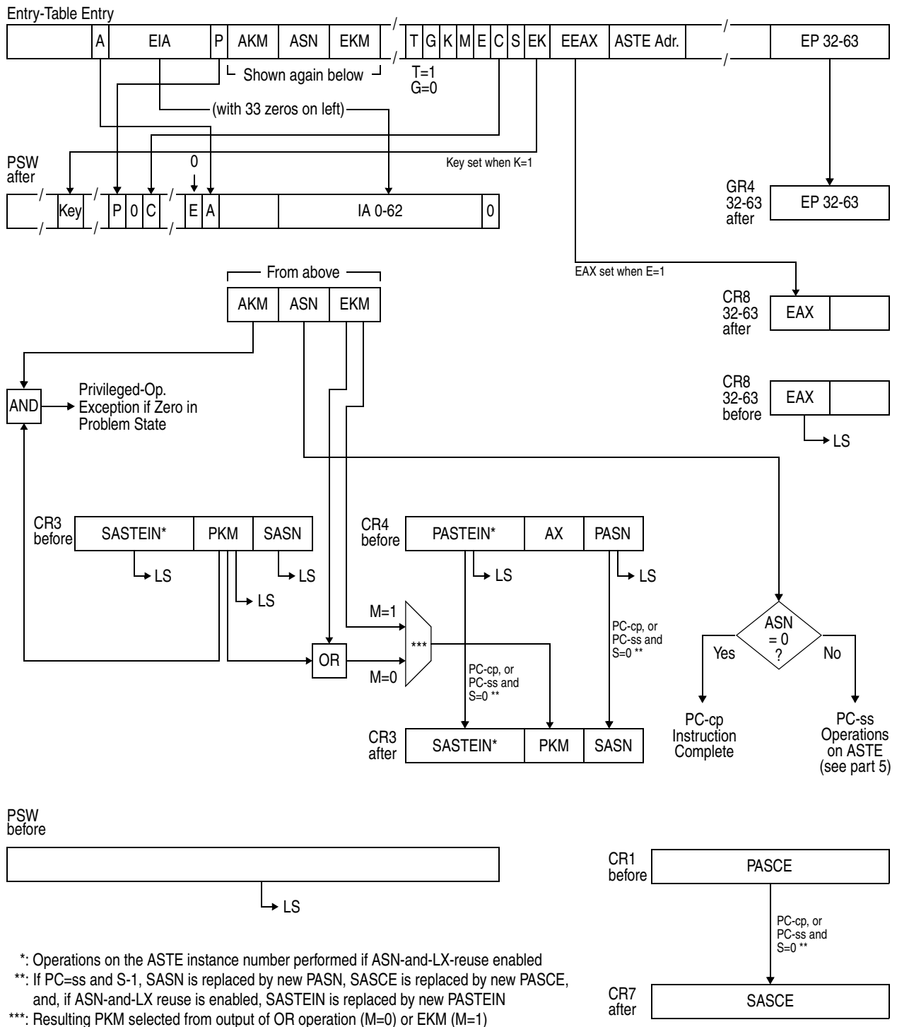
Figure 10-60. Execution of PROGRAM CALL (Part 4 of 5).
