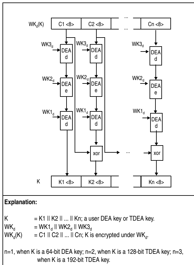
Figure 7-312. Decryption of DES or TDES Key Using WK_d
