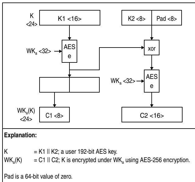
Figure 7-315. Encryption of 192-Bit AES Key Using WK_a
