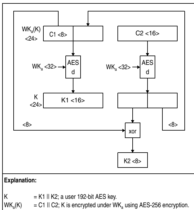
Figure 7-316. Decryption of 192-Bit AES Key Using WK_a
