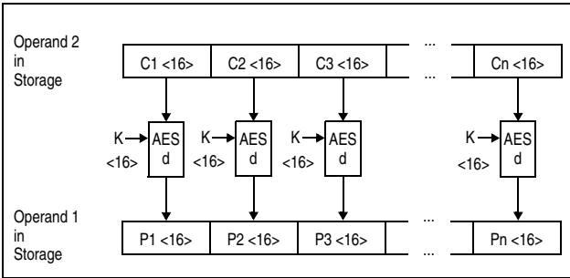
Figure 7-30. KM-AES Decipher Operation Using 128-Bit Key
