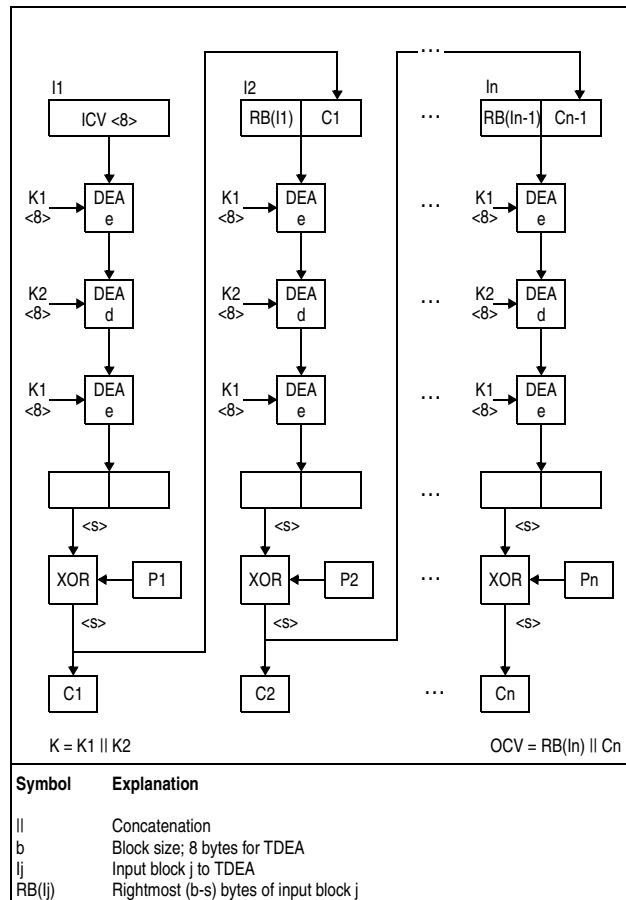
Figure 7-89. KMF-TDEA-128 Encipher Operation
