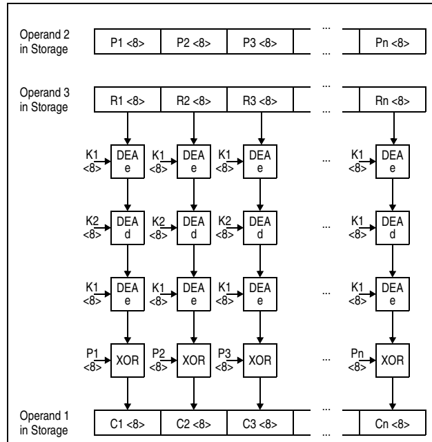
Figure 7-122. KMCTR TDEA Encipher Operation Using 128-Bit Key
