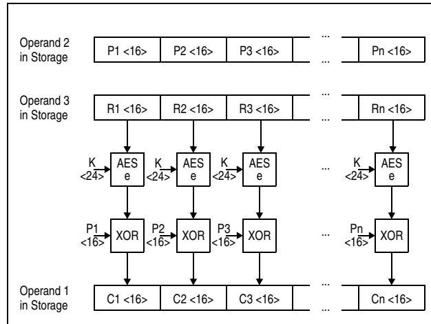
Figure 7-134. KMCTR AES Encipher Operation Using 192-Bit Key
