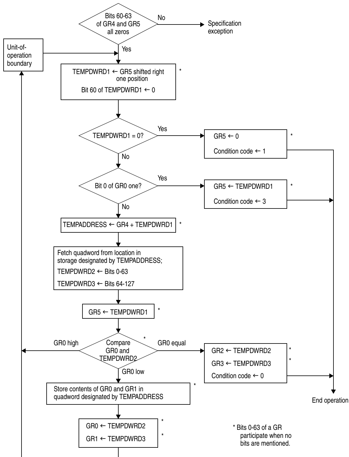
Figure 7-306. Execution of UPDATE TREE in the 64-Bit Addressing Mode
