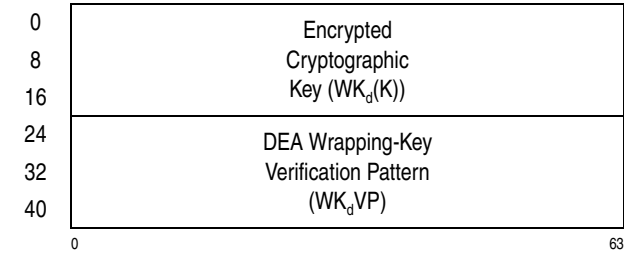
Figure 7-125. Parameter Block for KMCTR-Encrypted-TDEA-192
