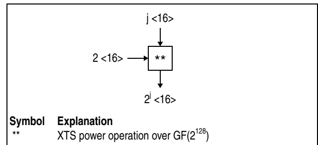
Figure 7-260. Symbol For XTS Power Operation Over GF(2^{128})
