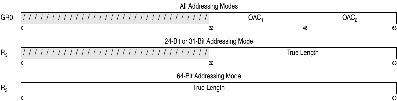
Figure 10-32. Register Contents for MOVE WITH OPTIONAL SPECIFICATIONS
