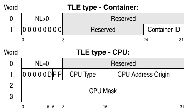
Figure 10-70. Topology-List Entries
