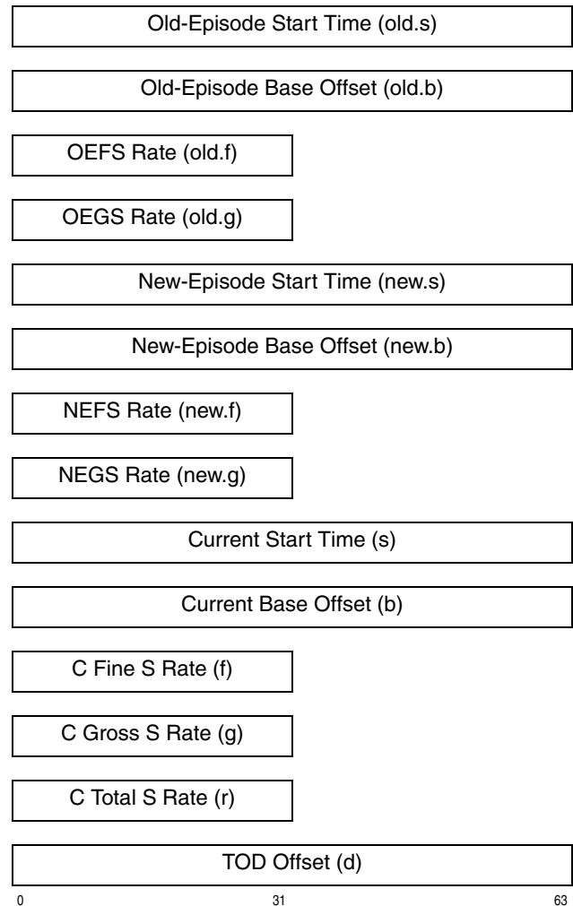
Figure 4-11. TOD-Clock-Steering Registers
