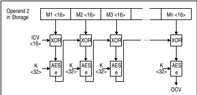
Figure 7-243. KMAC-AES-256
