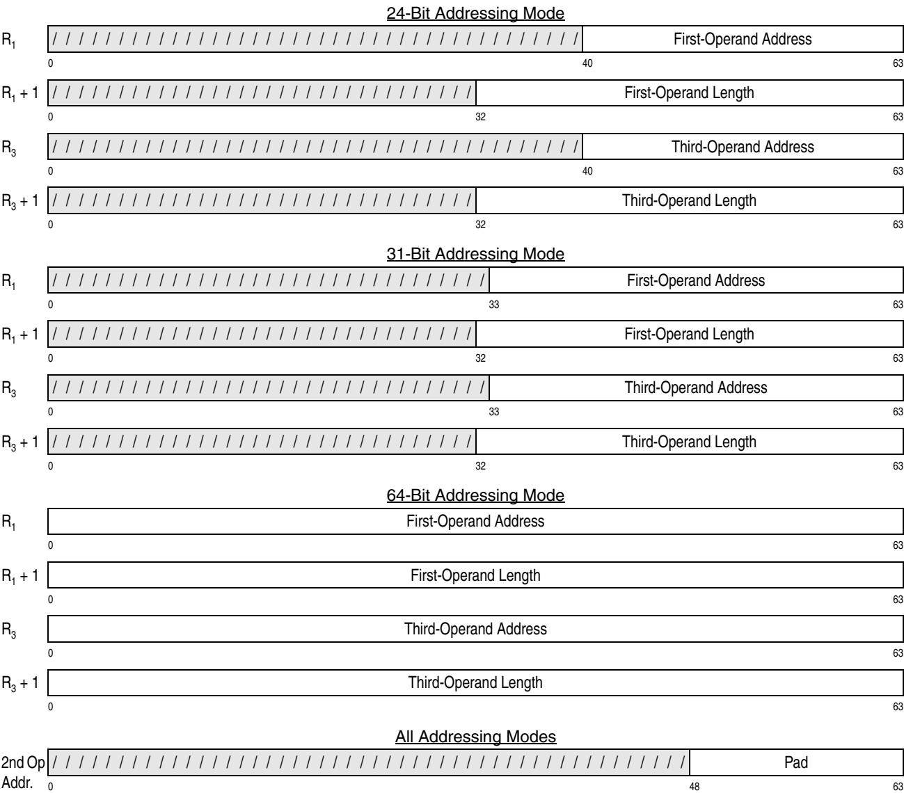
Figure 7-180. Register Contents and Second-Operand Address for COMPARE LOGICAL LONG UNICODE
