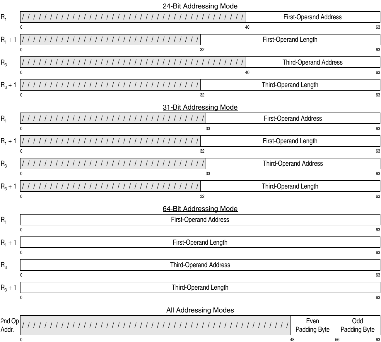
Figure 7-254. Register Contents and Second-Operand Address for MOVE LONG UNICODE
