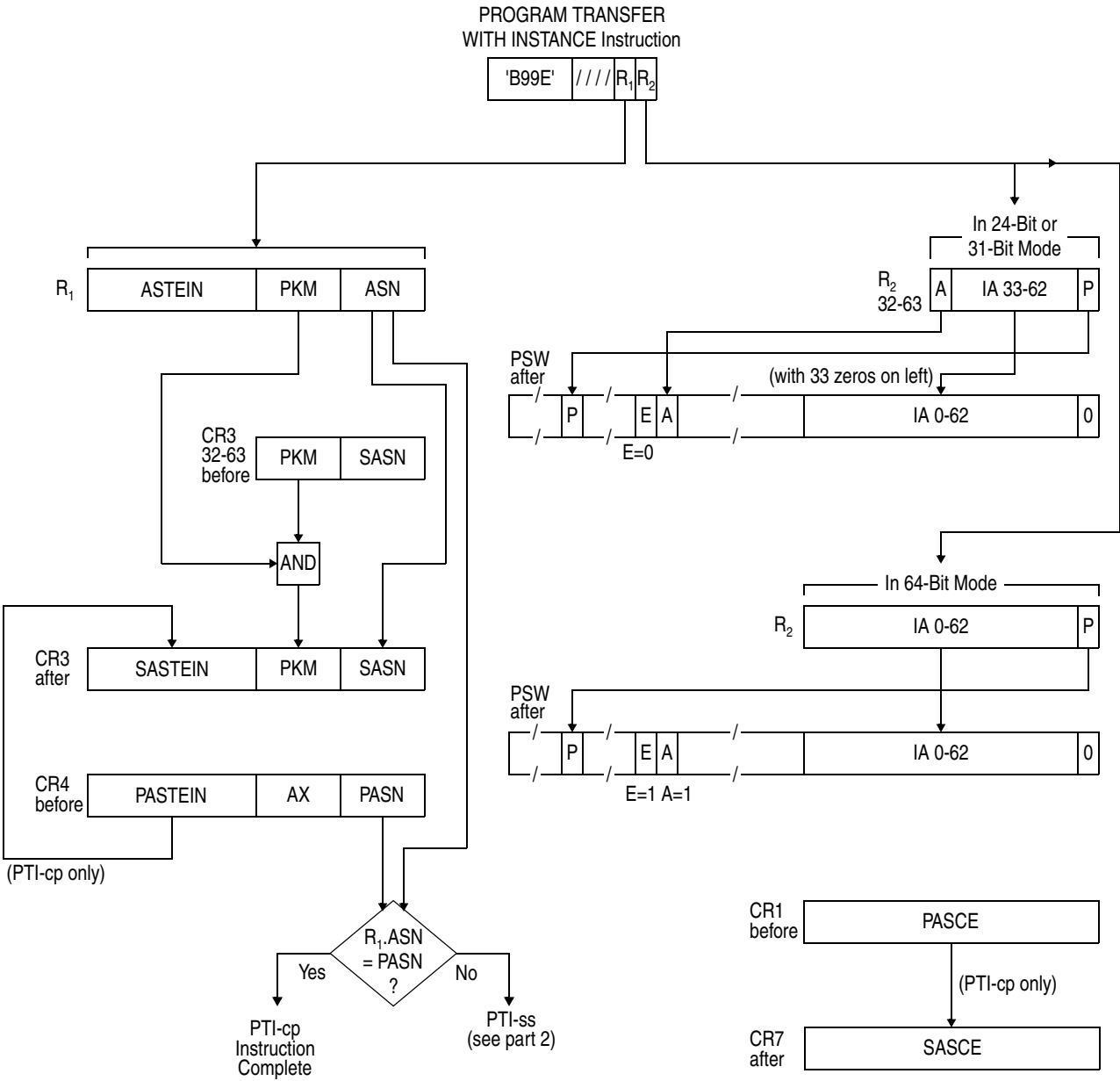
Figure 10-63. Execution of PROGRAM TRANSFER WITH INSTANCE (Part 1 of 2).
