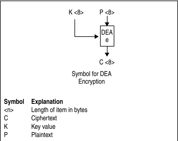
Figure 7-110. Symbols for DEA Encryption
