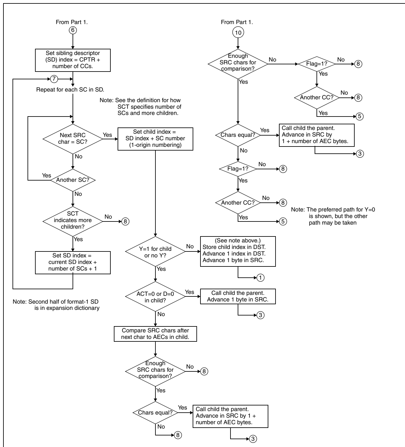
Figure 7-183. Compression Process (Part 2 of 2)
