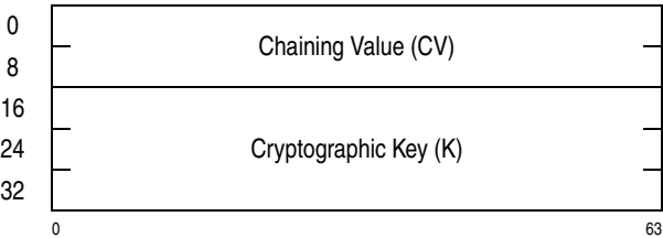
Figure 7-164. Parameter Block for KMO-AES-192
