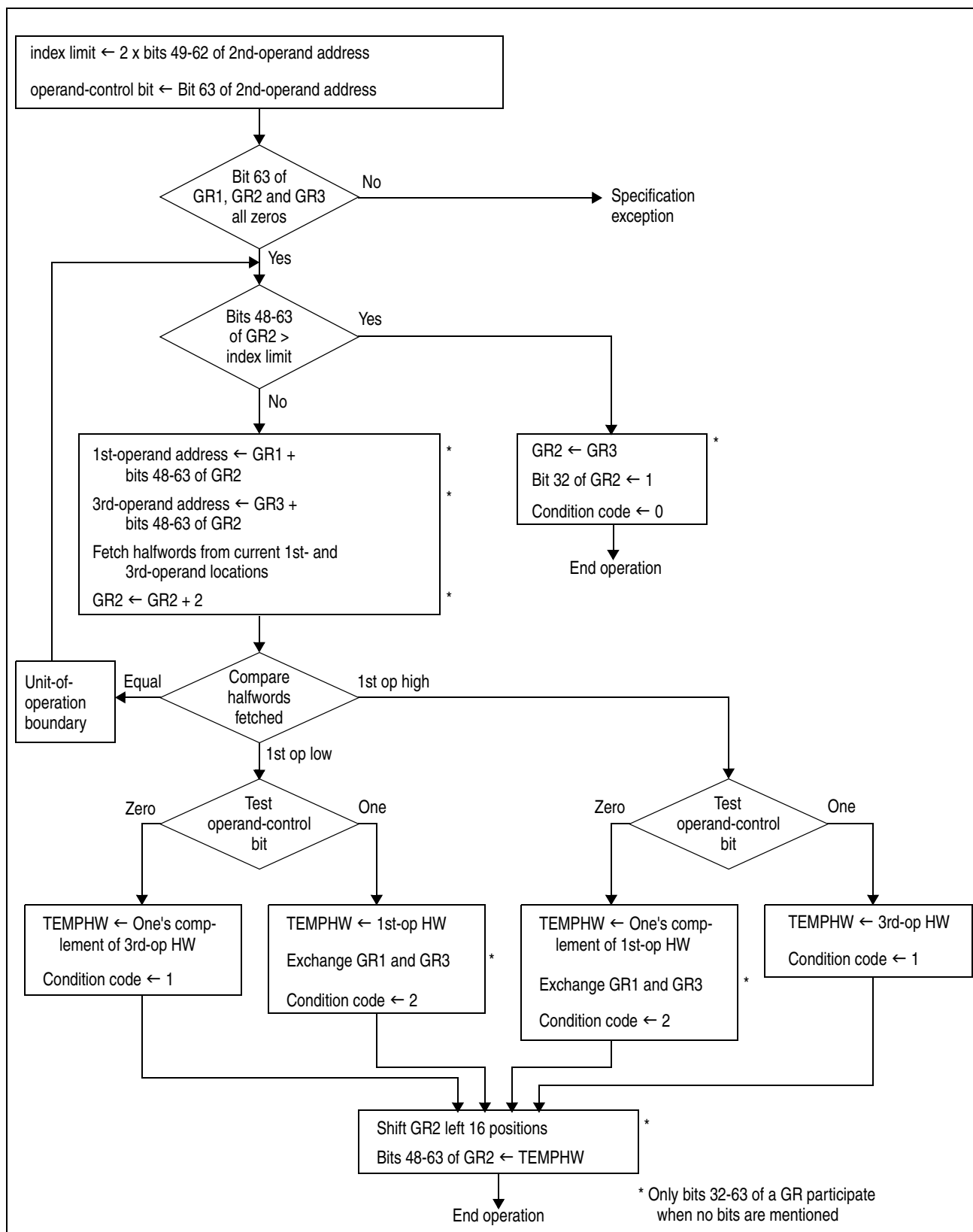
Figure 7-174. Execution of COMPARE AND FORM CODEWORD in the 24-Bit or 31-bit Addressing Mode
