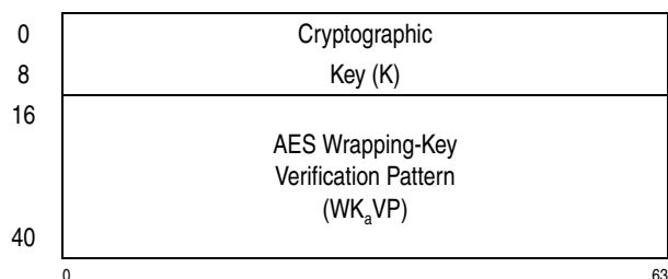
Figure 10-39. Parameter Block for PCKMO-Encrypt-AES-128-Key
