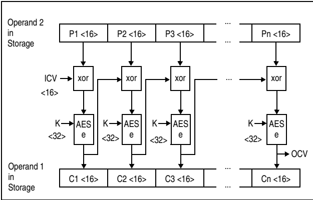
Figure 7-69. KMC AES Encipher Operation Using 256-Bit Key
