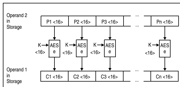
Figure 7-28. KM-AES Encipher Operation Using 128-Bit Key
