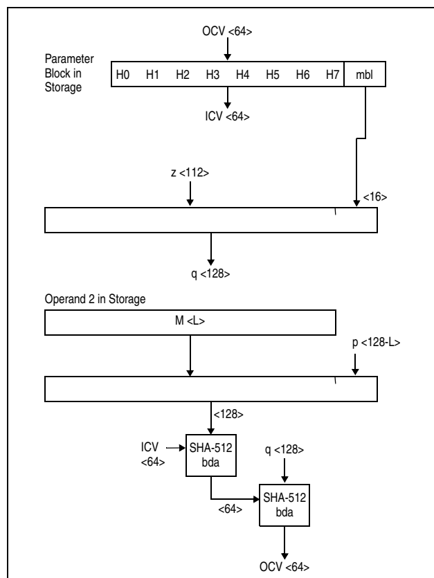
Figure 7-216. KLMD-SHA-512 Partial-Block Case 2 ( 112 \leq L \leq 127 )
