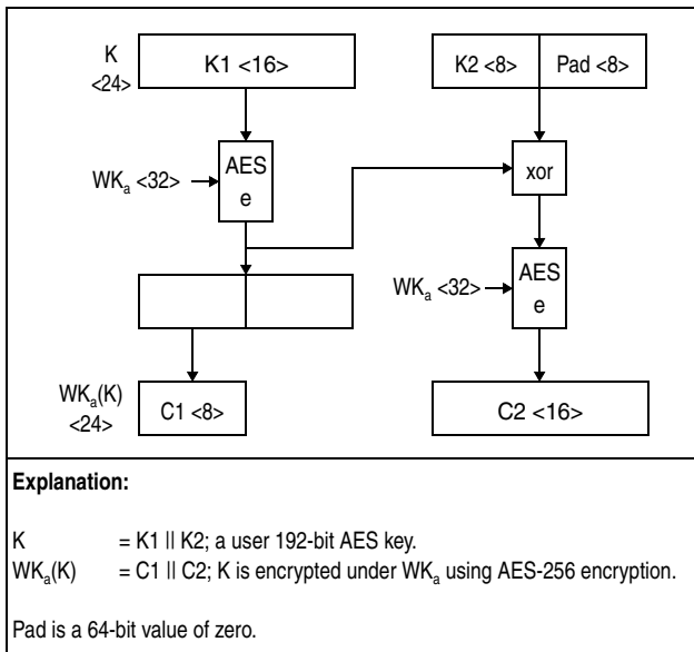
Figure 7-311. Encryption of 192-Bit AES Key Using WK_a
