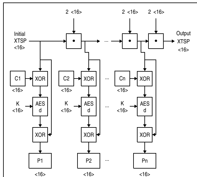
Figure 7-41. XTS-AES-128 Decipher Operation
