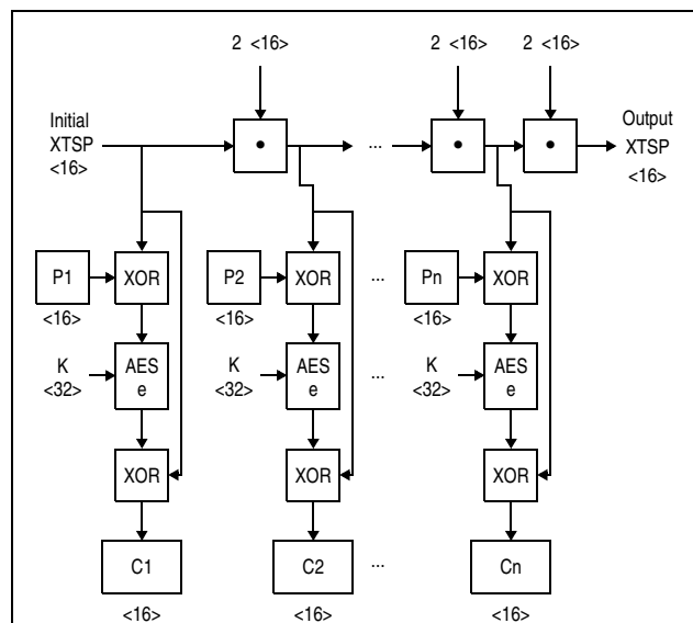
Figure 7-44. KM-XTS-AES-256 Encipher Operation
