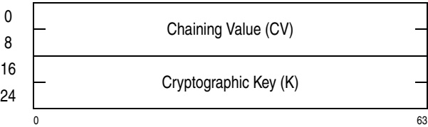
Figure 7-94. Parameter Block for KMF-AES-128
