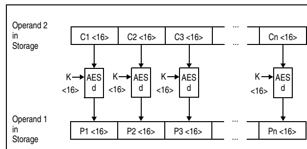
Figure 7-29. KM-AES Decipher Operation Using 128-Bit Key
