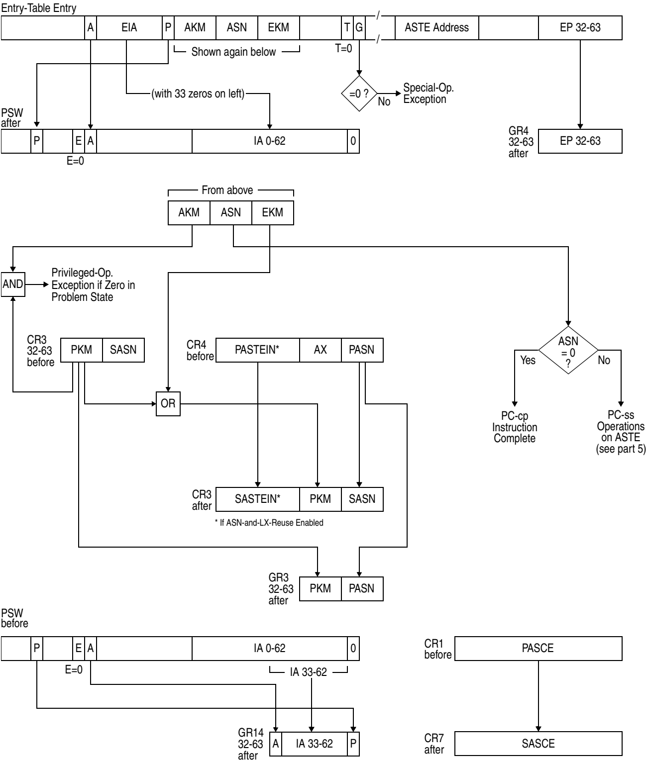
Figure 10-58. Execution of PROGRAM CALL (Part 1 of 5).
