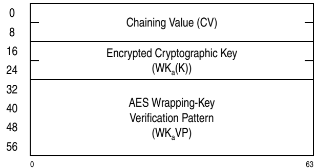
Figure 7-60. Parameter Block for KMC-Encrypted-AES-128
