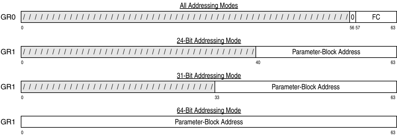
Figure 10-43. General Register Assignment for PERFORM TIMING FACILITY FUNCTION
