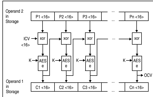
Figure 7-65. KMC AES Encipher Operation Using 192-Bit Key
