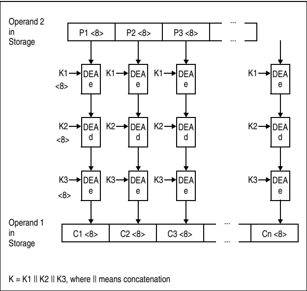
Figure 7-24. KM TDEA Encipher Operation Using 192-Bit Key
