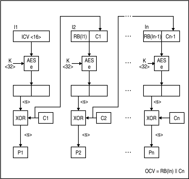
Figure 7-105. KMF-AES-256 Decipher Operation
