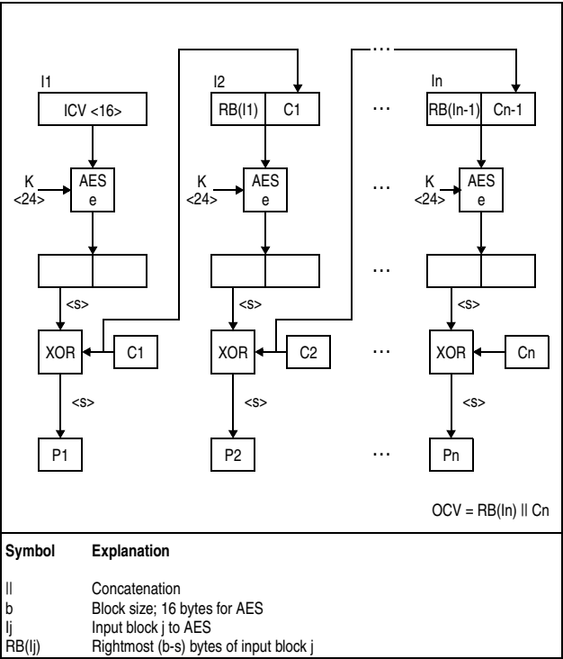
Figure 7-101. KMF-AES-192 Decipher Operation
