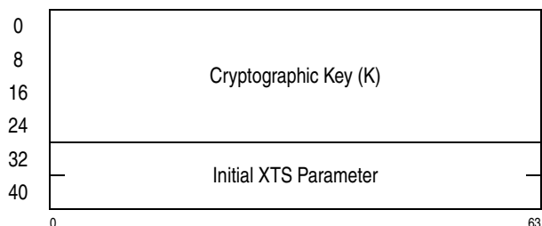
Figure 7-42. Parameter Block for KM-XTS-AES-256
