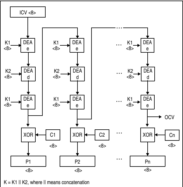
Figure 7-155. KMO-TDEA-128 Decipher Operation
