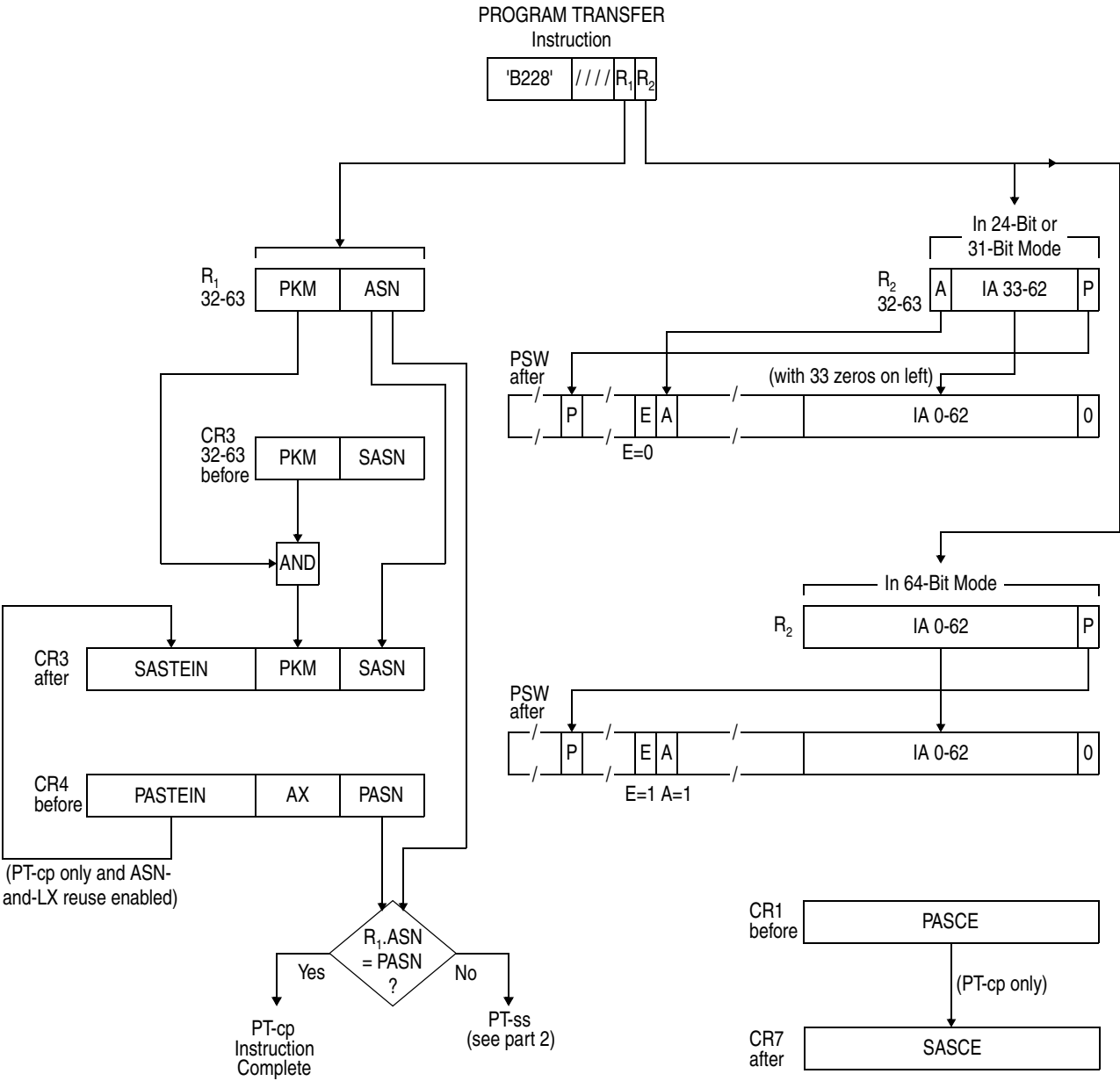
Figure 10-62. Execution of PROGRAM TRANSFER (Part 1 of 2).
