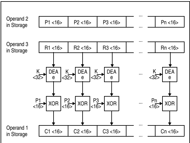
Figure 7-137. KMCTR AES Encipher Operation Using 256-Bit Key
