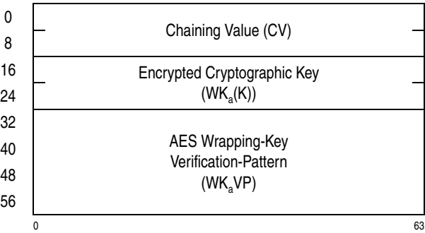
Figure 7-95. Parameter Block for KMF-Encrypted-AES-128
