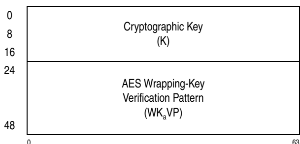
Figure 10-40. Parameter Block for PCKMO-Encrypt-AES-192-Key
