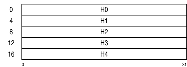
Figure 7-193. Parameter Block for KIMD-SHA-1
