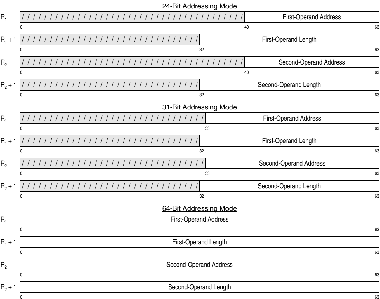
Figure 7-250. Register Contents for CONVERT UTF-8 TO UTF32
