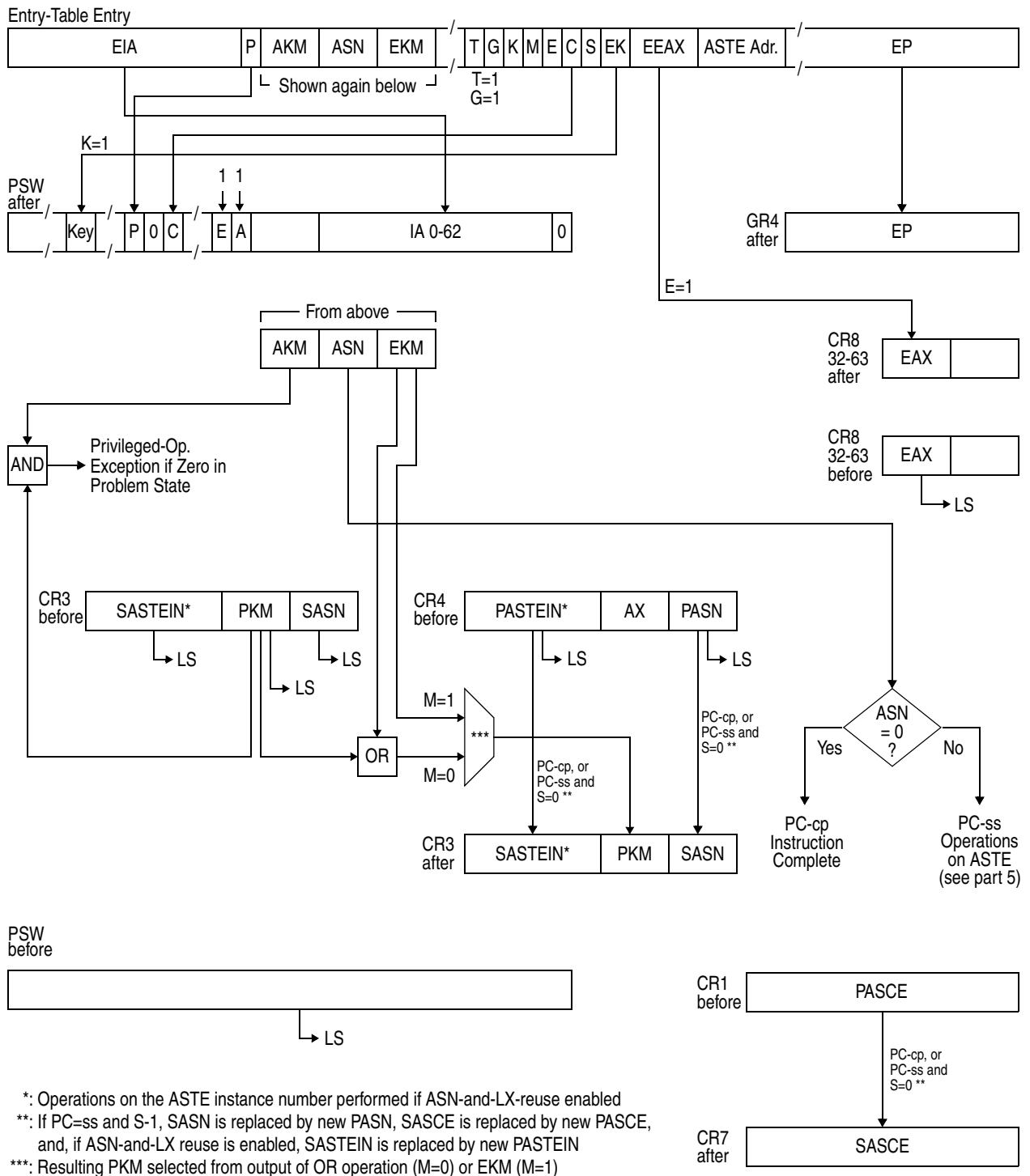
Figure 10-58. Execution of PROGRAM CALL (Part 3 of 5).
