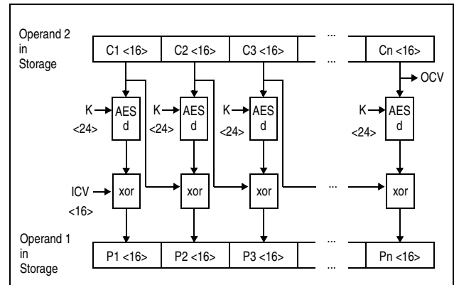
Figure 7-66. KMC AES Decipher Operation Using 192-Bit Key
