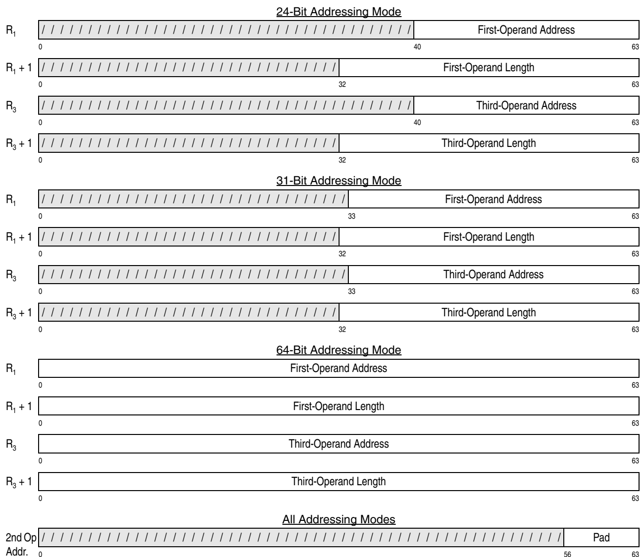
Figure 7-253. Register Contents and Second-Operand Address for MOVE LONG EXTENDED
