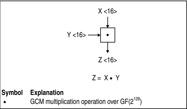
Figure 7-191. Symbol For GCM Multiplication Operation Over GF(2^{128})
