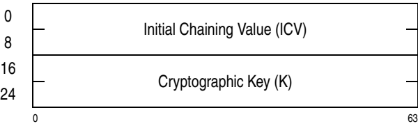
Figure 7-235. Parameter Block for KMAC-AES-128
