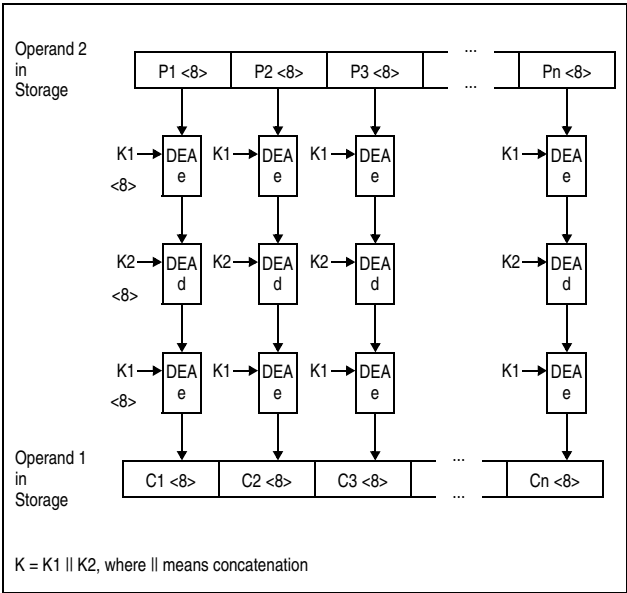
Figure 7-20. KM-TDEA Encipher Operation Using 128-Bit Key
