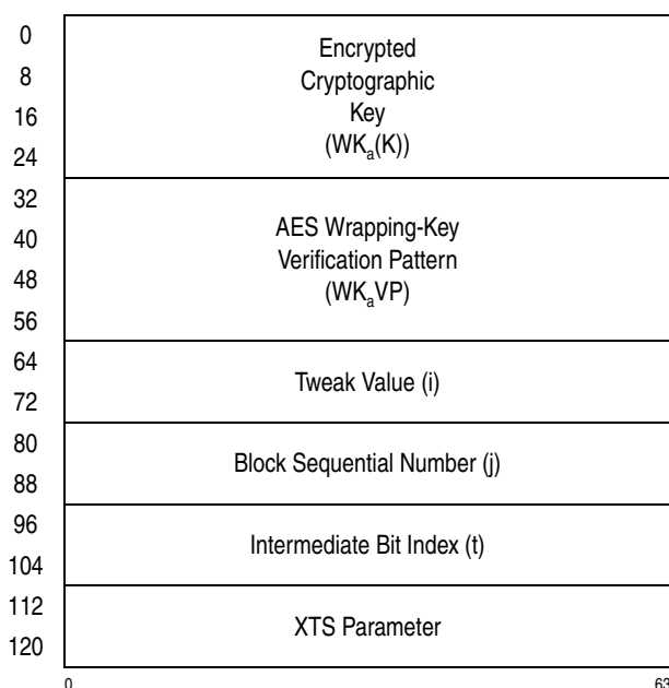
Figure 7-287. Parameter Block for PCC-Compute-XTS-Parameter-Using-Encrypted-AES-256
