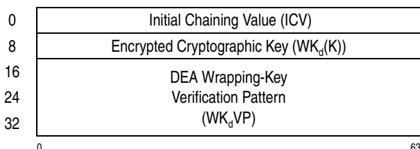
Figure 7-227. Parameter Block for KMAC-Encrypted-DEA
