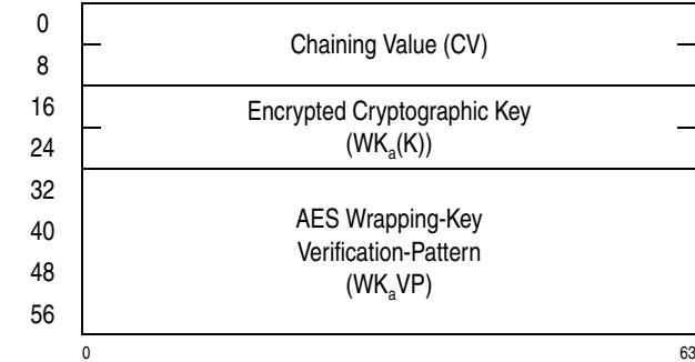
Figure 7-161. Parameter Block for KMO-Encrypted-AES-128
