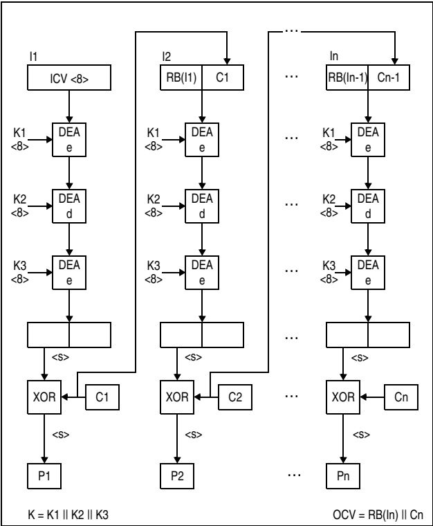
Figure 7-93. KMF-TDEA-192 Decipher Operation
