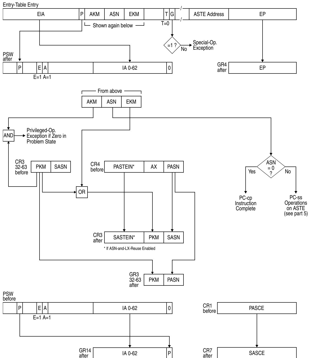
Figure 10-58. Execution of PROGRAM CALL (Part 2 of 5).
