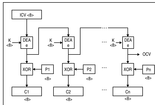
Figure 7-150. KMO-DEA Encipher Operation
