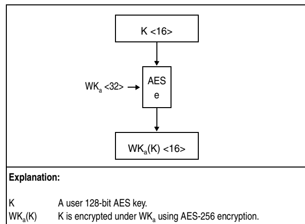
Figure 7-309. Encryption of 128-Bit AES Key Using WK_a
