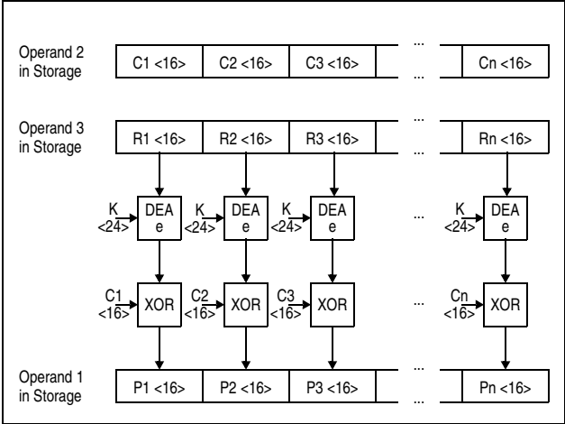
Figure 7-134. KMCTR AES Decipher Operation Using 192-Bit Key
