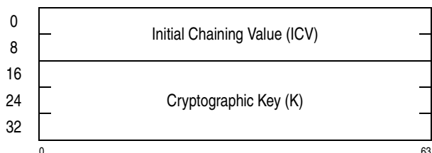
Figure 7-238. Parameter Block for KMAC-AES-192
