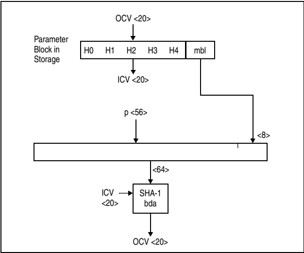
Figure 7-204. KLMD-SHA-1 Empty Block ( L = 0 )
