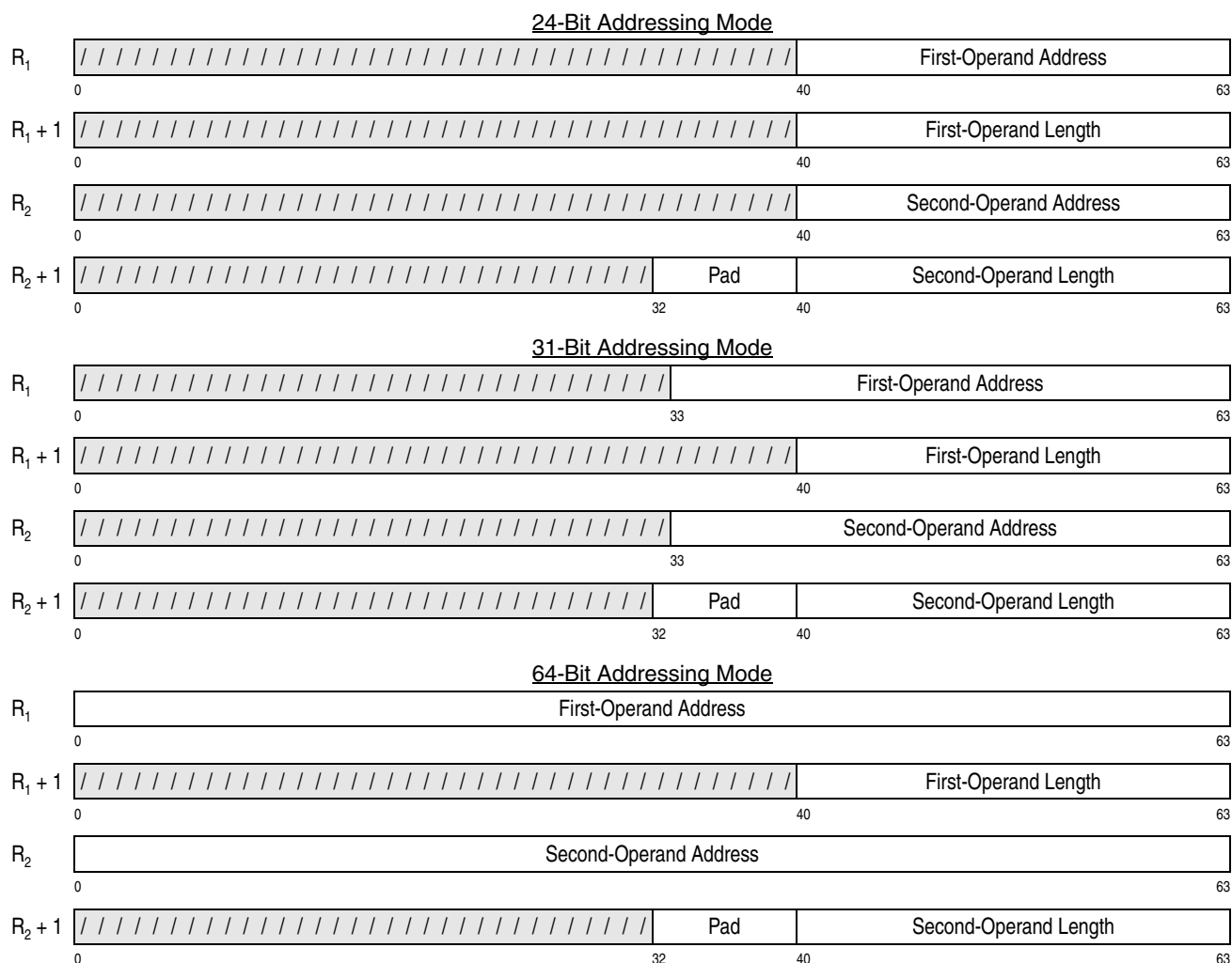
Figure 7-252. Register Contents for MOVE LONG
