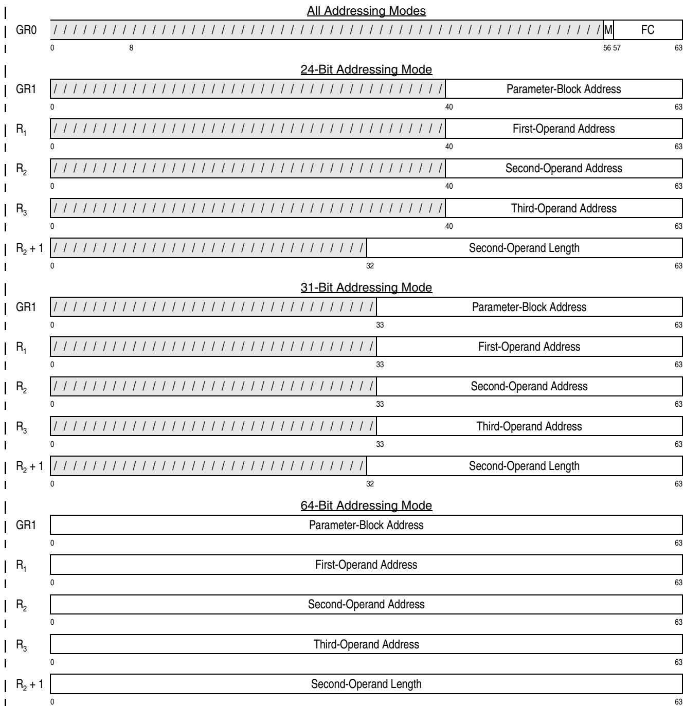
Figure 7-108. General Register Assignment for KMCTR
