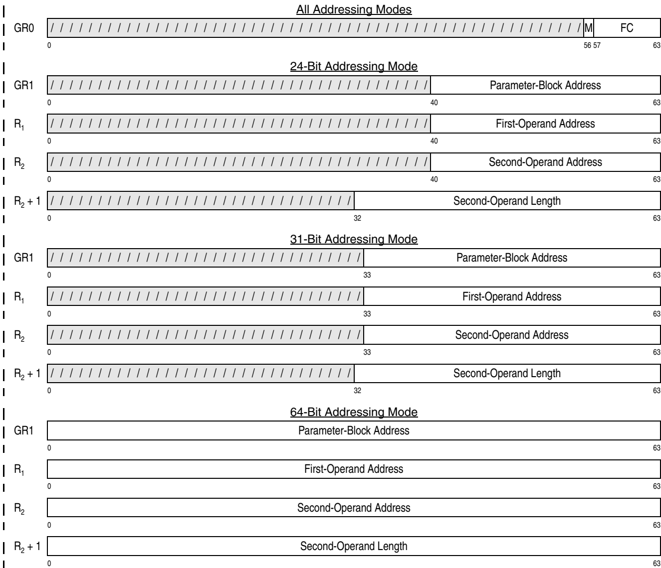
Figure 7-141. General Register Assignment for KMO
