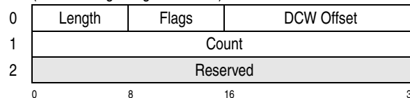
Figure 15-18. Transport-Status Header (TSH)
