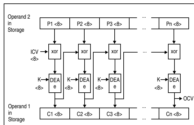
Figure 7-49. KMC DEA Encipher Operation Using 64-Bit Key
