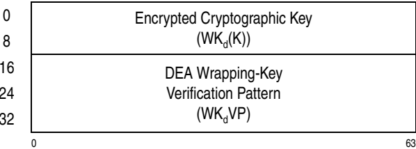
Figure 7-19. Parameter Block for KM-Encrypted-TDEA-128
