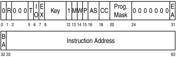
Figure 4-3. ESA/390 PSW Format, Except Bit 31 Shown as EA
