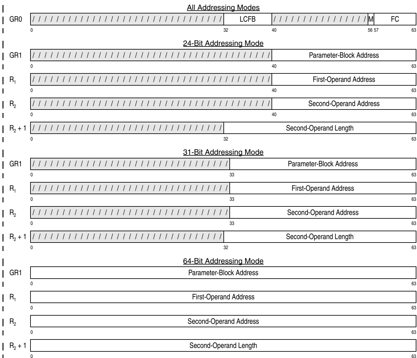
Figure 7-75. General Register Assignment for KMF
