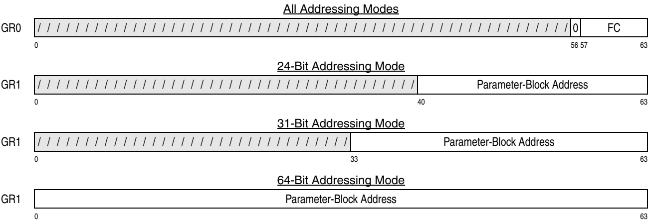
Figure 10-34. General Register Assignment for PCKMO
