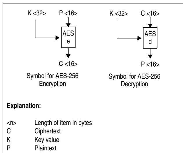
Figure 7-306. Symbols for AES-256 Encryption and Decryption
