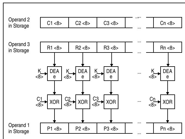
Figure 7-118. KMCTR DEA Decipher Operation Using 64-Bit Key
