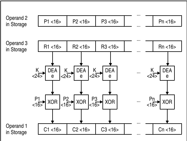
Figure 7-133. KMCTR AES Encipher Operation Using 192-Bit Key
