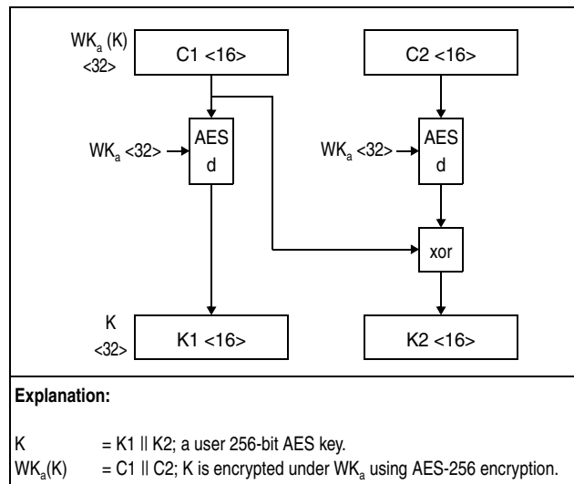
Figure 7-314. Decryption of 256-Bit AES Key Using WK_a
