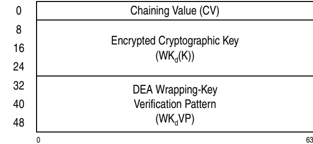
Figure 7-56. Parameter Block for KMC-Encrypted-TDEA-192
