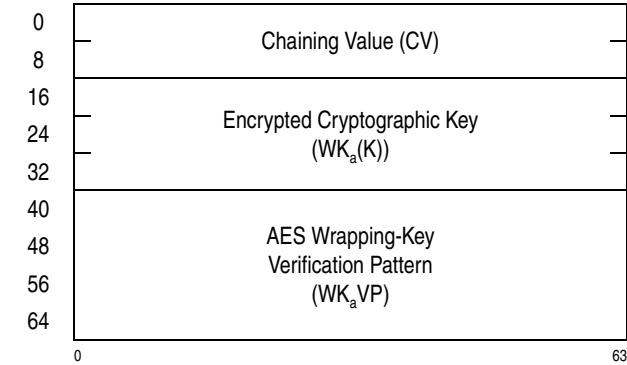
Figure 7-99. Parameter Block for KMF-Encrypted-AES-192
