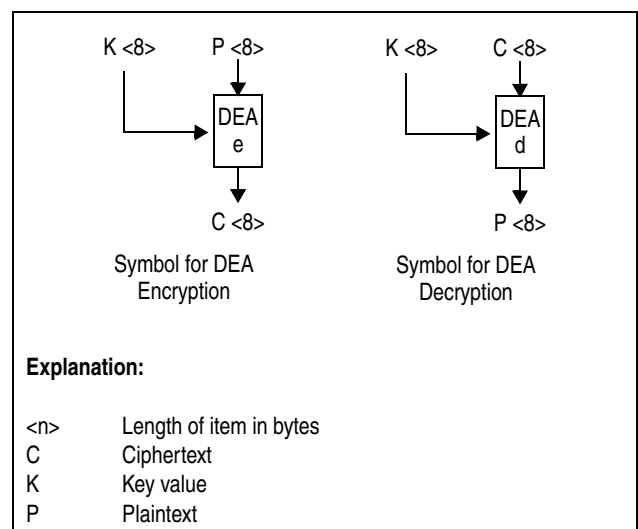
Figure 7-305. Symbols for DEA Encryption and Decryption
