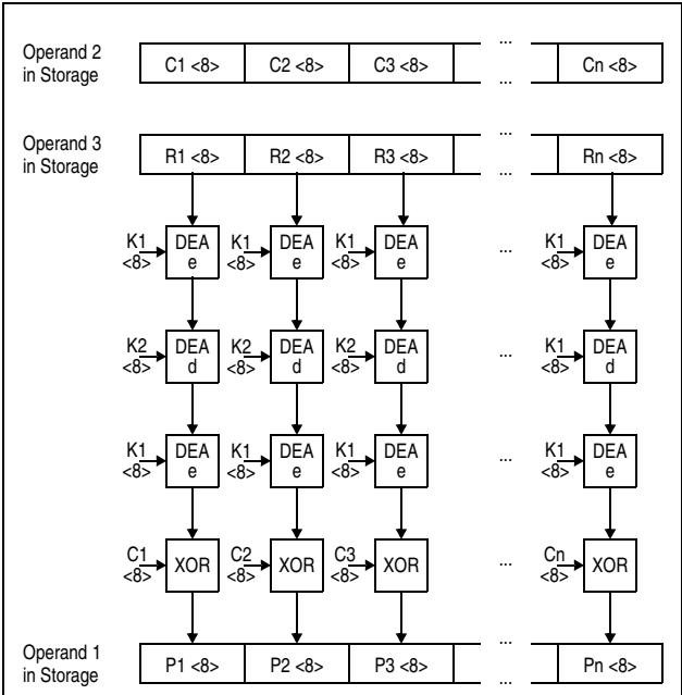
Figure 7-122. KMCTR TDEA DEcipher Operation Using 128-Bit Key
