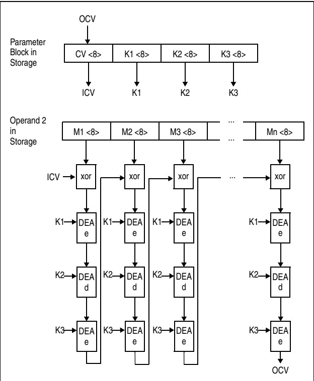
Figure 7-234. MAC Computation Using 192-bit TDEA Key
