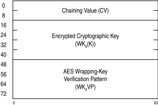
Figure 7-169. Parameter Block for KMO-AES-256
