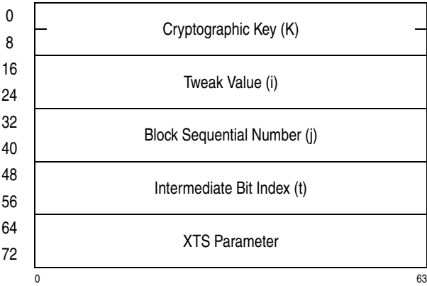
Figure 7-283. Parameter Block for PCC-Compute-XTS-Parameter-Using-AES-128
