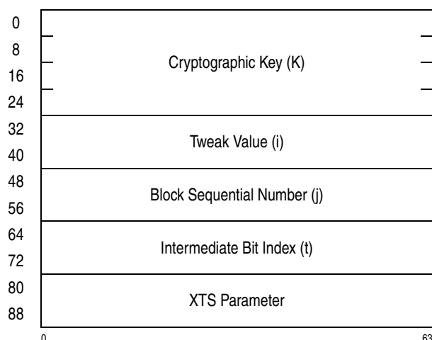
Figure 7-286. Parameter Block for PCC-Compute-XTS-Parameter-Using-AES-256
