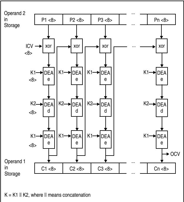
Figure 7-53. KMC TDEA Encipher Operation Using 128-Bit Key
