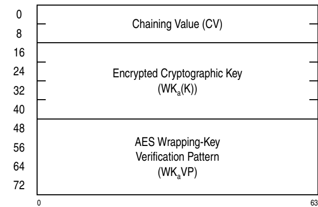
Figure 7-103. Parameter Block for KMF-AES-256
