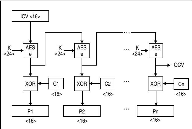
Figure 7-167. KMO-AES-192 Decipher Operation
