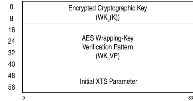
Figure 7-39. Parameter Block for KM-XTS-Encrypted-AES-128
