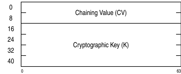
Figure 7-102. Parameter Block for KMF-AES-256
