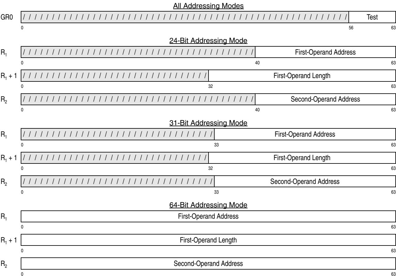
Figure 7-299. Register Contents for TRANSLATE EXTENDED
