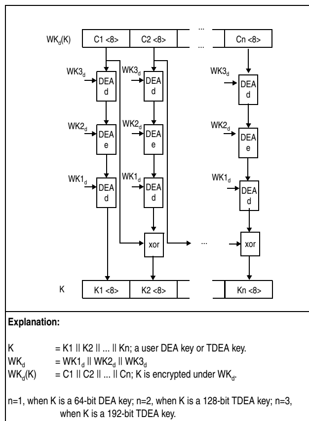
Figure 7-308. Decryption of DES or TDES Key Using WK_d
