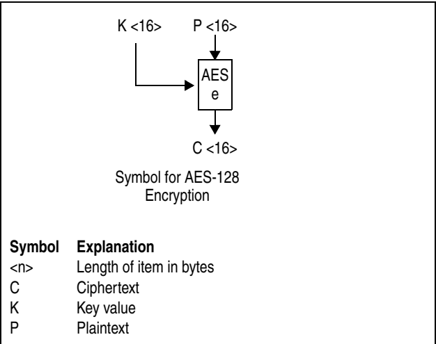
Figure 7-111. Symbols for AES-128 Encryption
