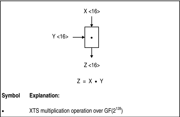
Figure 7-8. Symbol For XTS Multiplication Operation Over GF(2^{128})
