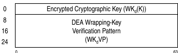
Figure 7-116. Parameter Block for KMCTR-Encrypted-DEA
