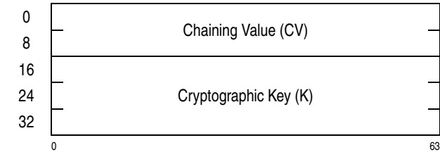
Figure 7-98. Parameter Block for KMF-AES-192
