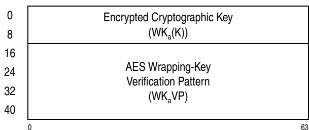
Figure 7-27. Parameter Block for KM-Encrypted-AES-128
