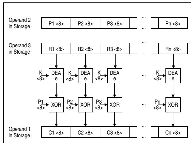
Figure 7-117. KMCTR DEA Encipher Operation Using 64-Bit Key
