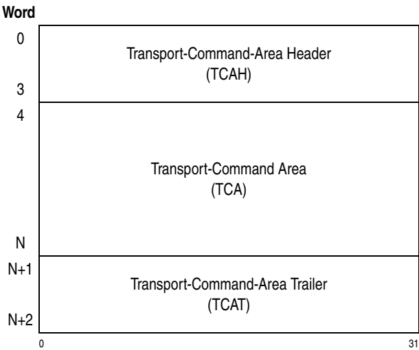
Figure 15-8. Transport-Command-Control Block (TCCB)
