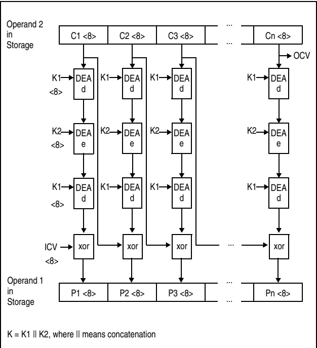
Figure 7-54. KMC TDEA Decipher Operation Using 128-Bit Key
