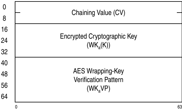
Figure 7-64. Parameter Block for KMC-Encrypted-AES-192
