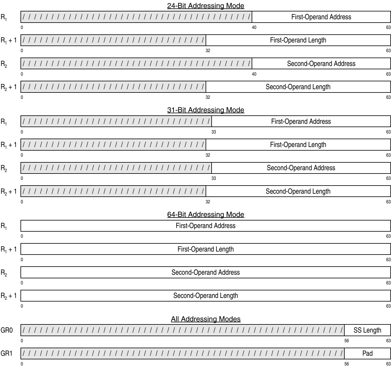
Figure 7-181. Register Contents and Second-Operand Address for COMPARE UNTIL SUBSTRING EQUAL
