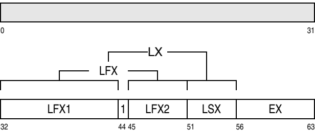
Second-Operand Address when ASN-and-LX Reuse Is Enabled and Bit 44 Is One
