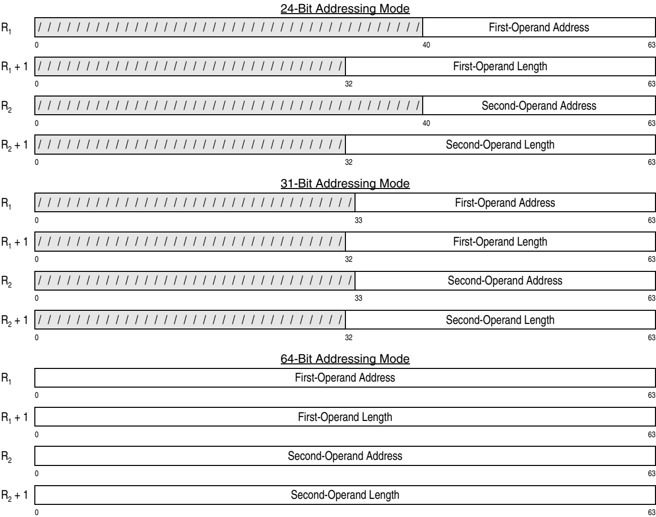
Figure 7-248. Register Contents for CONVERT UTF-32 TO UTF-8
