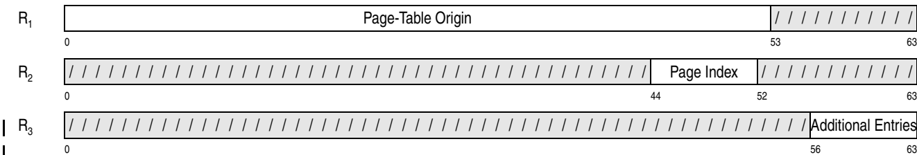
Figure 10-15. Register Contents for INVALIDATE PAGE TABLE ENTRY
