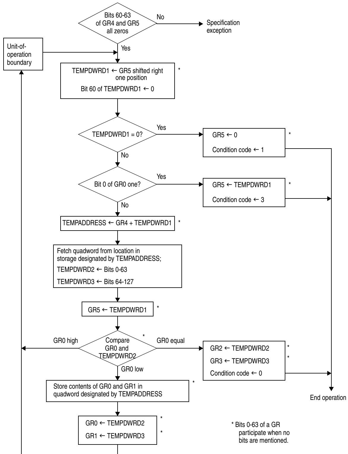
Figure 7-302. Execution of UPDATE TREE in the 64-Bit Addressing Mode
