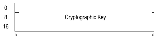
Figure 7-30. Parameter Block for KM-AES-192
