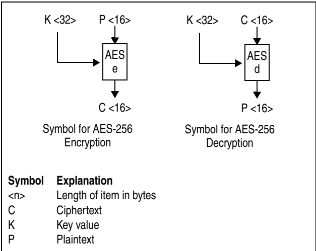
Figure 7-12. Symbols for AES-256 Encryption and Decryption
