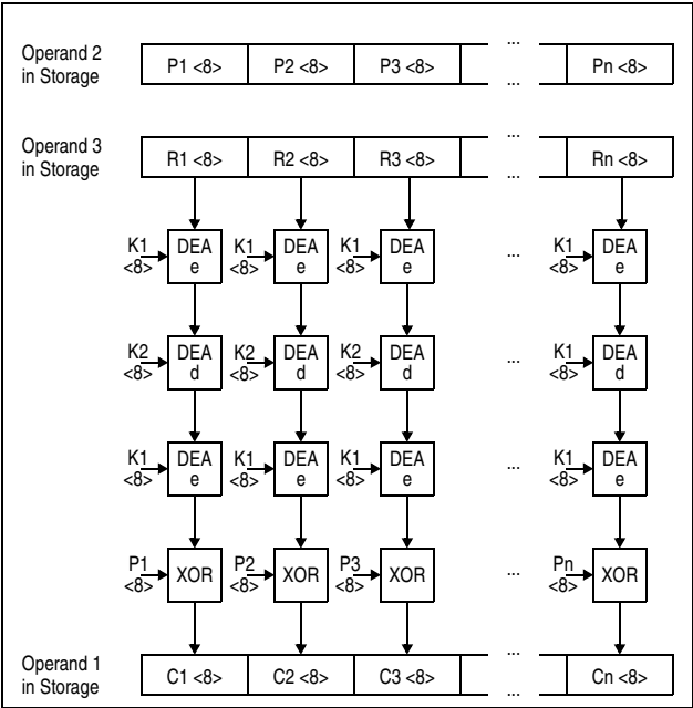
Figure 7-121. KMCTR TDEA Encipher Operation Using 128-Bit Key
