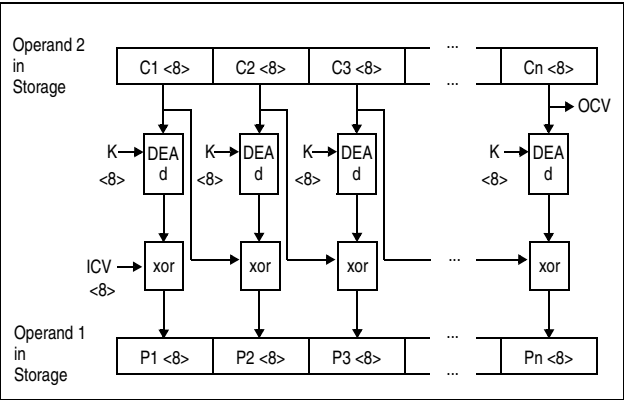
Figure 7-50. KMC DEA Decipher Operation Using 64-Bit Key
