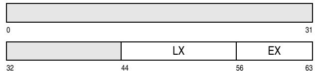
Effective Address when ASN-and-LX Reuse Is Not Enabled
