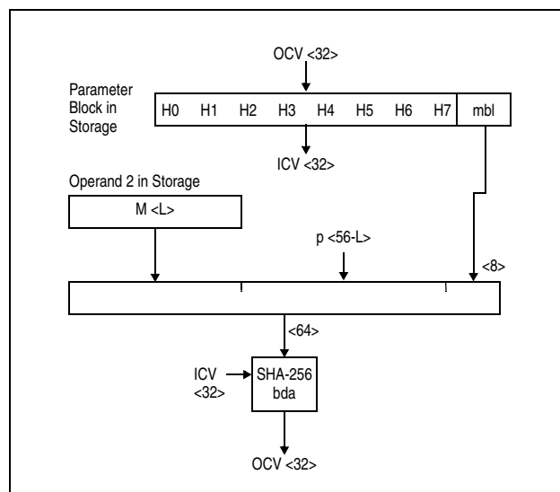
Figure 7-210. KLMD-SHA-256 Partial-Block Case 1 ( 1 \leq L \leq 55 )
