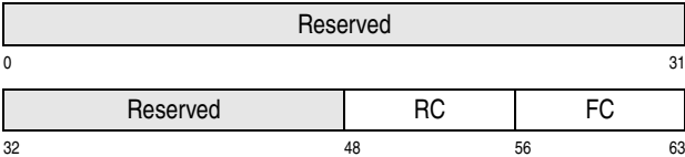
Figure 10-56. General-Register R_1 Format
