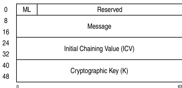
Figure 7-274. Parameter Block for PCC-Compute-Last-Block-CMAC-Using-AES-128
