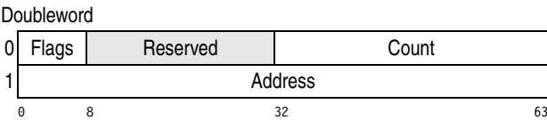
Figure 15-26. Transport-Indirect-Data-Address Word (TIDAW)
