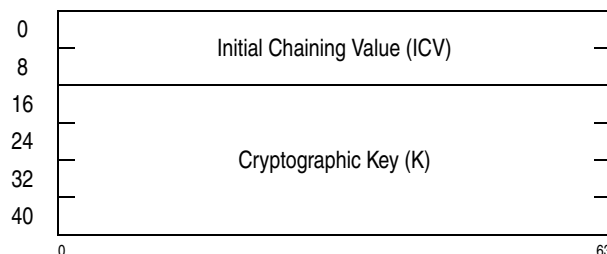
Figure 7-241. Parameter Block for KMAC-AES-256
