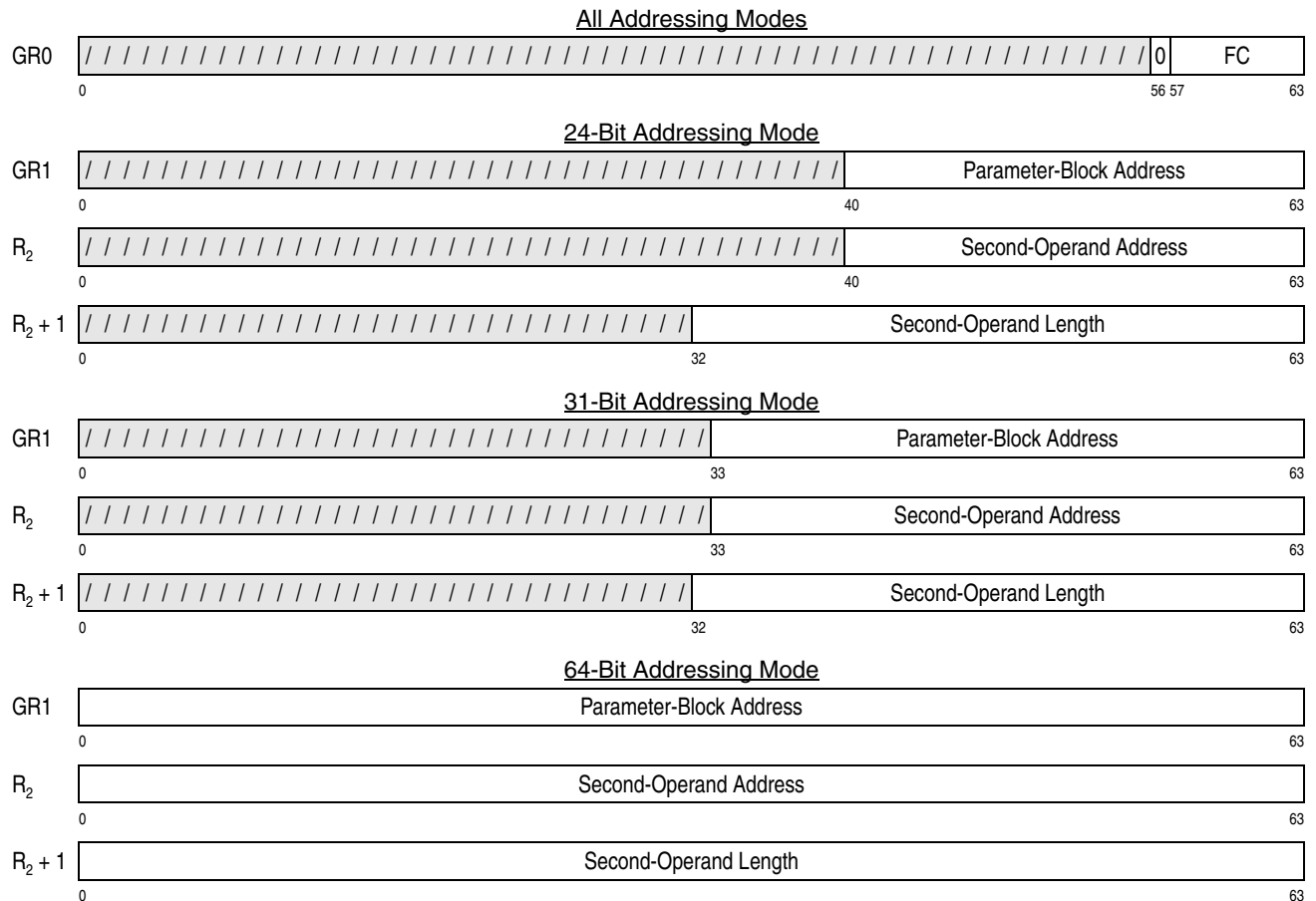
Figure 7-187. General Register Assignment for KIMD and KLMD
