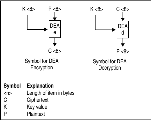
Figure 7-143. Symbols for DEA Encryption and Decryption
