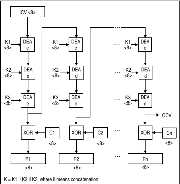
Figure 7-159. KMO-TDEA-192 Decipher Operation
