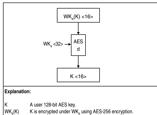
Figure 7-310. Decryption of 128-Bit AES Key Using WK_a
