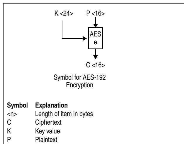
Figure 7-223. Symbols for AES-192 Encryption
