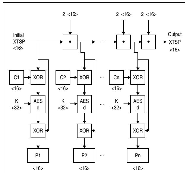
Figure 7-45. XTS-AES-128 Decipher Operation
