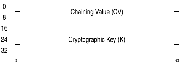
Figure 7-63. Parameter Block for KMC-AES-192
