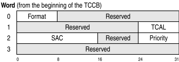
Figure 15-9. Transport-Command-Area Header (TCAH)
