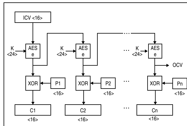
Figure 7-166. KMO-AES-192 Encipher Operation
