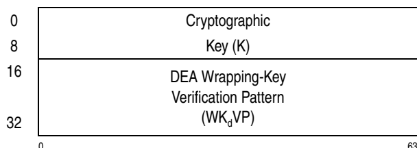
Figure 10-37. Parameter Block for PCKMO-Encrypt-TDEA-128-Key
