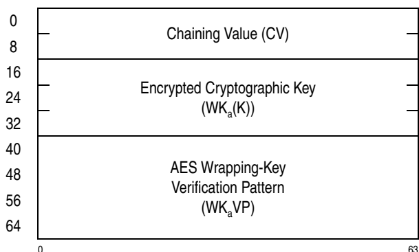
Figure 7-165. Parameter Block for KMO-Encrypted-AES-192
