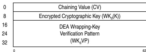
Figure 7-83. Parameter Block for KMF-Encrypted-DEA
