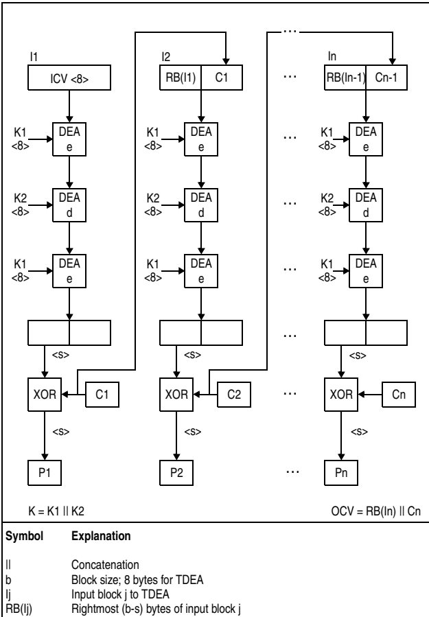
Figure 7-89. KMF-TDEA-128 Decipher Operation
