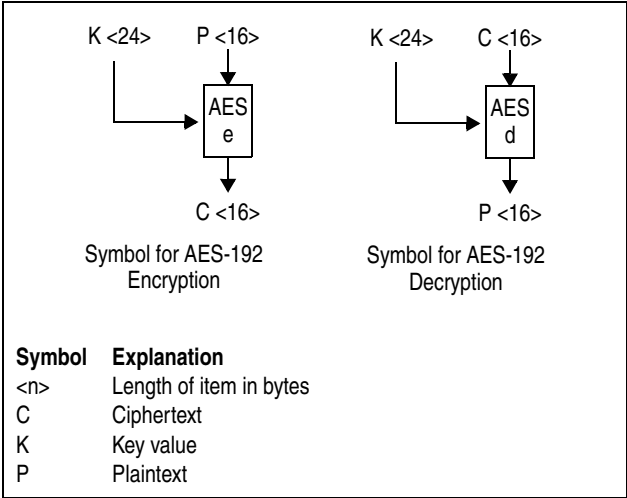
Figure 7-11. Symbols for AES-192 Encryption and Decryption
