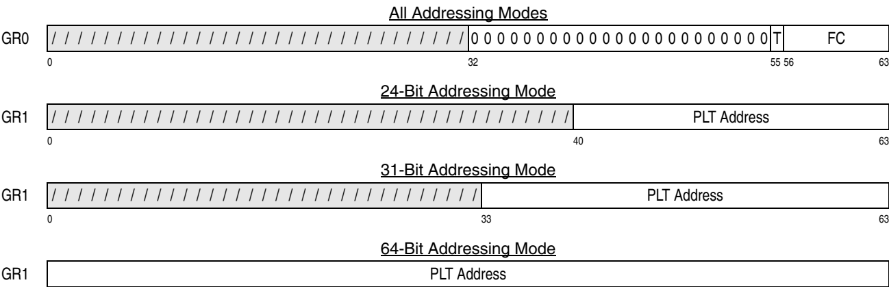
Figure 7-291. General Register Assignment for PLO
