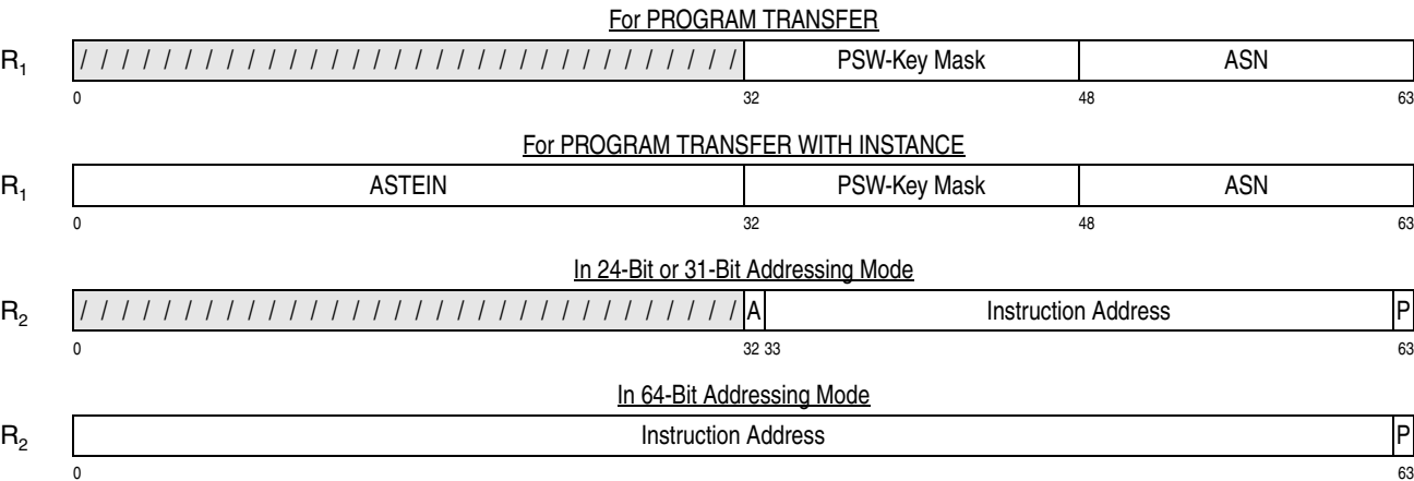
Figure 10-60. Register Contents for PROGRAM TRANSFER (WITH INSTANCE)
