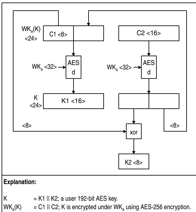
Figure 7-312. Decryption of 192-Bit AES Key Using WK_a
