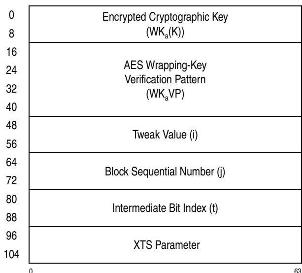
Figure 7-284. Parameter Block for PCC-Compute-XTS-Parameter-Using-Encrypted-AES-128
