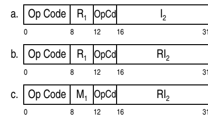
Figure 5-1. Basic Instruction Formats (Part 1 of 4)
