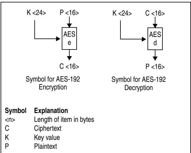
Figure 7-262. Symbols for AES-192 Encryption and Decryption
