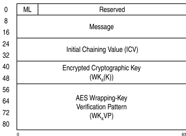
Figure 7-275. Parameter Block for PCC-Compute-Last-Block-CMAC-Using-Encrypted-AES-128
