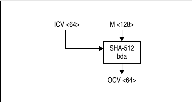
Figure 7-190. Symbol for SHA-512 Block Digest Algorithm
