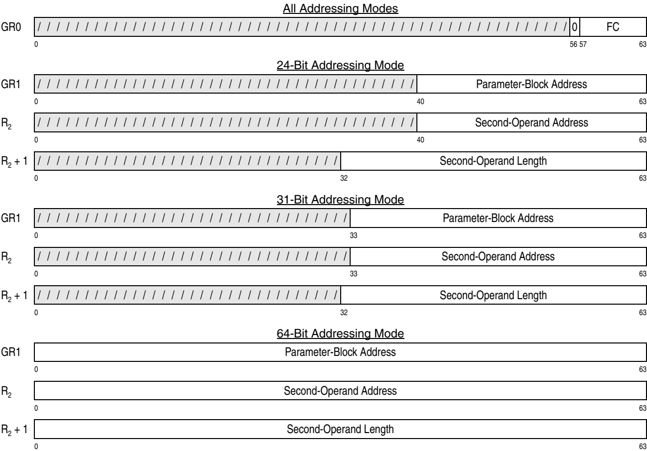
Figure 7-219. General Register Assignment for KMAC
