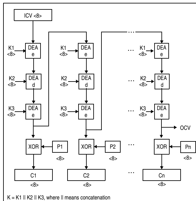
Figure 7-158. KMO-TDEA-192 Encipher Operation
