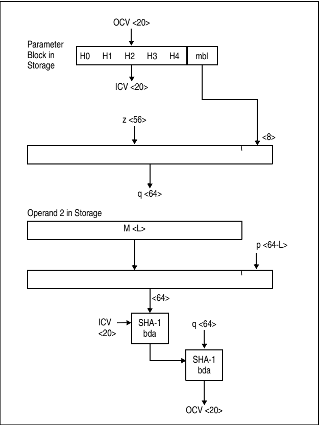
Figure 7-206. KLMD-SHA-1 Partial-Block Case 2 ( 56 \leq L \leq 63 )
