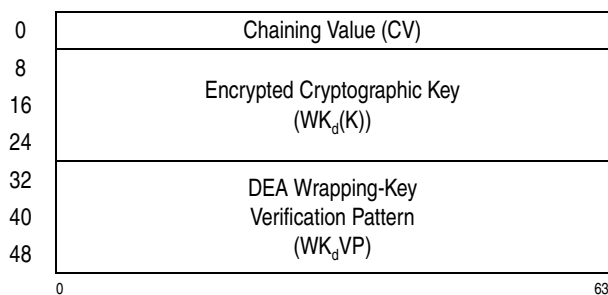
Figure 7-157. Parameter Block for KMO-Encrypted-TDEA-192
