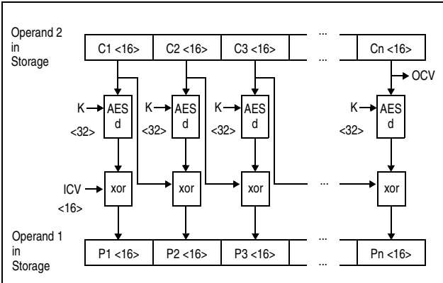
Figure 7-70. KMC AES Decipher Operation Using 256-Bit Key
