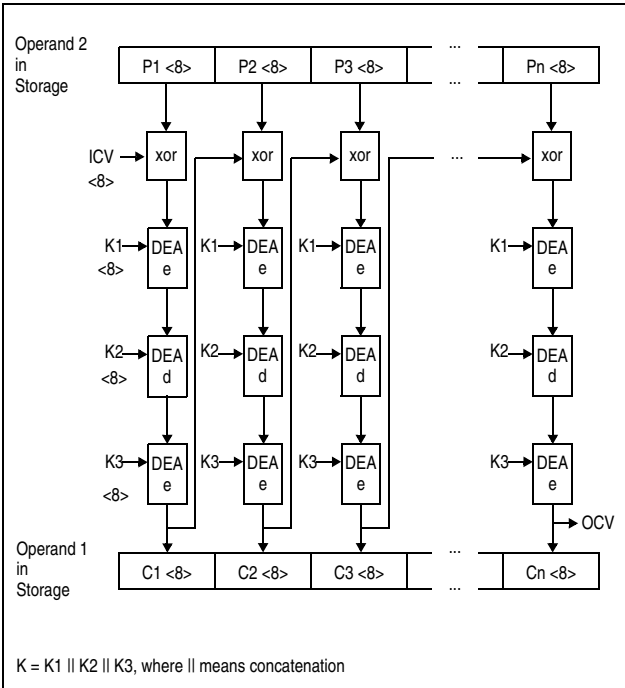
Figure 7-57. KMC TDEA Encipher Operation Using 192-Bit Key
