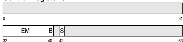
Control Register 9
