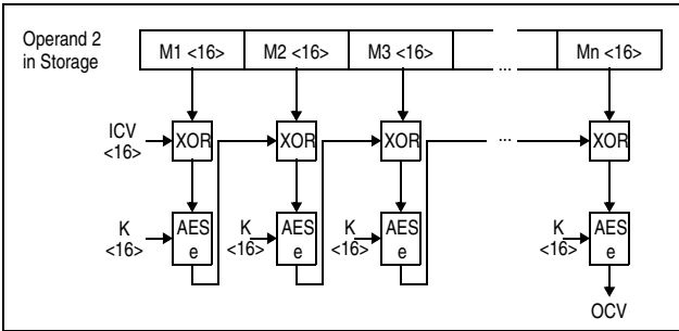
Figure 7-237. KMAC-AES-128
