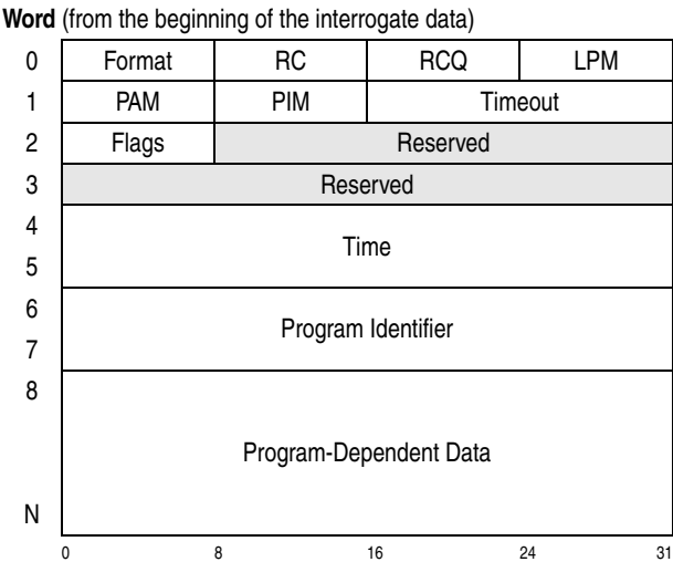
Figure 15-16. Interrogate Data
