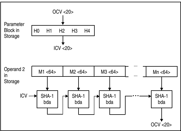
Figure 7-194. KIMD-SHA-1
