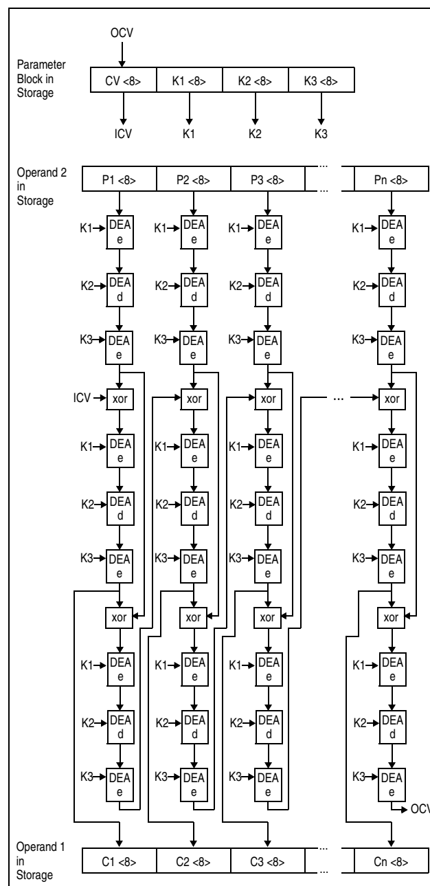
Figure 7-72. KMC-PRNG
