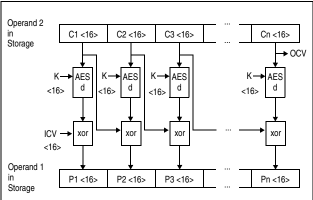
Figure 7-62. KMC AES Decipher Operation Using 128-Bit Key
