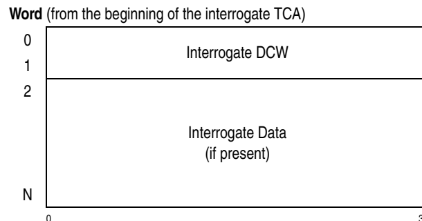
Figure 15-15. Interrogate Transport-Command Area (TCA)
