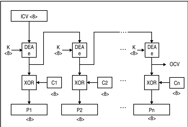
Figure 7-151. KMO-DEA Decipher Operation
