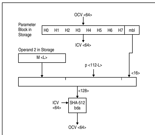
Figure 7-215. KLMD-SHA-512 Partial-Block Case 1 ( 1 \leq L \leq 111 )
