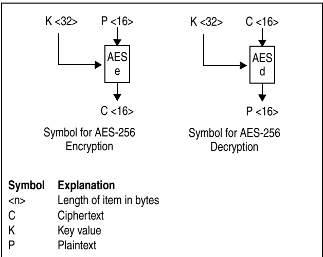
Figure 7-263. Symbols for AES-256 Encryption and Decryption
