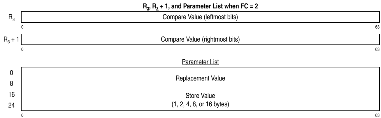
Figure 7-177. Register Contents for COMPARE AND SWAP AND STORE
