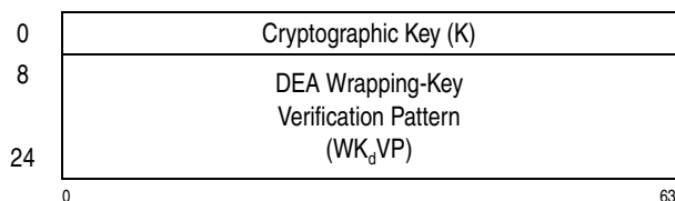
Figure 10-36. Parameter Block for PCKMO-Encrypt-DEA-Key
