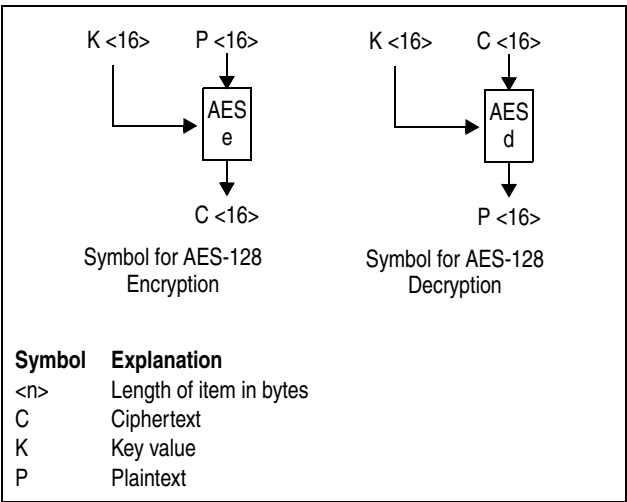
Figure 7-261. Symbols for AES-128 Encryption and Decryption
