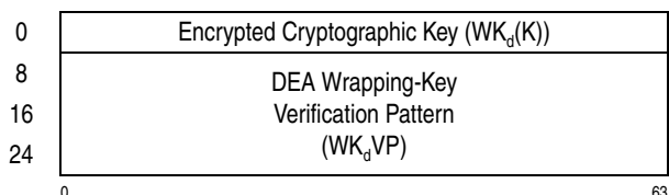
Figure 7-15. Parameter Block for KM-Encrypted-DEA
