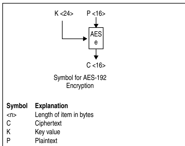
Figure 7-79. Symbols for AES-192 Encryption
