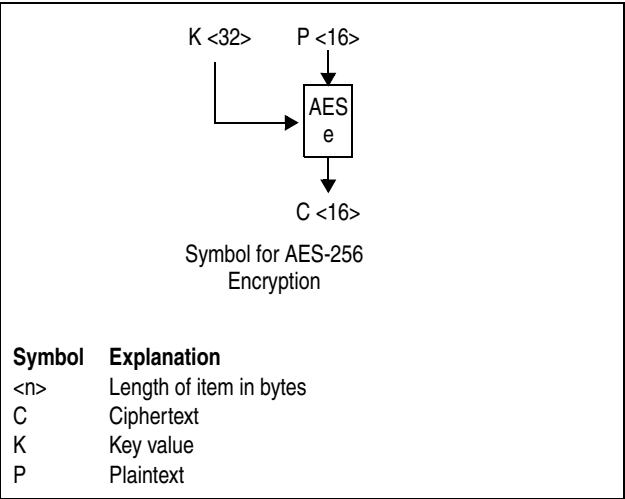
Figure 7-146. Symbols for AES-256 Encryption
