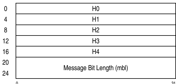
Figure 7-202. Parameter Block for KLMD-SHA-1
