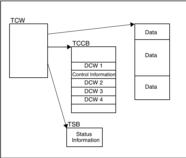
Figure 2. Example of TCW Channel Program Example Designating I/O
