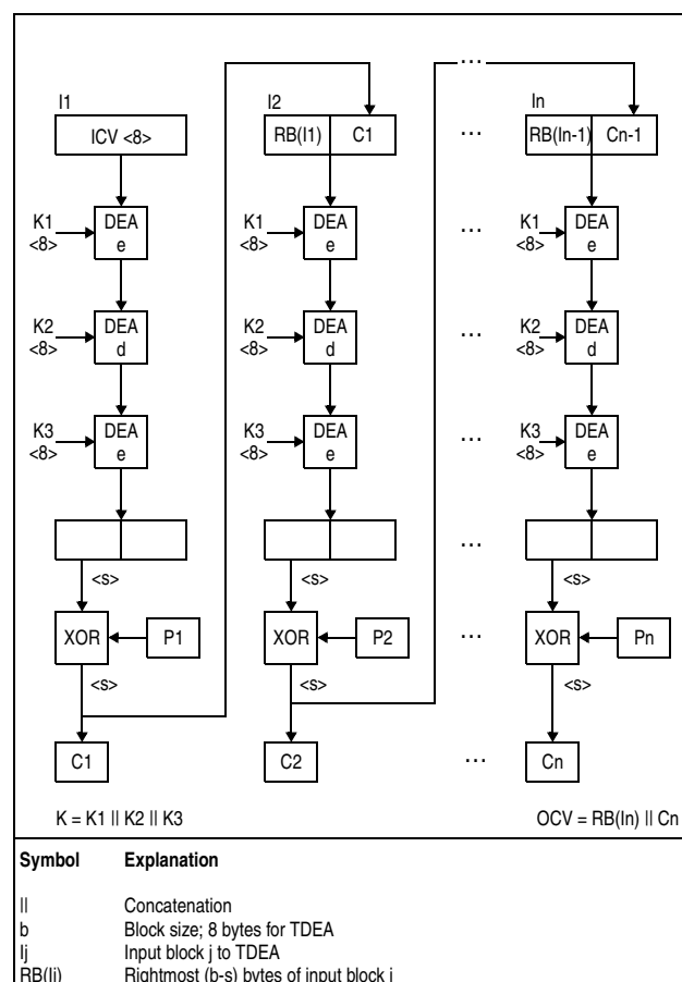
Figure 7-92. KMF-TDEA-192 Encipher Operation
