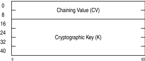
Figure 7-168. Parameter Block for KMO-AES-256
