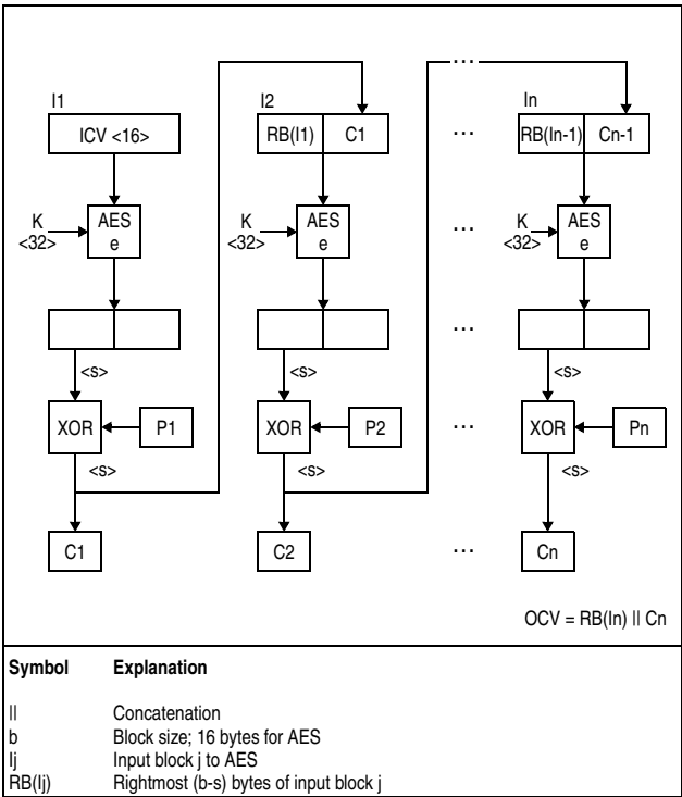
Figure 7-104. KMF-AES-256 Encipher Operation
