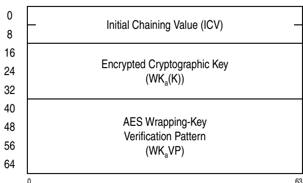
Figure 7-239. Parameter Block for KMAC-Encrypted-AES-192
