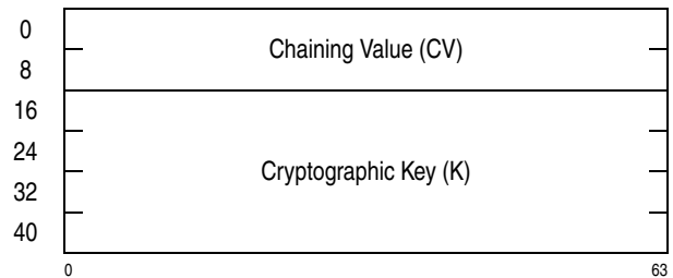
Figure 7-67. Parameter Block for KMC-AES-256
