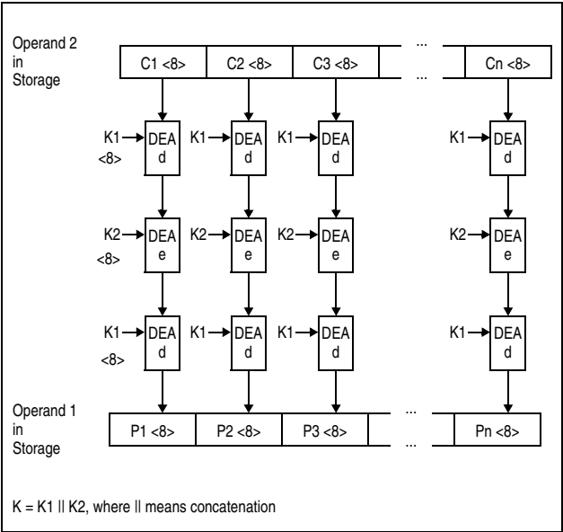
Figure 7-21. KM TDEA Decipher Operation Using 128-Bit Key
