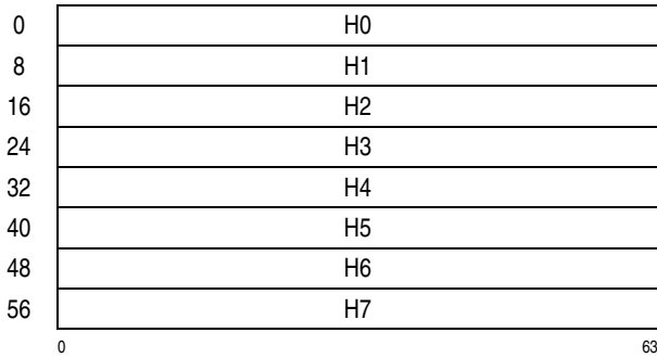
Figure 7-197. Parameter Block for KIMD-SHA-512
