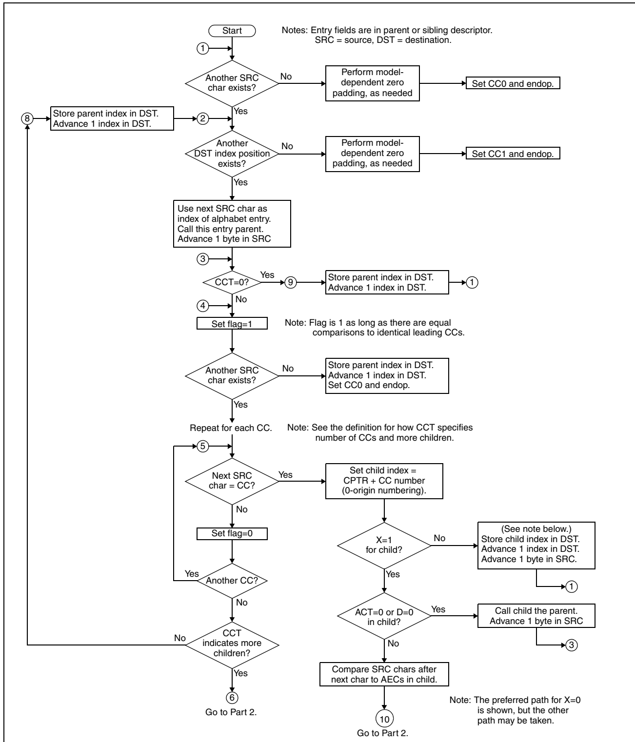
Figure 7-183. Compression Process (Part 1 of 2)
