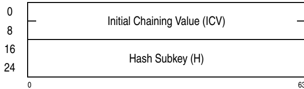
Figure 7-199. Parameter Block for KIMD-GHASH
