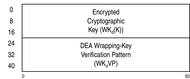
Figure 7-124. Parameter Block for KMCTR-Encrypted-TDEA-192
