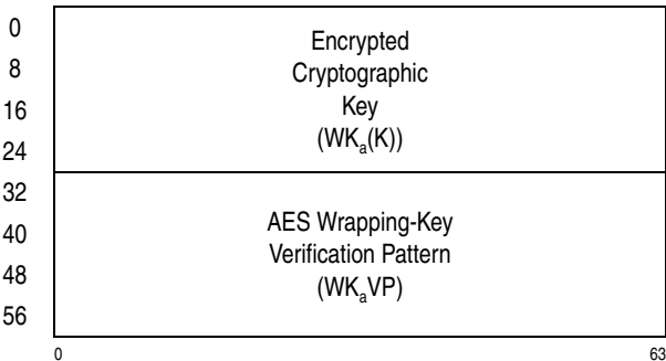
Figure 7-35. Parameter Block for KM-Encrypted-AES-256
