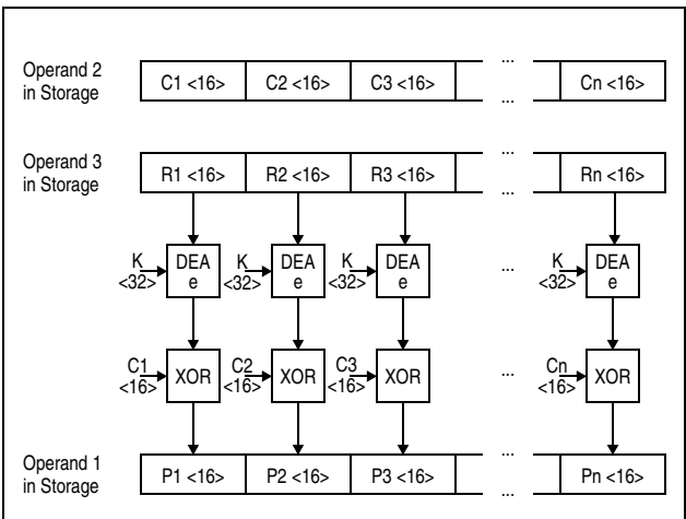
Figure 7-138. KMCTR AES Decipher Operation Using 256-Bit Key
