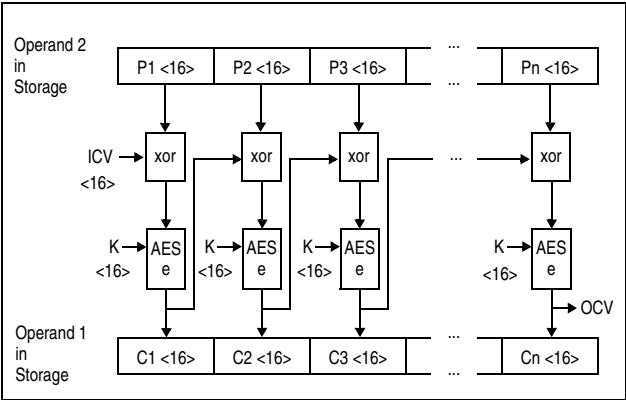
Figure 7-61. KMC AES Encipher Operation Using 128-Bit Key
