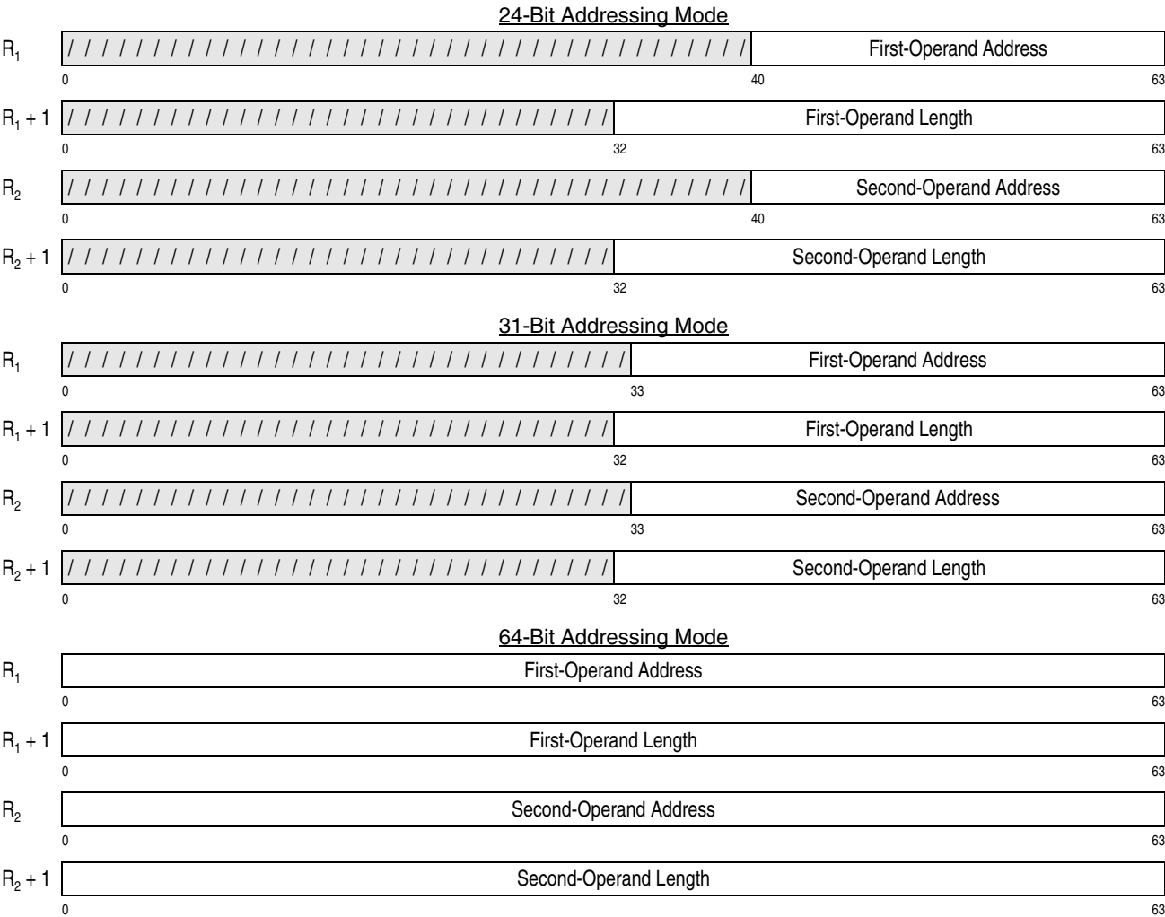
Figure 7-247. Register Contents for CONVERT UTF-32 TO UTF-16
