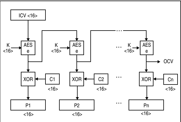
Figure 7-163. KMO-AES-128 Decipher Operation
