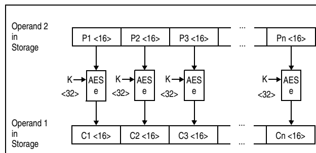
Figure 7-37. KM AES Decipher Operation Using 256-Bit Key
