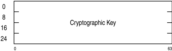
Figure 7-34. Parameter Block for KM-AES-256
