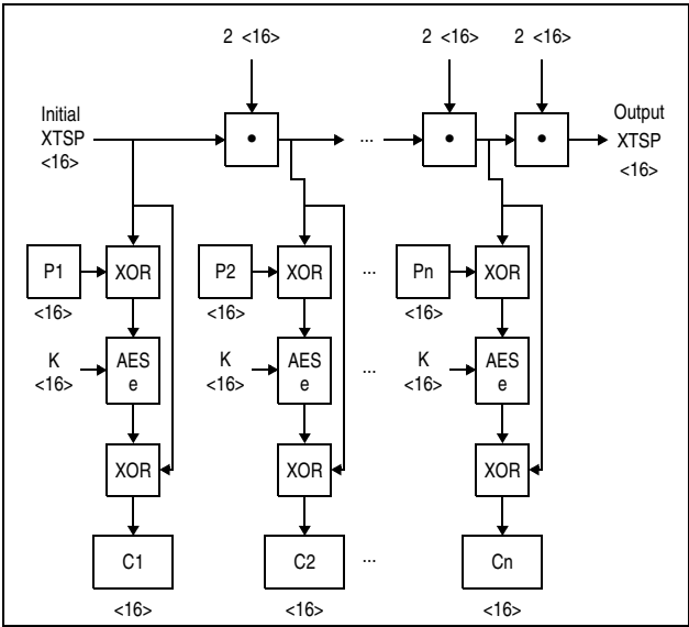
Figure 7-40. KM-XTS-AES-128 Encipher Operation
