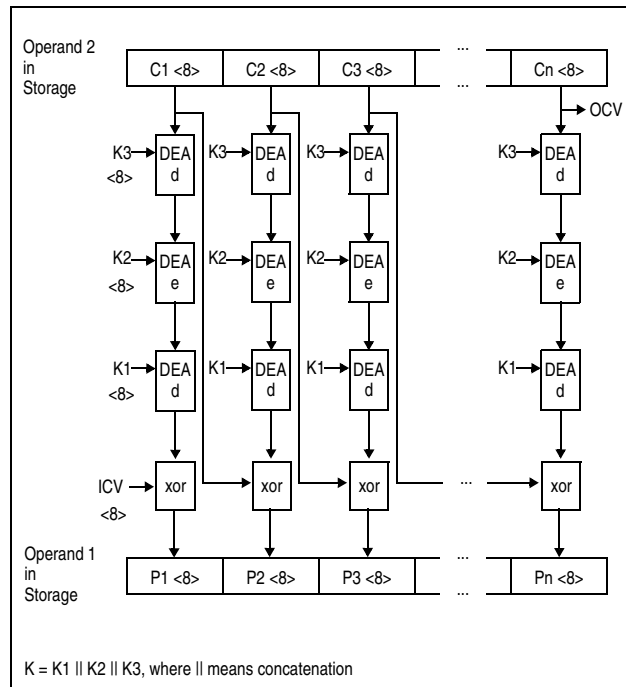
Figure 7-58. KMC TDEA Decipher Operation Using 192-Bit Key
