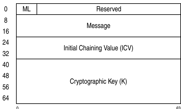
Figure 7-280. Parameter Block for PCC-Compute-Last-Block-CMAC-Using-AES-256
