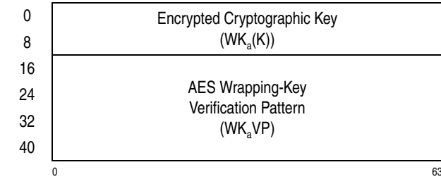
Figure 7-128. Parameter Block for KMCTR-Encrypted-AES-128
