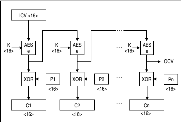
Figure 7-162. KMO-AES-128 Encipher Operation
