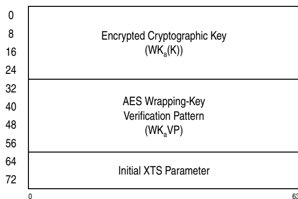
Figure 7-43. Parameter Block for KM-XTS-Encrypted-AES-256
