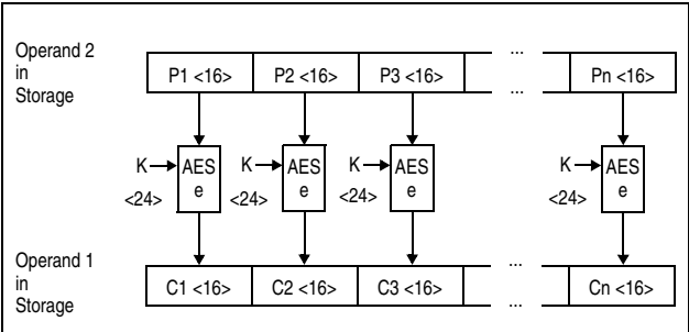
Figure 7-32. KM AES Encipher Operation Using 192-Bit Key
