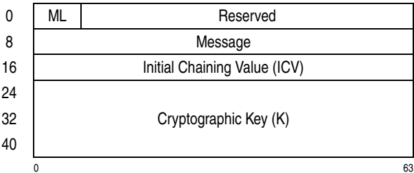
Figure 7-271. Parameter Block for PCC-Compute-Last-Block-CMAC-Using-TDEA-192
