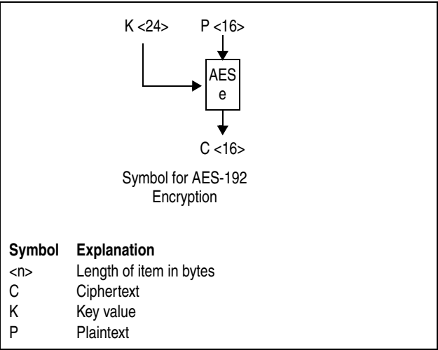
Figure 7-145. Symbols for AES-192 Encryption
