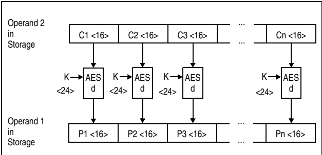
Figure 7-33. KM AES Decipher Operation Using 192-Bit Key
