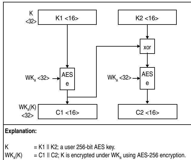
Figure 7-313. Encryption of 256-Bit AES Key Using WK_a
