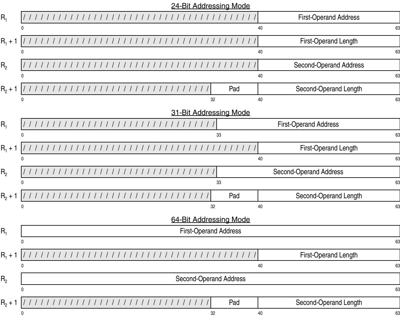
Figure 7-178. Register Contents for COMPARE LOGICAL LONG
