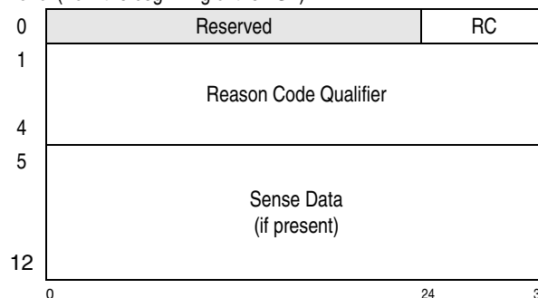
Figure 15-20. Device-Detected-Program-Check Transport-Status Area (TSA)
