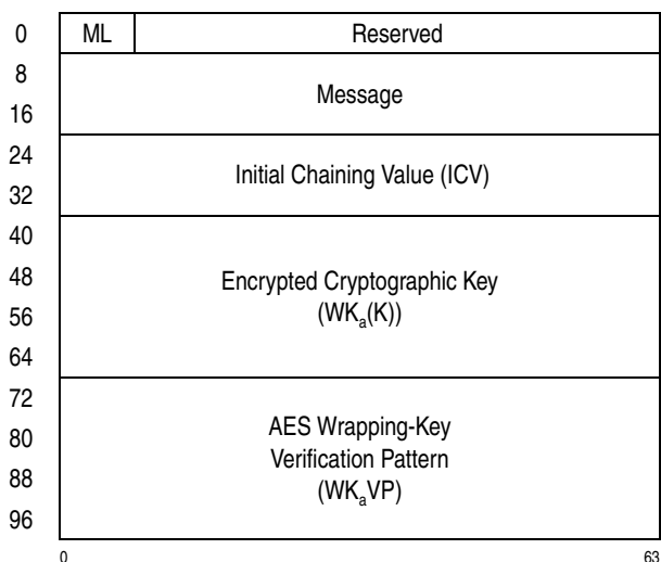
Figure 7-281. Parameter Block for PCC-Compute-Last-Block-CMAC-Using-Encrypted-AES-256
