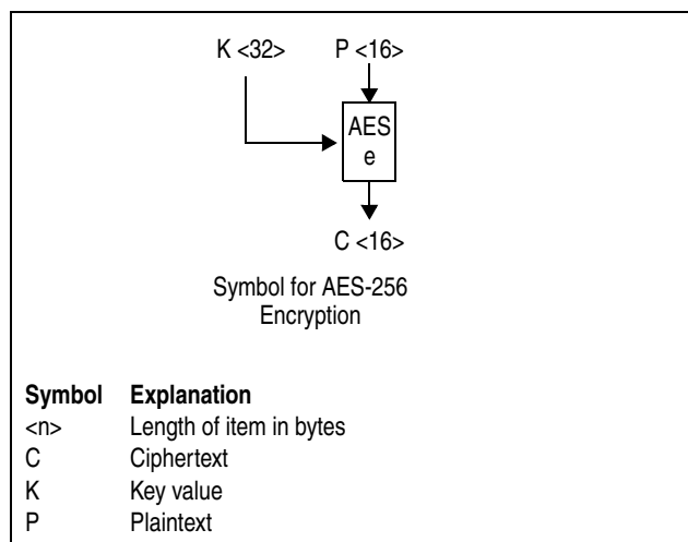
Figure 7-113. Symbols for AES-256 Encryption
