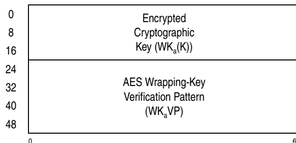
Figure 7-31. Parameter Block for KM-Encrypted-AES-192
