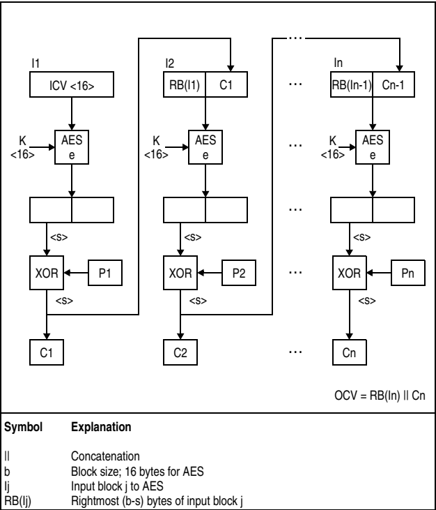
Figure 7-96. KMF-AES-128 Encipher Operation
