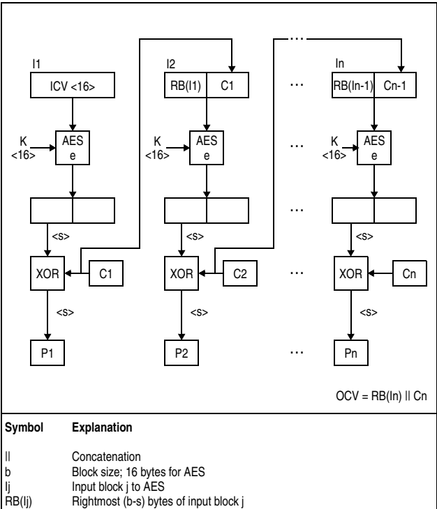
Figure 7-97. KMF-AES-128 Decipher Operation
