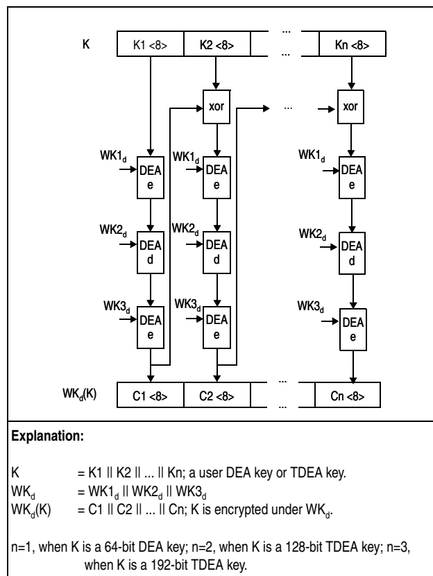
Figure 7-307. Encryption of DEA or TDEA Key Using WK_d
