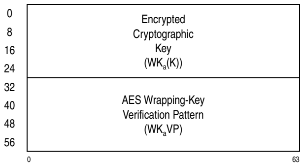
Figure 7-136. Parameter Block for KMCTR-Encrypted-AES-256
