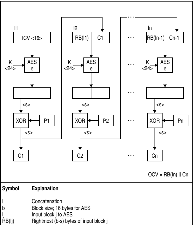
Figure 7-100. KMF-AES-192 Encipher Operation
