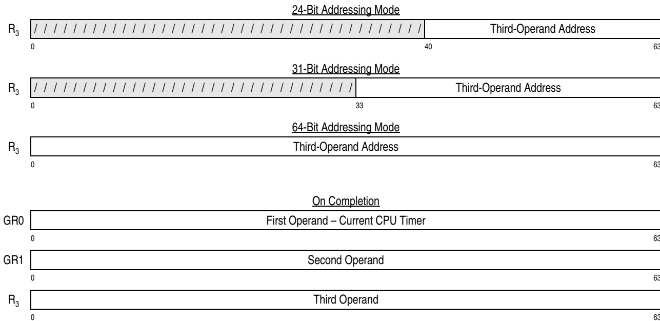
Figure 7-251. General Register Assignment for EXTRACT CPU TIME
