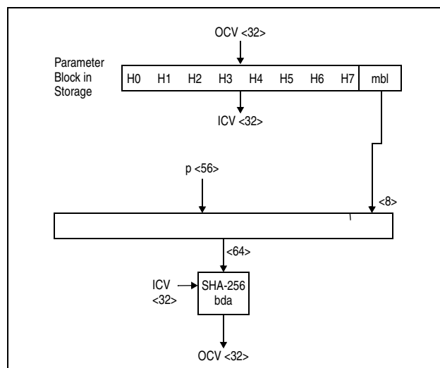
Figure 7-209. KLMD-SHA-256 Empty Block ( L = 0 )
