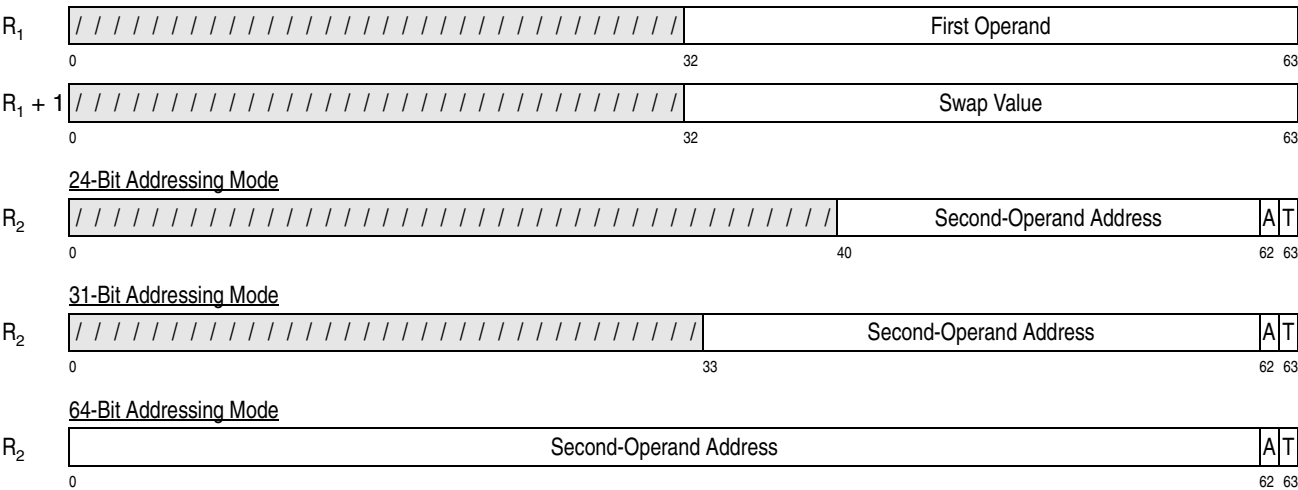
Figure 10-5. Register Contents for COMPARE AND SWAP AND PURGE (CSP)
