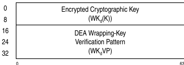
Figure 7-120. Parameter Block for KMCTR Encrypted-TDEA-128
