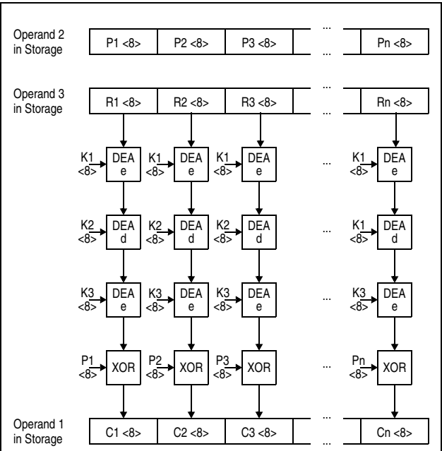
Figure 7-125. KMCTR TDEA Encipher Operation Using 192-Bit Key
