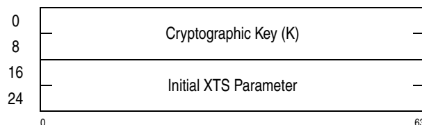
Figure 7-38. Parameter Block for KM-XTS-AES-128
