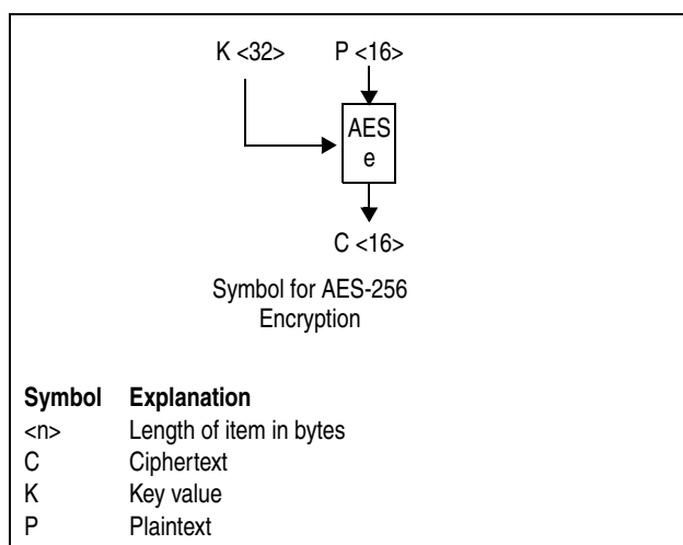
Figure 7-80. Symbols for AES-256 Encryption
