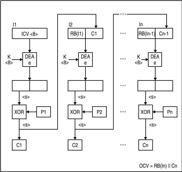
Figure 7-84. KMF-DEA Encipher Operation
