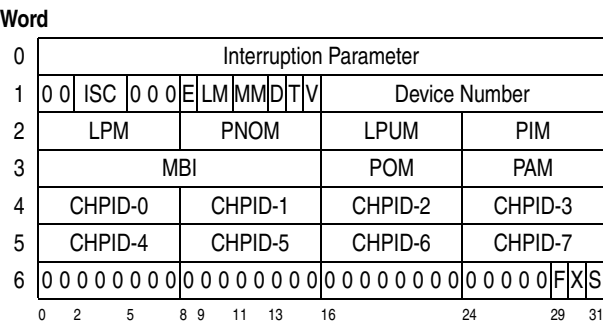
Figure 15-1. PMCW Format
