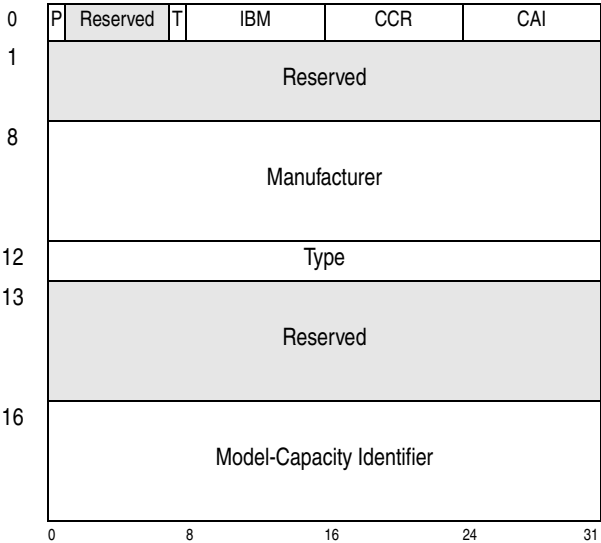
SYSIB 1.1.1
