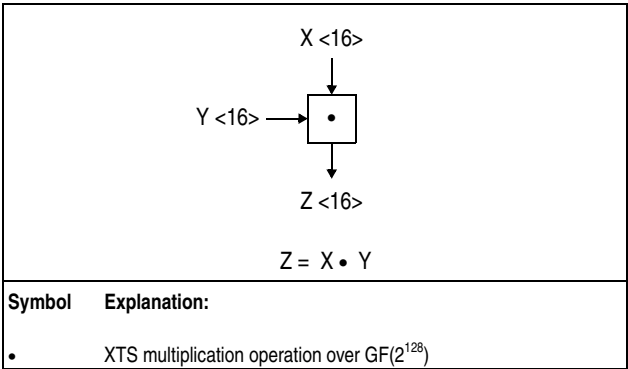
Figure 7-258. Symbol For XTS Multiplication Operation Over GF(2^{128})
