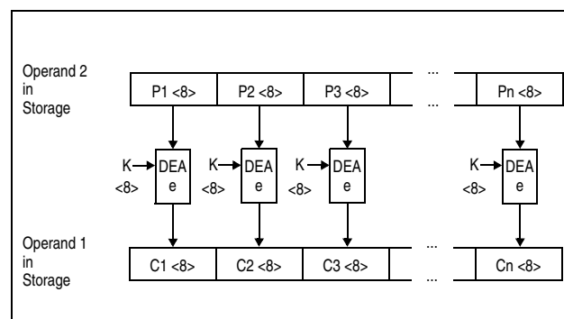
Figure 7-16. KM-DEA Encipher Operation Using 64-Bit Key
