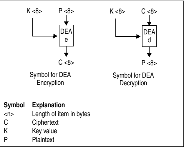
Figure 7-77. Symbols for DEA Encryption and Decryption
