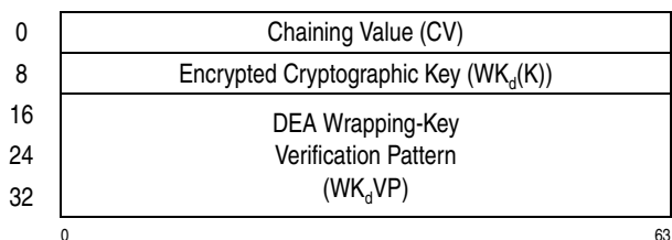
Figure 7-48. Parameter Block for KMC-Encrypted-DEA
