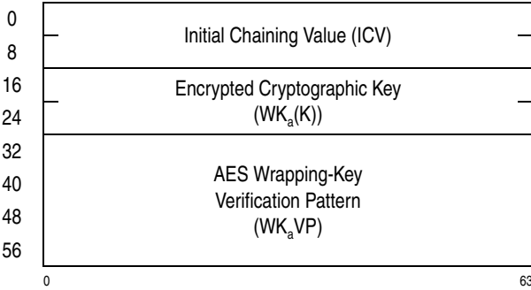
Figure 7-236. Parameter Block for KMAC-Encrypted-AES-128
