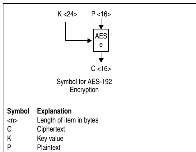
Figure 7-112. Symbols for AES-192 Encryption
