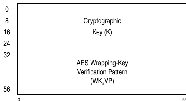
Figure 10-41. Parameter Block for PCKMO-Encrypt-AES-256-Key
