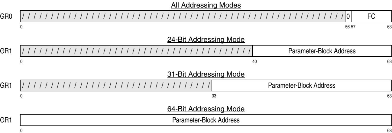
Figure 7-256. General Register Assignment for PCC
