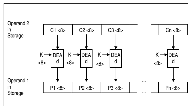
Figure 7-17. KM-DEA Decipher Operation Using 64-Bit Key
