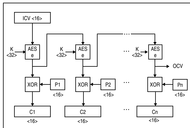
Figure 7-170. KMO-AES-256 Encipher Operation
