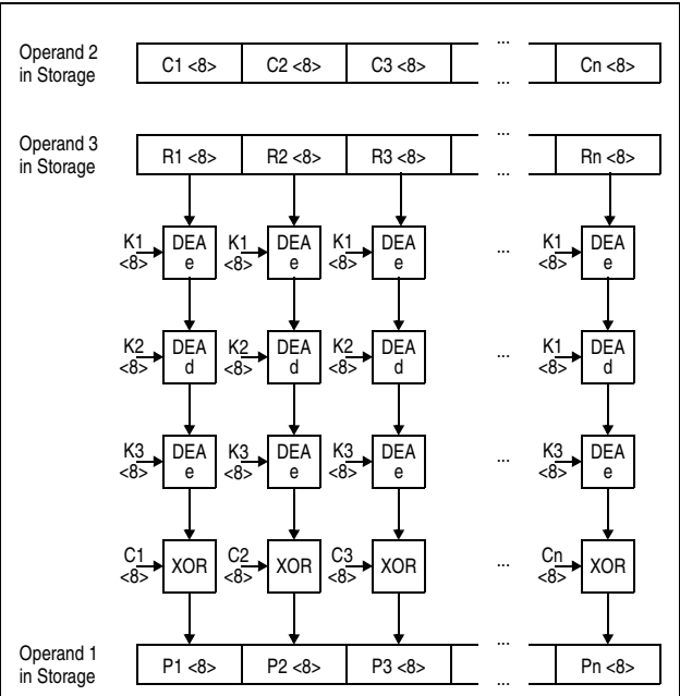
Figure 7-126. KMCTR TDEA Decipher Operation Using 192-Bit Key
