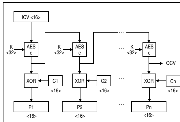
Figure 7-171. KMO-AES-256 Decipher Operation
