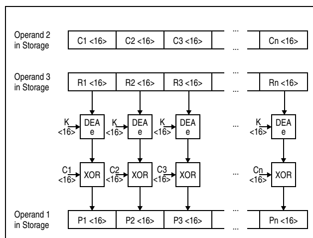
Figure 7-130. KMCTR AES Decipher Operation Using 128-Bit Key
