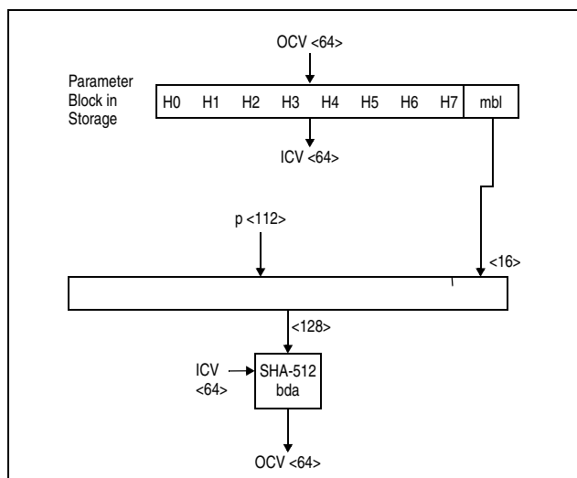
Figure 7-214. KLMD-SHA-512 Empty Block ( L = 0 )
