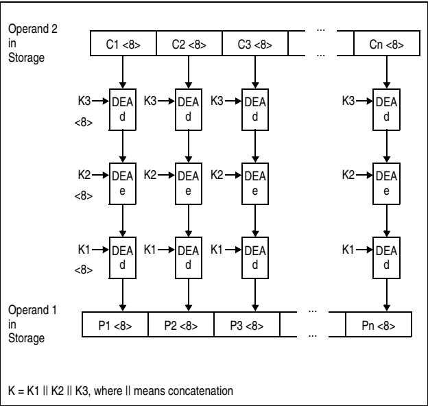
Figure 7-25. KM TDEA Decipher Operation Using 192-Bit Key
