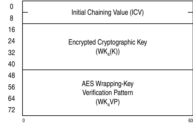
Figure 7-242. Parameter Block for KMAC-Encrypted-AES-256
