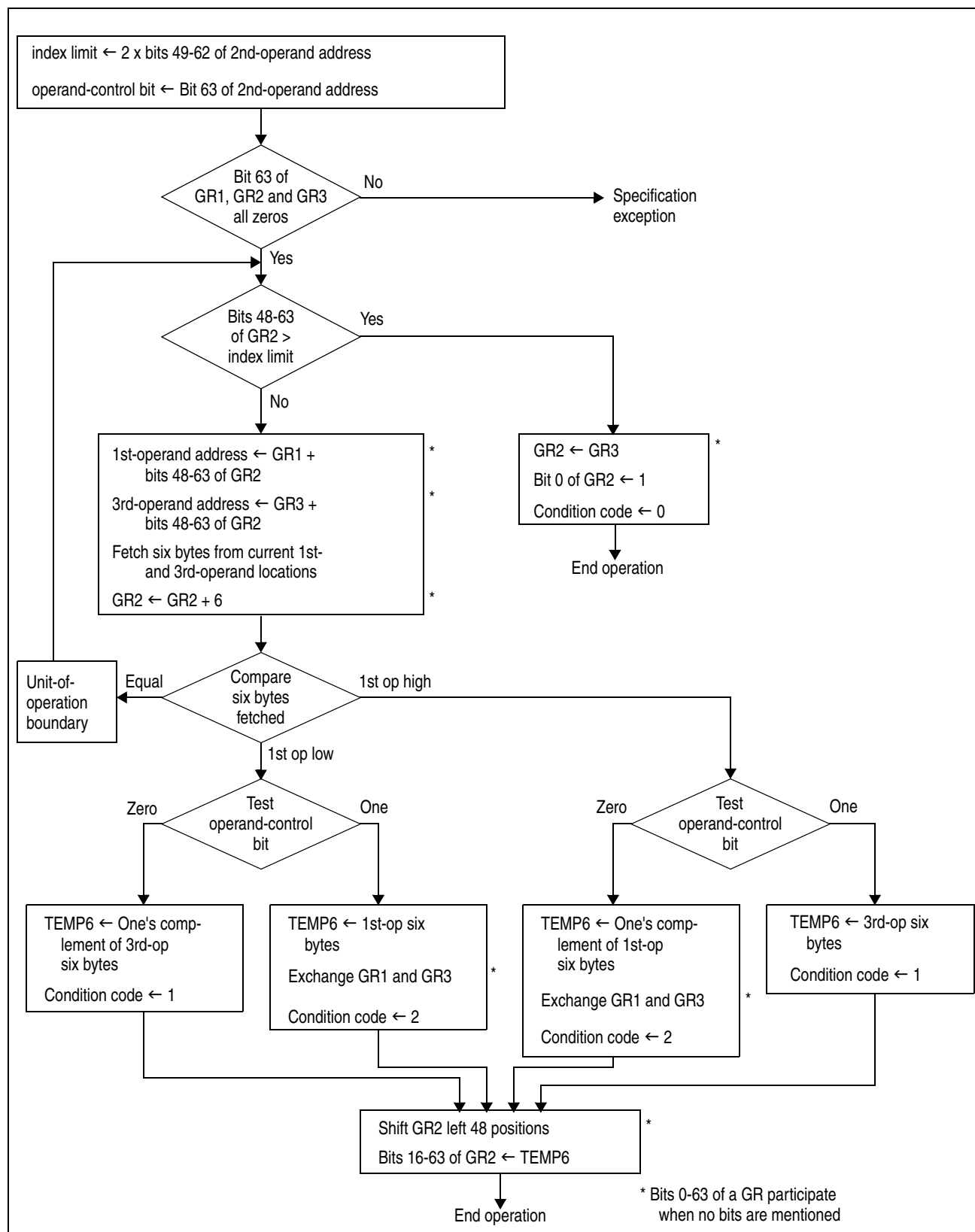
Figure 7-176. Execution of COMPARE AND FORM CODEWORD in the 64-bit Addressing Mode
