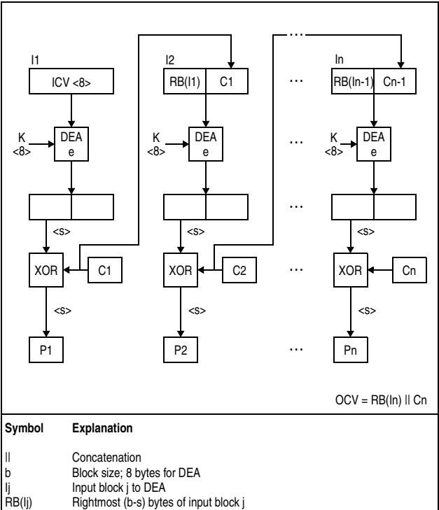
Figure 7-85. KMF-DEA Decipher Operation
