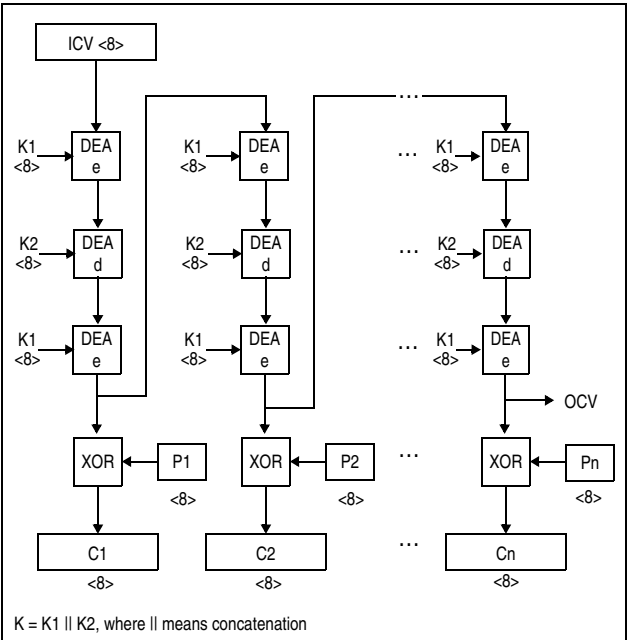
Figure 7-154. KMO-TDEA-128 Encipher Operation
