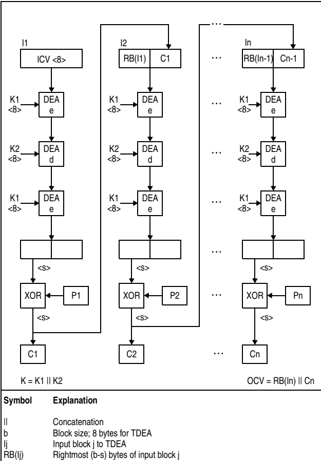
Figure 7-88. KMF-TDEA-128 Encipher Operation
