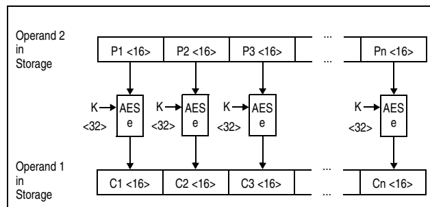
Figure 7-36. KM AES Encipher Operation Using 256-Bit Key
