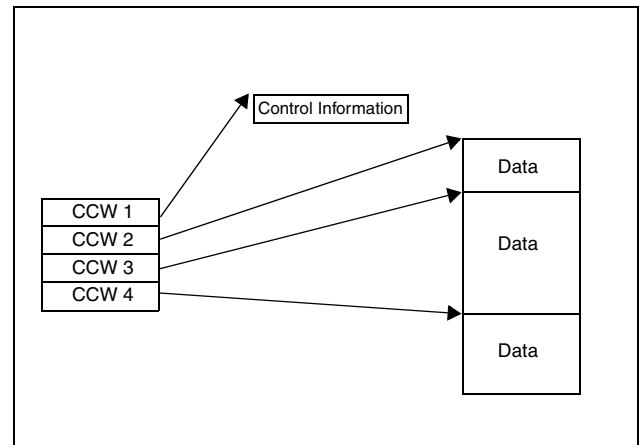
Figure 1. CCW Channel Program Example
