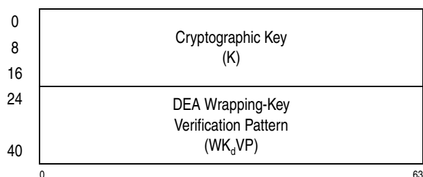
Figure 10-38. Parameter Block for PCKMO-Encrypt-TDEA-192-Key
