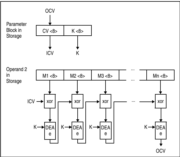
Figure 7-228. MAC Computation Using 64-bit DEA Key
