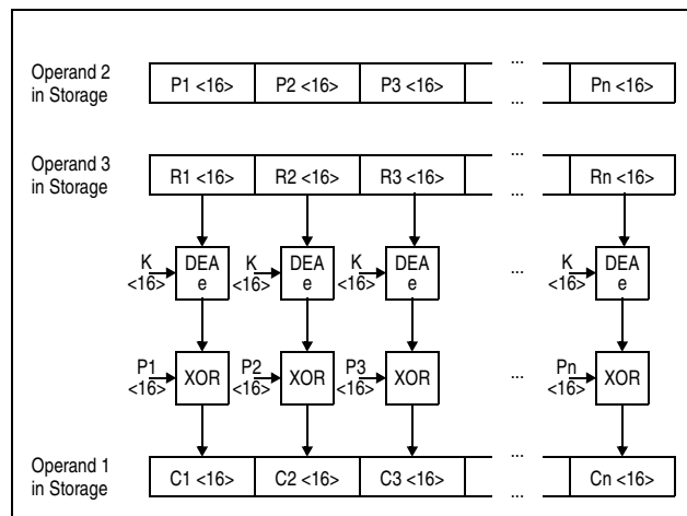
Figure 7-129. KMCTR AES Encipher Operation Using 128-Bit Key
