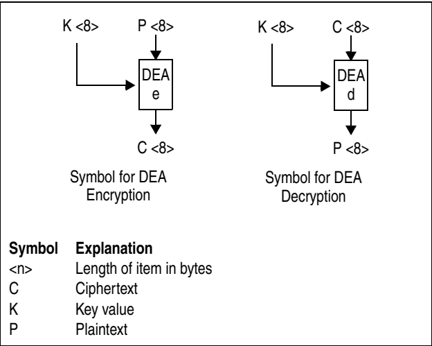
Figure 7-221. Symbols for DEA Encryption and Decryption
