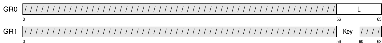
Figure 10-32. Register Contents of MOVE WITH SOURCE KEY
