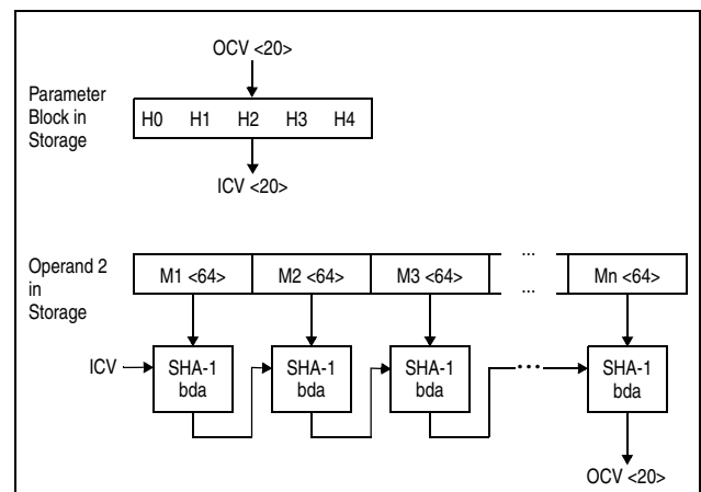
Figure 7-73. KIMD-SHA-1
