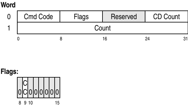
Figure 15-9. Device-Command Word (DCW)
