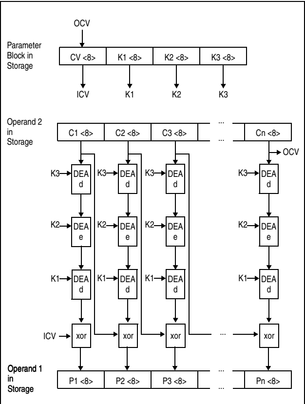
Figure 7-40. KMC-TDEA-192 Decipher Operation
