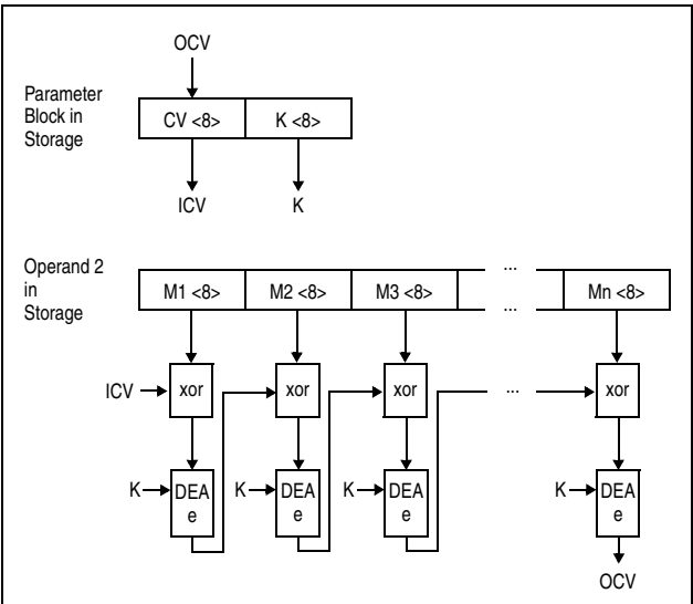
Figure 7-101. KMAC-DEA
