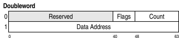
Figure 15-4. Modified-Indirect-Data-Address Word (MIDAW)
