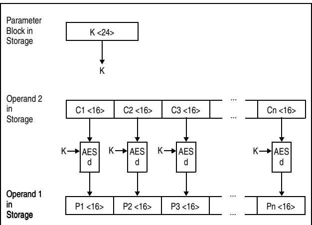
Figure 7-27. KM-AES-192 Decipher Operation
