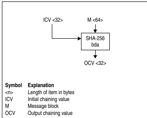
Figure 7-69. Symbol for SHA-256 Block Digest Algorithm
