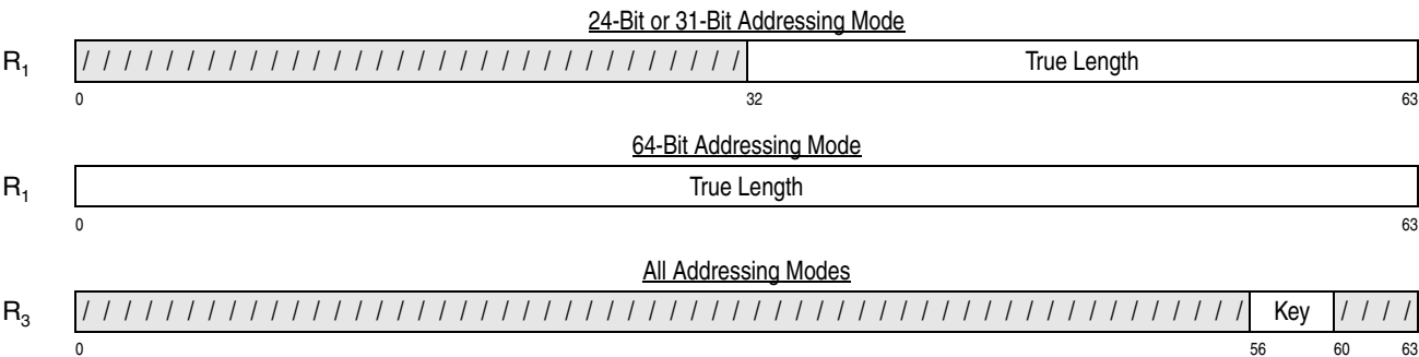
Figure 10-25. Register Contents of MOVE TO PRIMARY and MOVE TO SECONDARY
