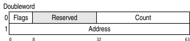
Figure 15-5. Transport-Indirect-Data-Address Word (TIDAW)
