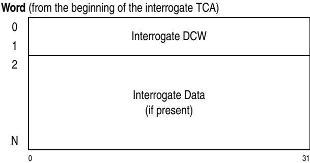
Figure 15-12. Interrogate Transport-Command Area (TCA)
