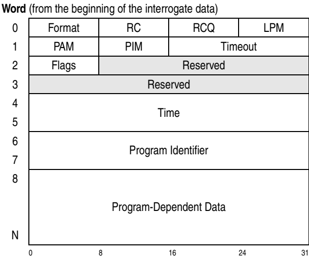
Figure 15-13. Interrogate Data
