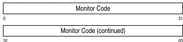
Real Locations 176-183
