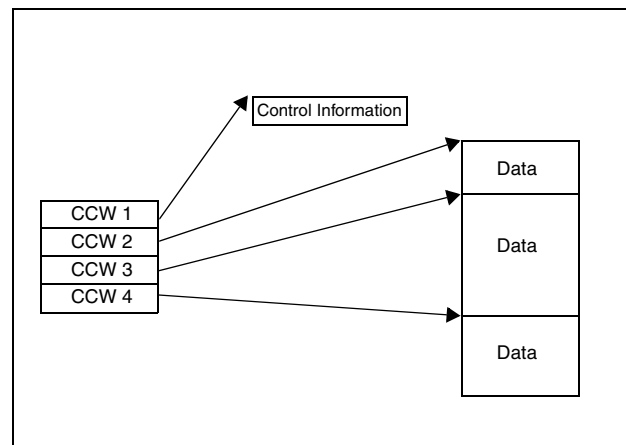
Figure 1. CCW Channel Program Example
