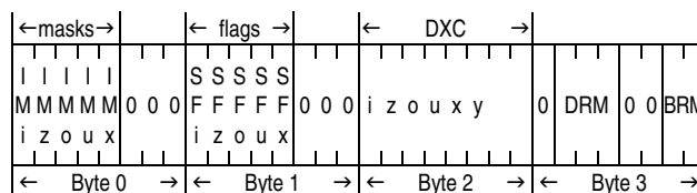
Figure 9-5. FPC Register Overview
