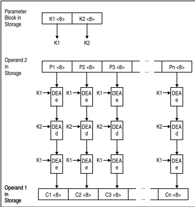
Figure 7-17. KM-TDEA-128 Encipher Operation
