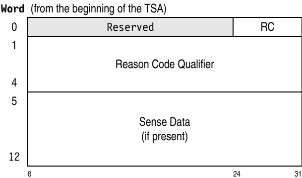
Figure 15-17. Device-Detected-Program-Check Transport-Status Area (TSA)
