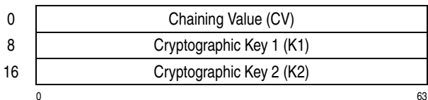
Figure 7-102. Parameter Block for KMAC-TDEA-128
