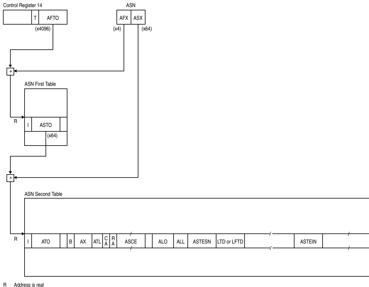
Figure 3-8. ASN Translation
