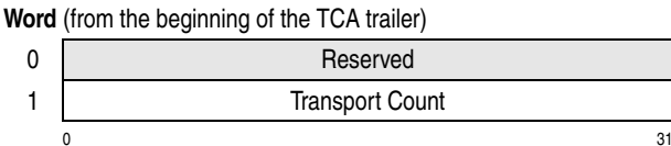
Figure 15-10. Transport-Command-Area Trailer (TCAT) - Uni-Directional
