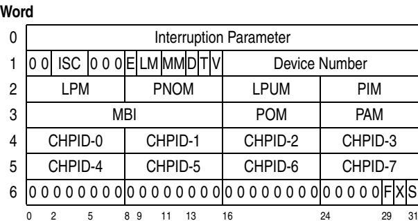
Figure 15-1. PMCW Format
