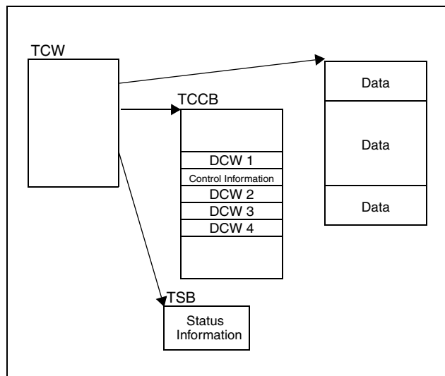
Figure 2. Uni-Directional TCW Channel Program Example
