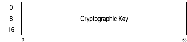
Figure 7-25. Parameter Block for KM-AES-192
