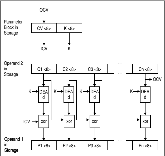
Figure 7-34. KMC-DEA Decipher Operation
