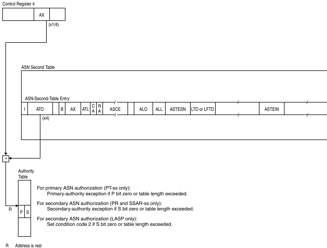
Figure 3-9. ASN Authorization
