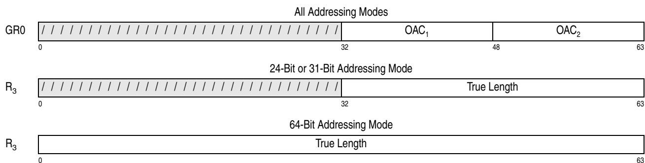
Figure 10-30. Register Contents for MOVE WITH OPTIONAL SPECIFICATIONS
