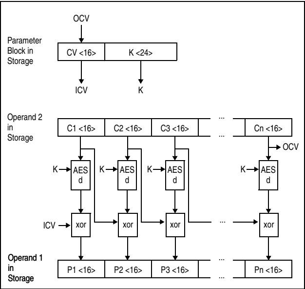
Figure 7-46. KMC-AES-192 Decipher Operation
