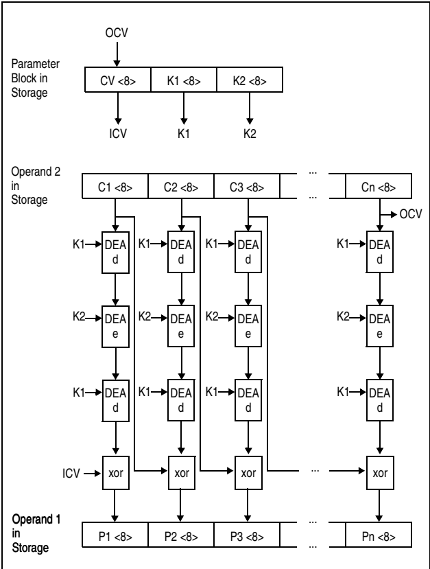
Figure 7-37. KMC-TDEA-128 Decipher Operation
