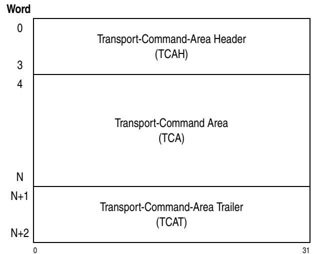
Figure 15-6. Transport-Command-Control Block (TCCB)
