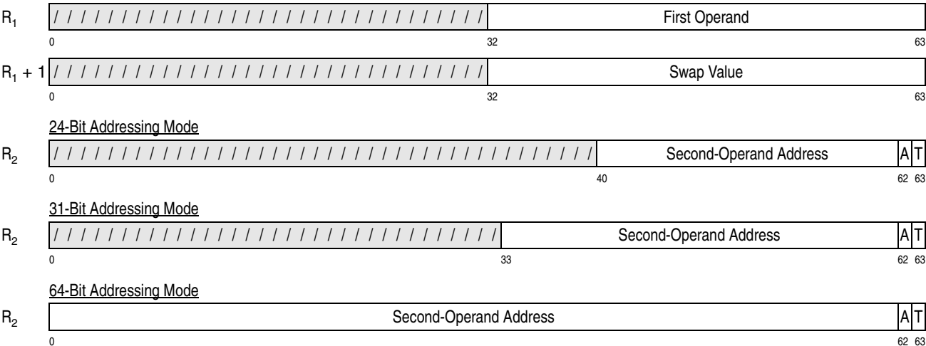
Figure 10-5. Register Contents for COMPARE AND SWAP AND PURGE (CSP)
