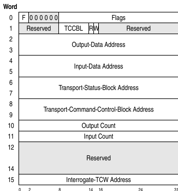
Figure 15-5. Transport-Control Word (TCW)
