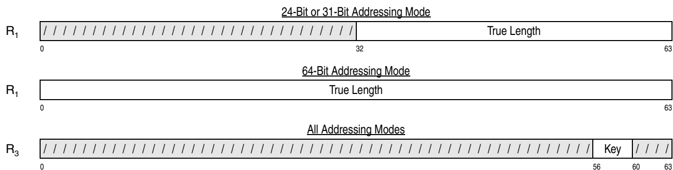
Figure 10-28. Register Contents of MOVE WITH KEY
