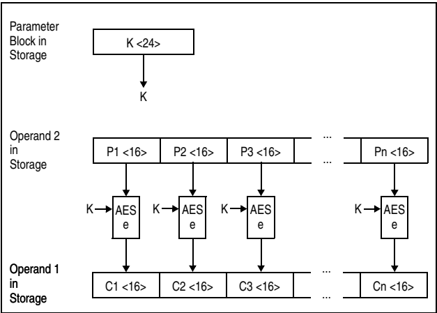
Figure 7-26. KM-AES-192 Encipher Operation
