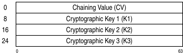
Figure 7-104. Parameter Block for KMAC-TDEA-192
