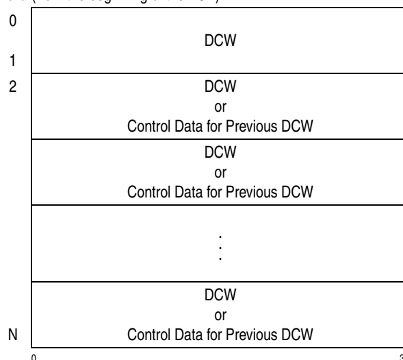
Figure 15-8. Transport-Command Area (TCA)
