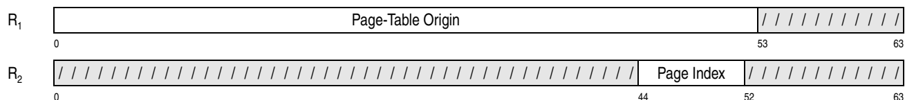
Figure 10-15. Register Contents for INVALIDATE PAGE TABLE ENTRY
