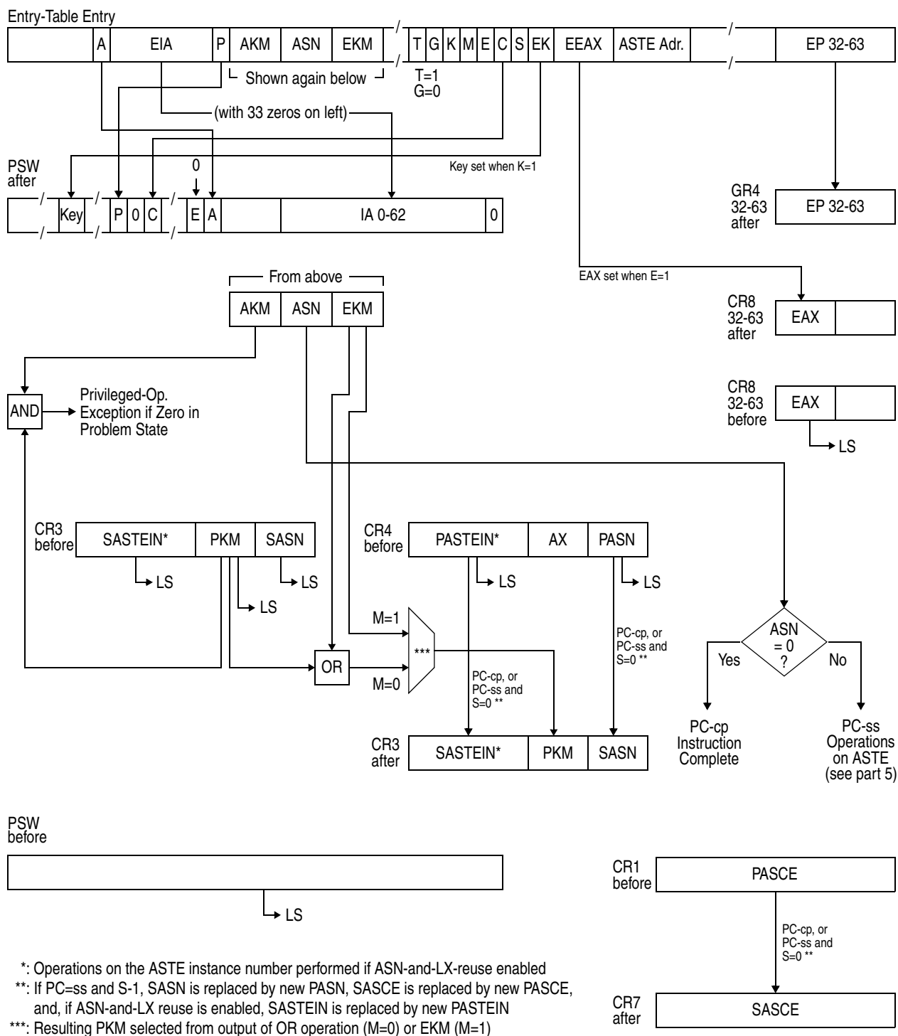
Figure 10-49. Execution of PROGRAM CALL (Part 4 of 5).
