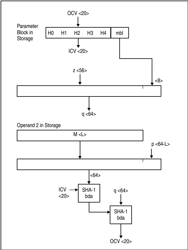
Figure 7-83. KLMD-SHA-1 Partial-Block Case 2 ( 56 \leq L \leq 63 )
