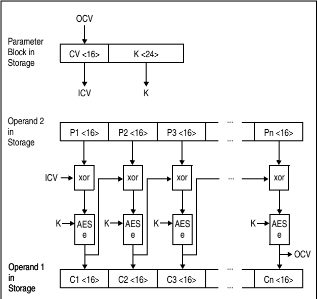
Figure 7-45. KMC-AES-192 Encipher Operation
