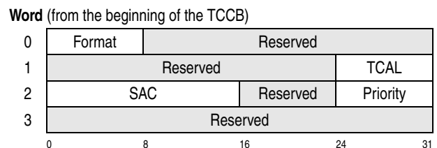
Figure 15-7. Transport-Command-Area Header (TCAH)
