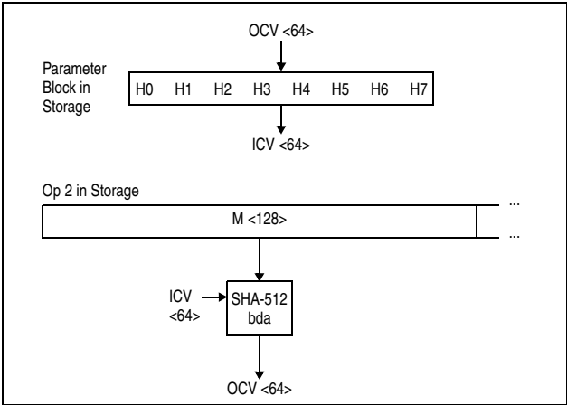
Figure 7-90. KLMD-SHA-512 Full Block ( L \geq 128 )
