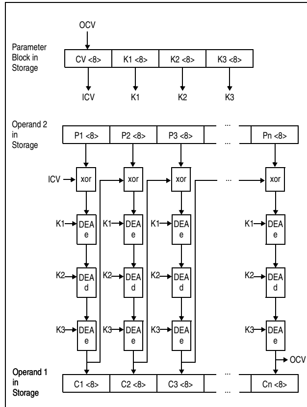
Figure 7-39. KMC-TDEA-192 Encipher Operation
