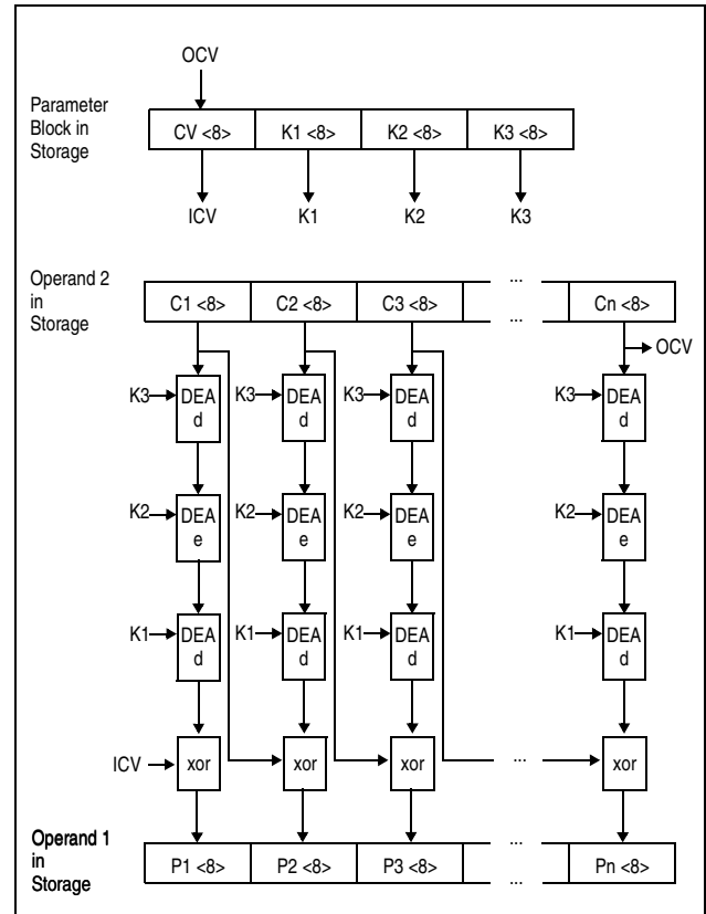
Figure 7-40. KMC-TDEA-192 Decipher Operation
