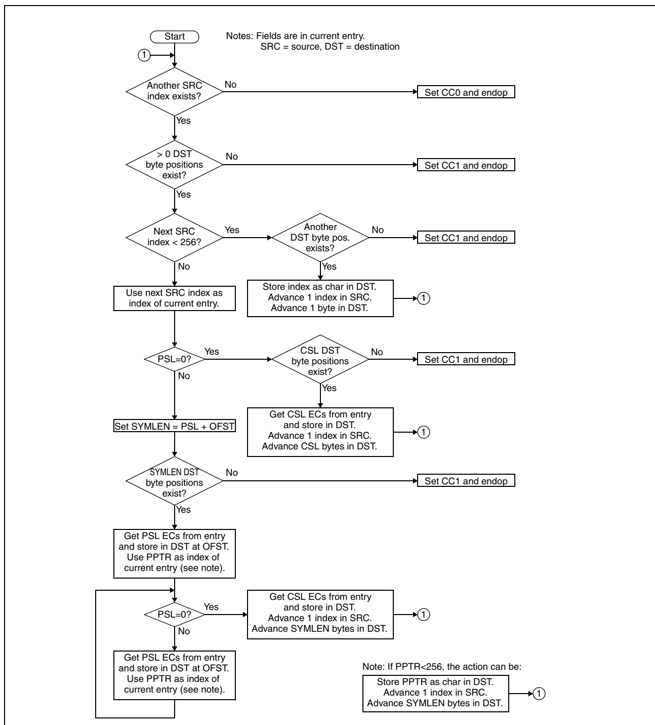
Figure 7-64. Expansion Process
