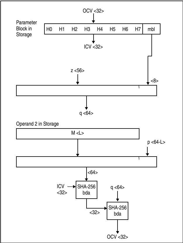
Figure 7-88. KLMD-SHA-256 Partial-Block Case 2 ( 56 \leq L \leq 63 )
