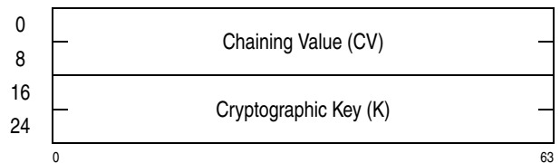
Figure 7-41. Parameter Block for KMC-AES-128
