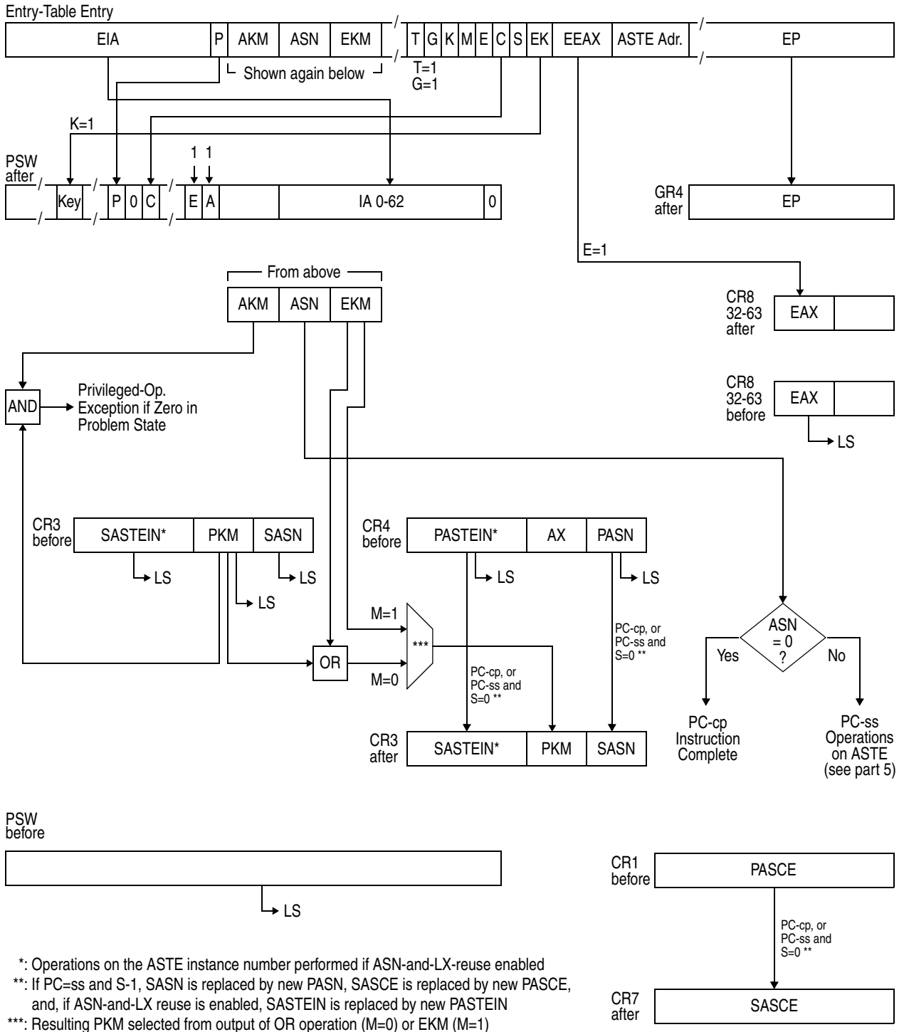
Figure 10-49. Execution of PROGRAM CALL (Part 3 of 5).
