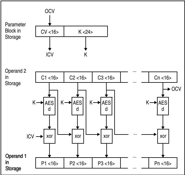
Figure 7-46. KMC-AES-192 Decipher Operation
