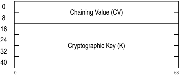
Figure 7-47. Parameter Block for KMC-AES-256
